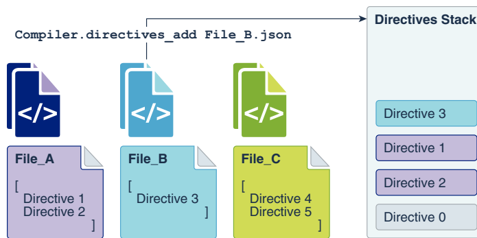
Figure 2-3 Adding a Directive to a Running Program
