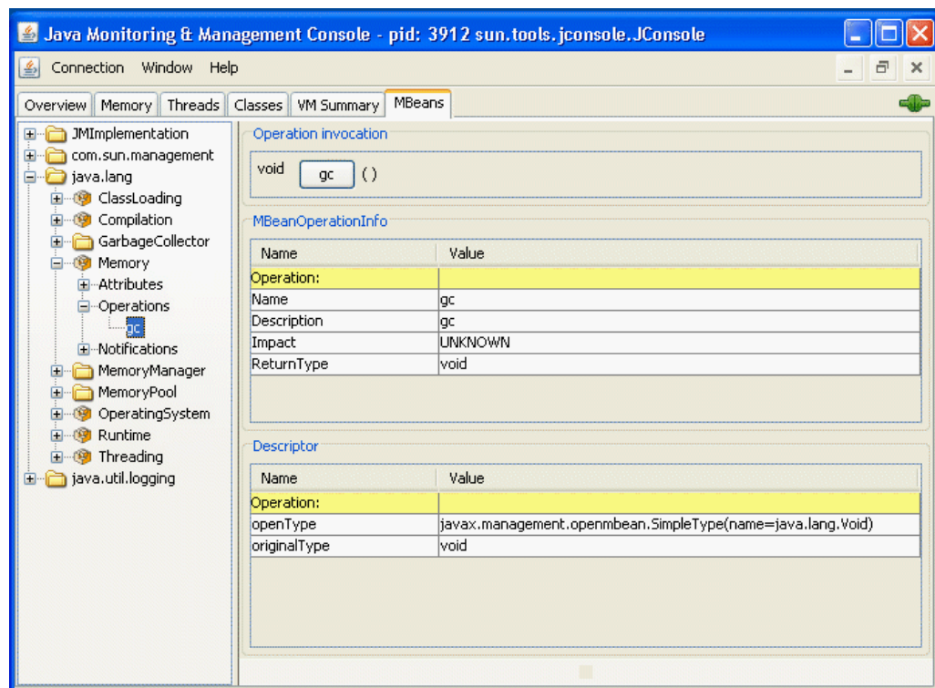
Figure 3-21 Viewing Individual MBean Operations
