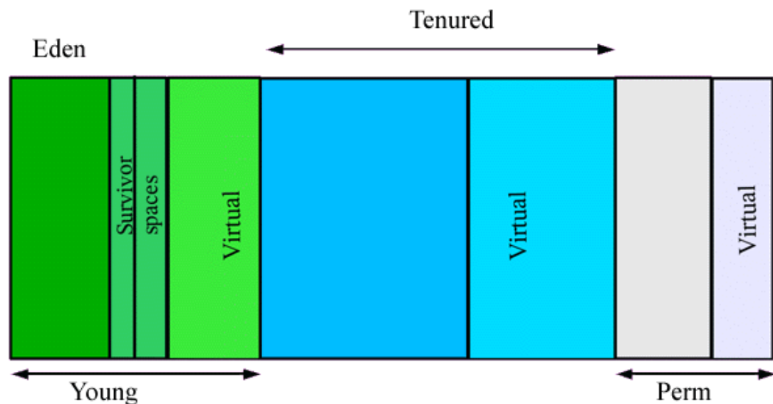
Figure 3-7 Generations of Data in Garbage Collection
