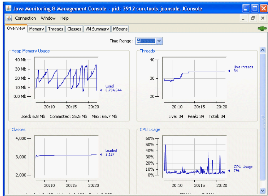
Figure 3-5 Overview Tab
