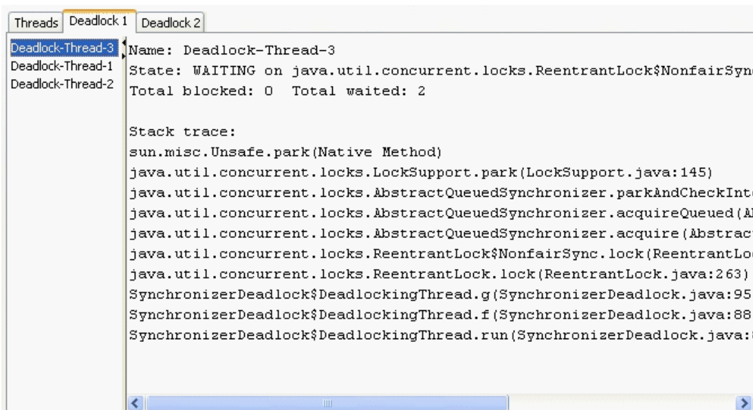
Figure 3-9 Deadlocked Threads
