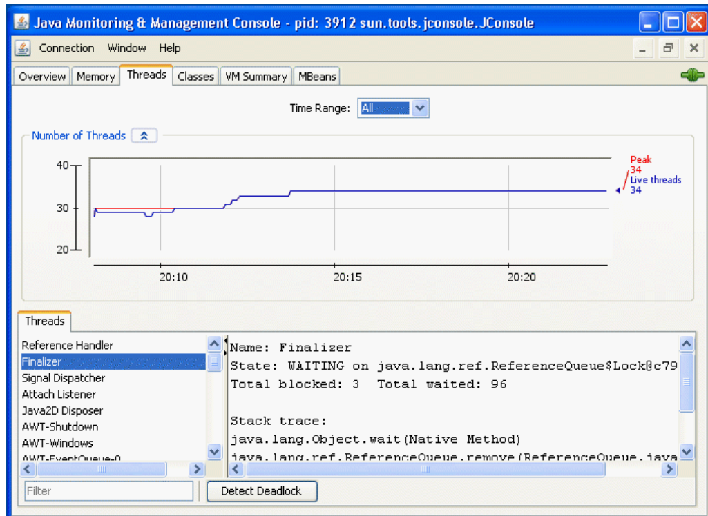
Figure 3-8 Threads Tab
