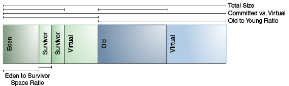
Figure 4-1 Heap Options
