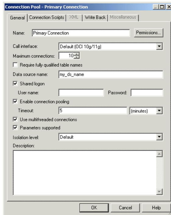
Figure 5–8 Connection Pool Dialog for Primary Connection Pool
