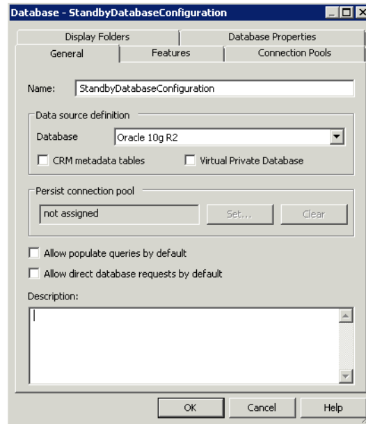
Figure 5–6 Database Dialog for Standby Database Configuration
