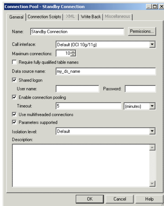
Figure 5–7 Connection Pool Dialog for Standby Connection Pool
