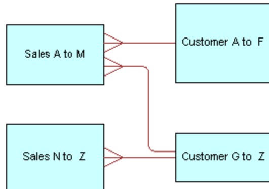
Figure 8-8 Joins for Fragmented Tables Example
