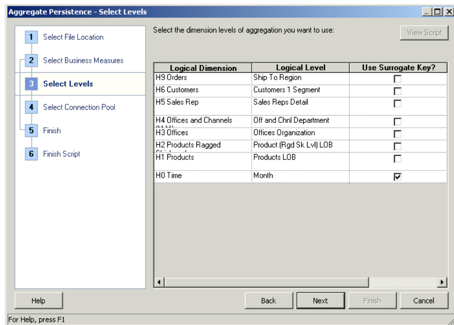
Figure 13–3 Aggregate Persistence Wizard: Select Levels Screen
