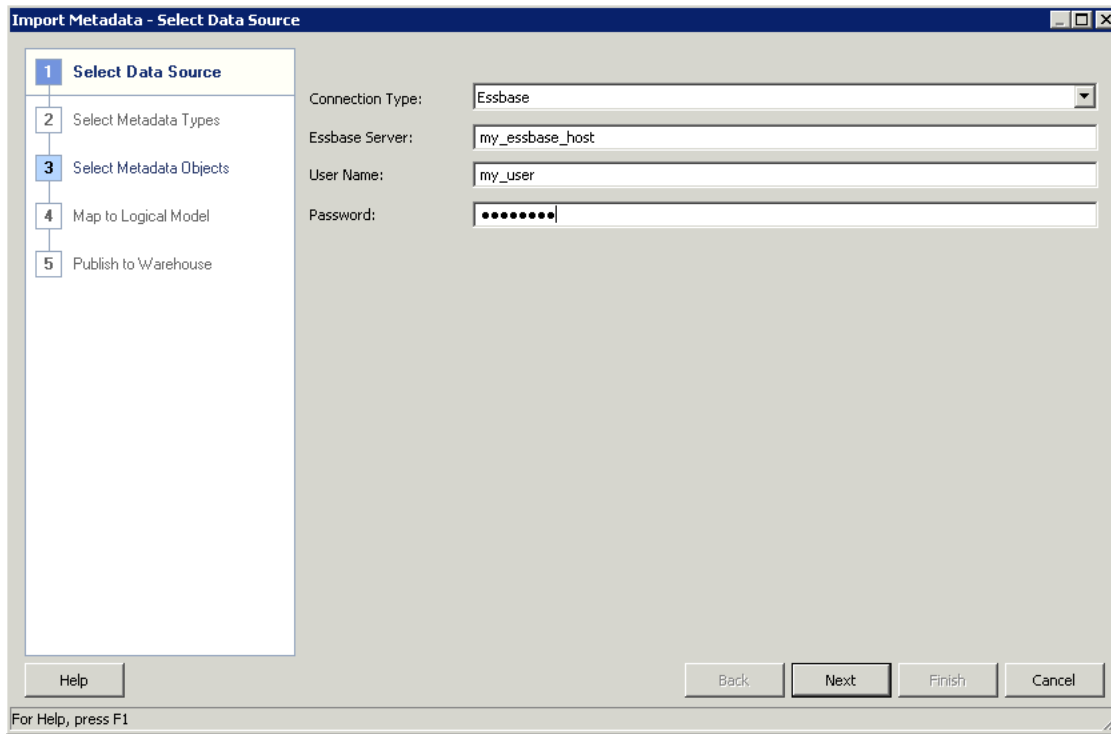
Figure 5–3 Import Metadata Wizard: Multidimensional Data Source
