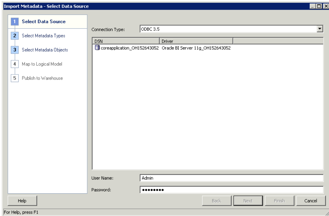
Figure 5–2 Import Metadata Wizard: Relational Data Source
