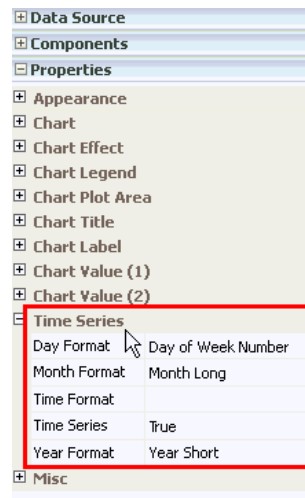
Figure 3–67 Time Series Date Formatting Options
