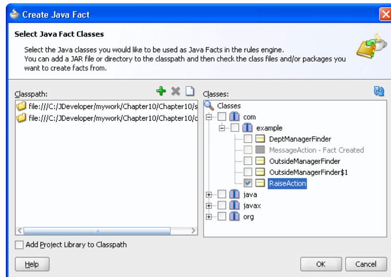
Figure 10–18 Create Java Fact from Raise Action Class
