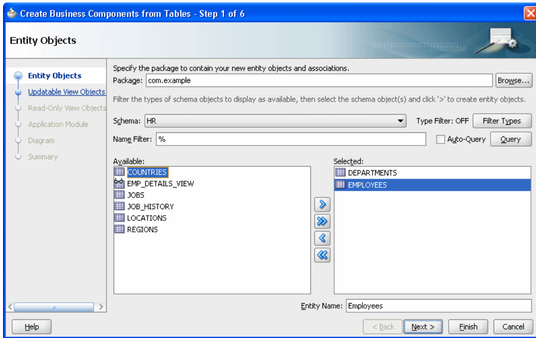
Figure 10–2 Selecting Entity Objects for Sample Application
