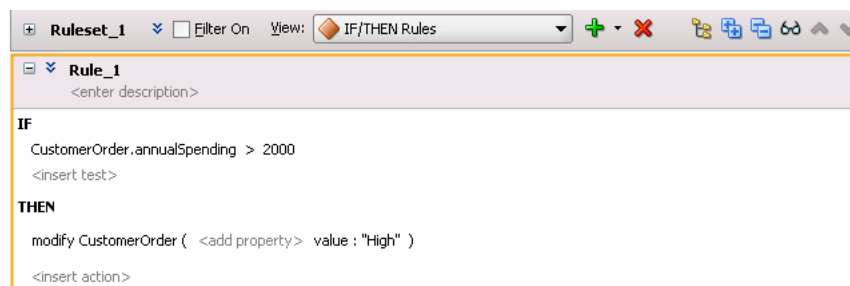
Figure 4–30 Rule with Test and Action Added
