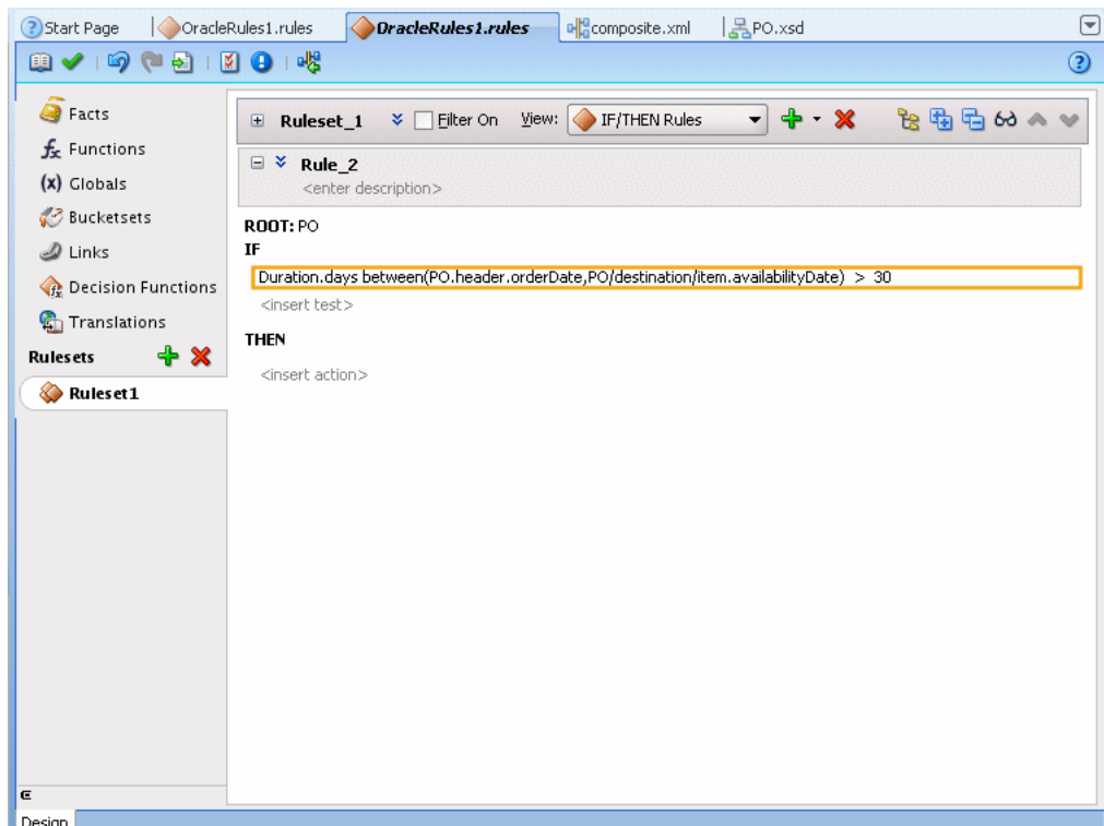
Figure 4–63 Simple Tree Mode: Right-Hand Operand with Value 30
