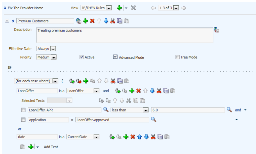
Figure 12–41 Showing Advanced Mode Rule Options
