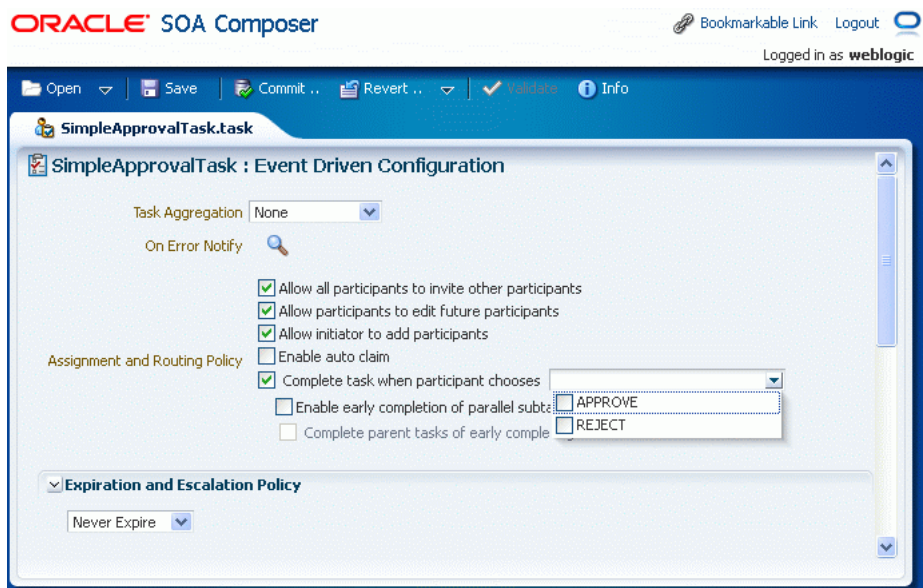
Figure 12–108 Setting Assignment and Routing Policy
