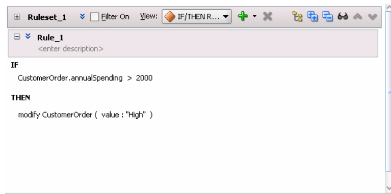
Figure 4–10 Adding a Test to a Rule
