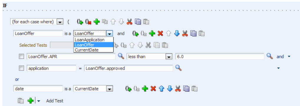
Figure 12–42 Specifying Pattern Variable and Fact Type
