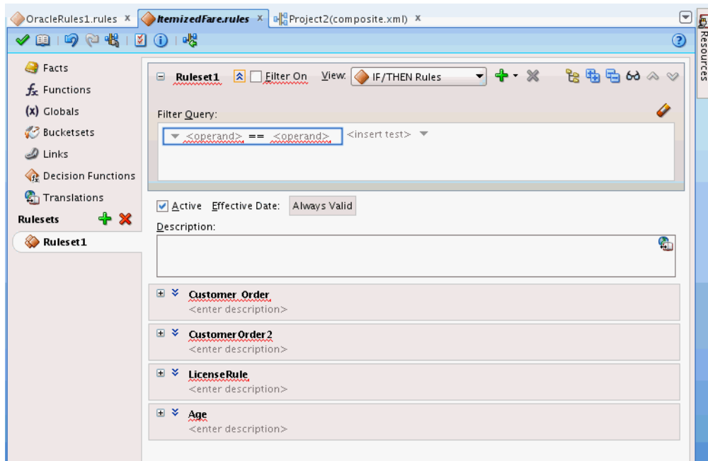
Figure 4–5 Inserting a Default Filter Query Test
