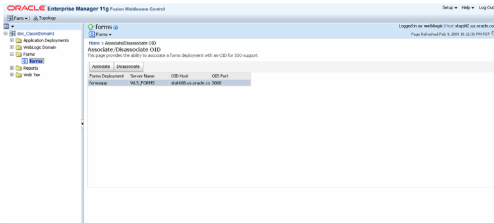
Figure 9–4 Associate/Disassociate OID
