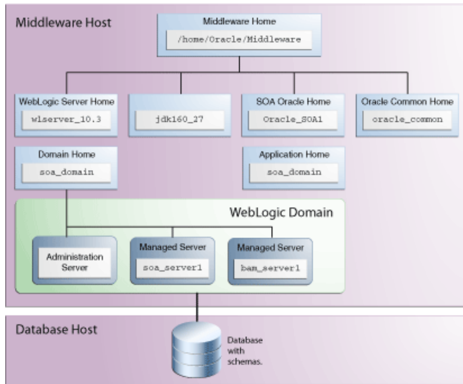
Figure 2 Completed Installation and Configuration Topology
