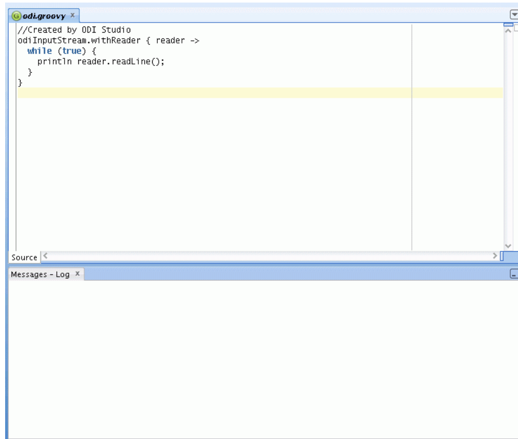
Figure C-1 Groovy Editor
