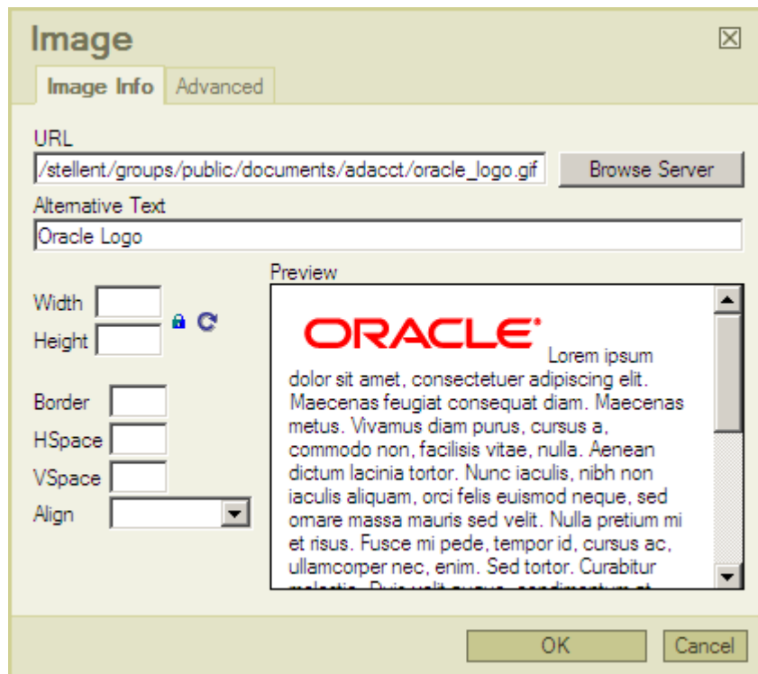
Figure 5–5 Image Dialog
