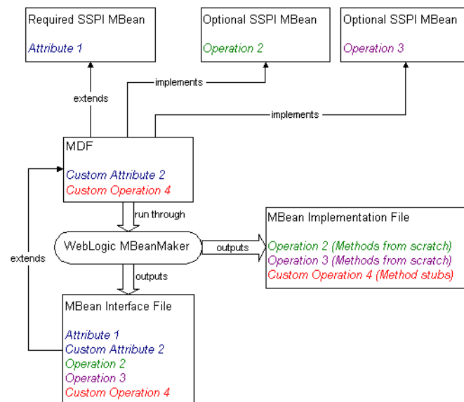
Figure 3–7 What the WebLogic MBeanMaker Provides
