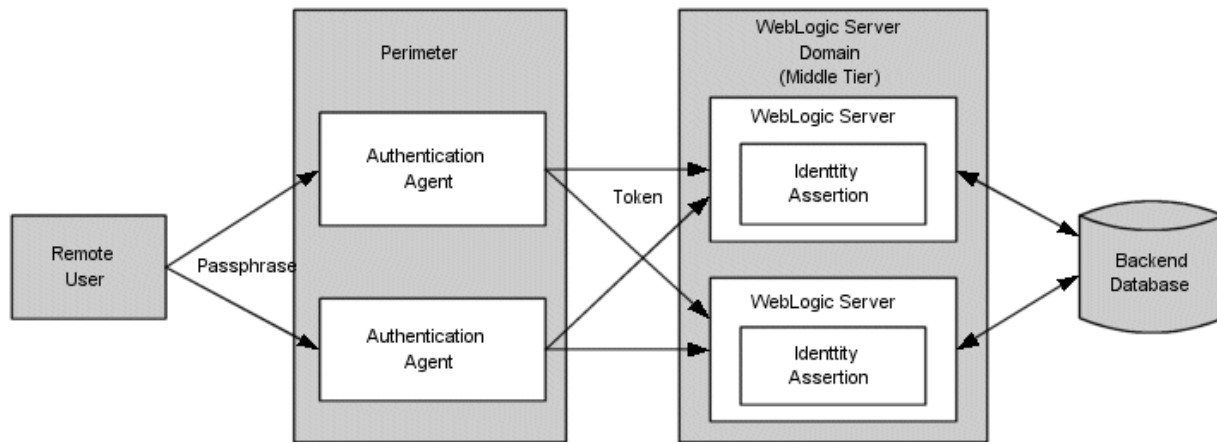
Figure 3–2 Perimeter Authentication
