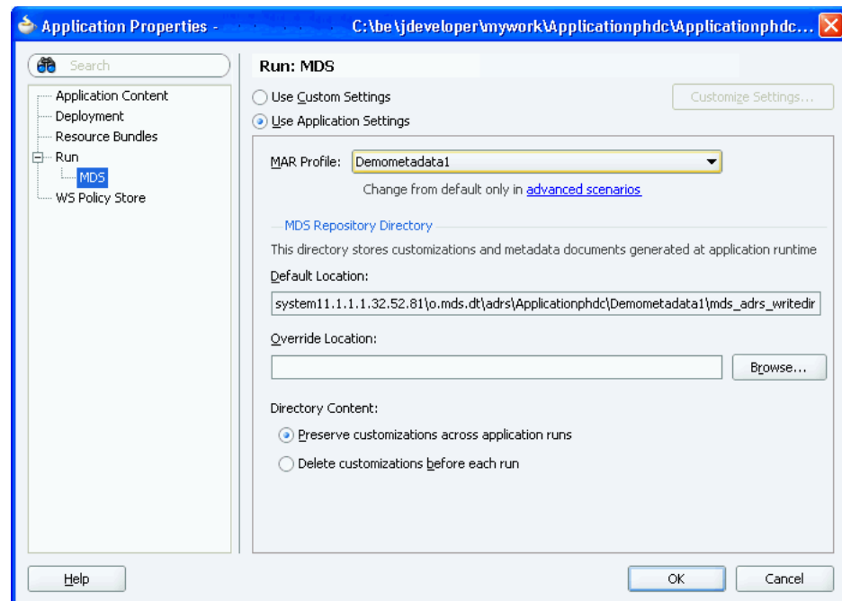
Figure 8–1 Setting the Run MDS options
