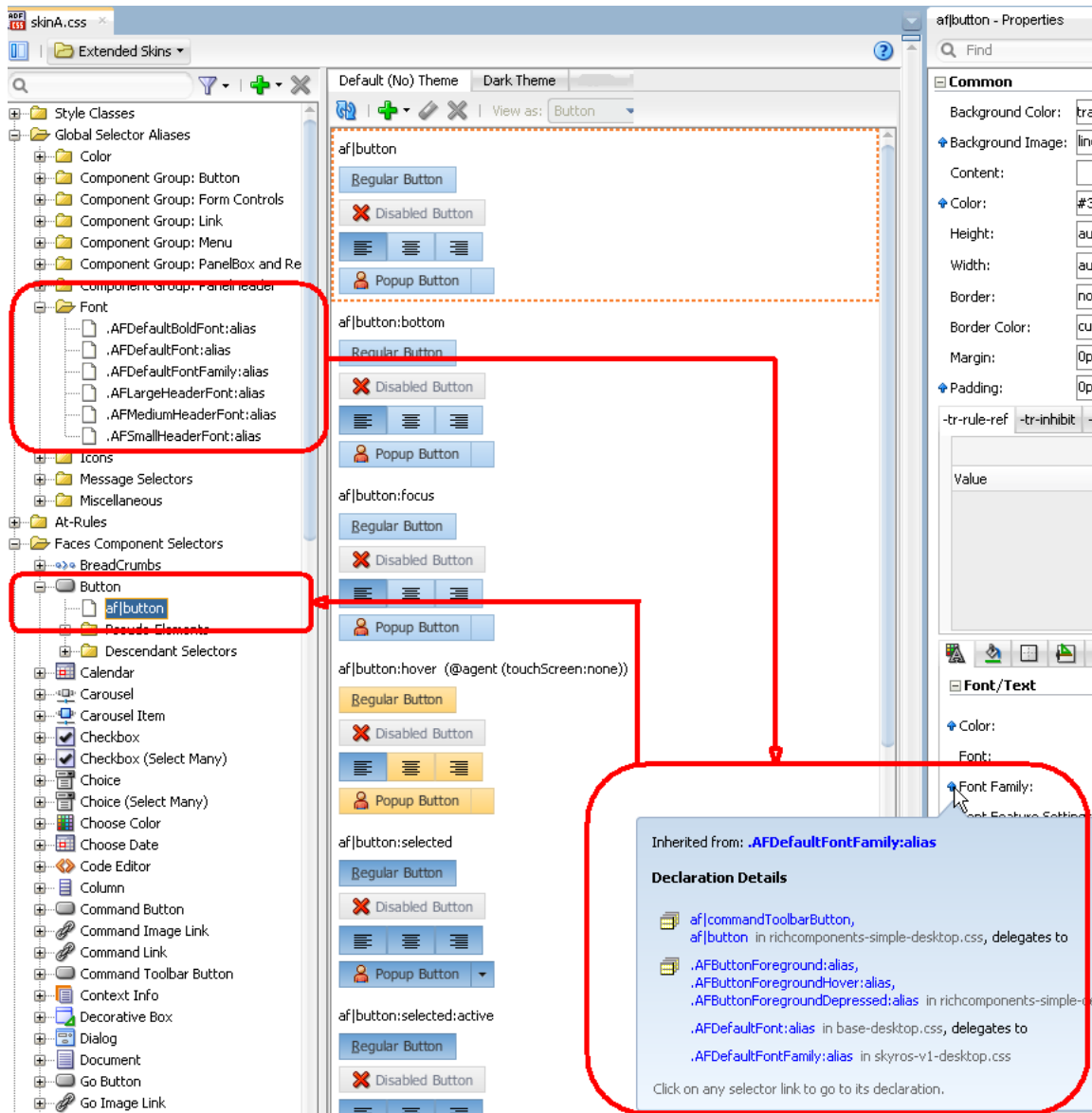
Figure 8–1 Component Selector Inheriting Value from Global Selector Alias
