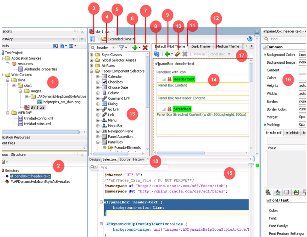
Figure 3–2 ADF Skin Selectors Editor
