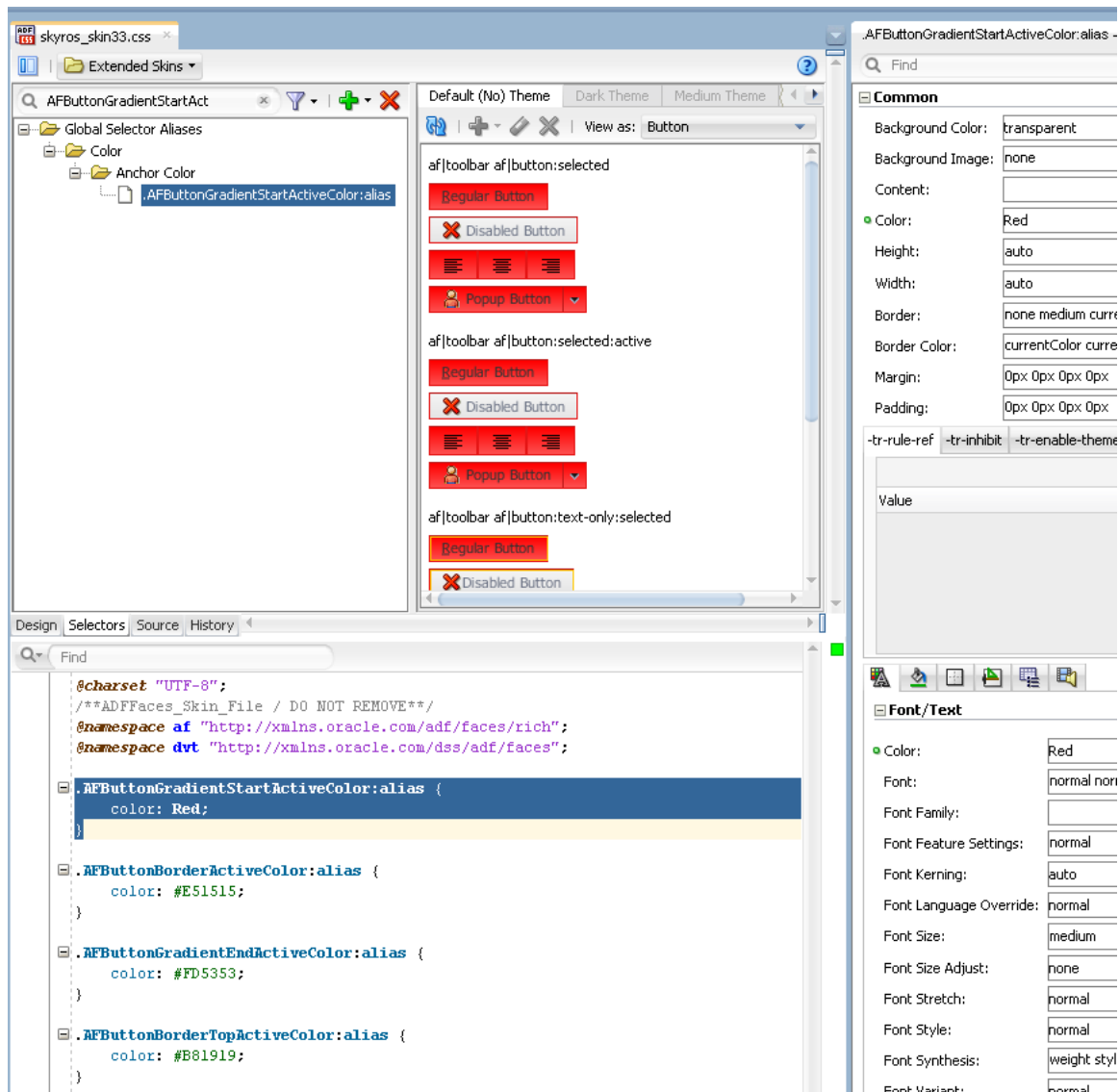
Figure 6–4 Modified Anchor Color and Effect on Derivative Colors
