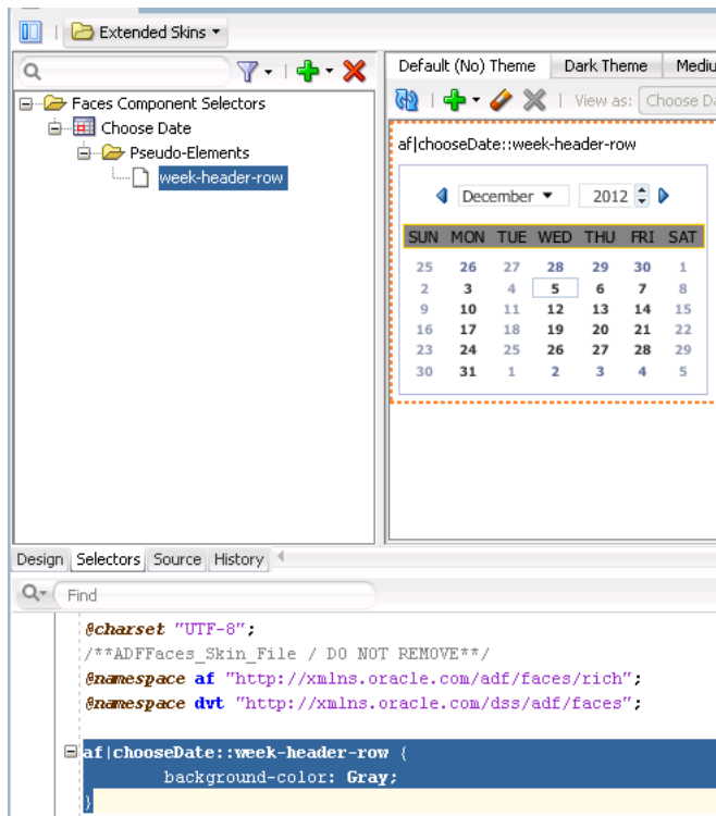
Figure 2–3 Pseudo-Elements for the Choose Date Component
