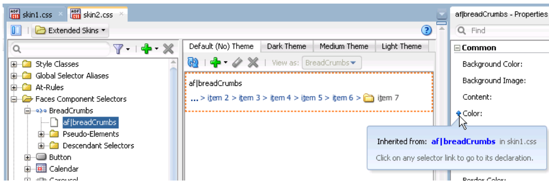
Figure 3–8 Information Tip Showing Hyperlink to Navigate to Source Declaration
