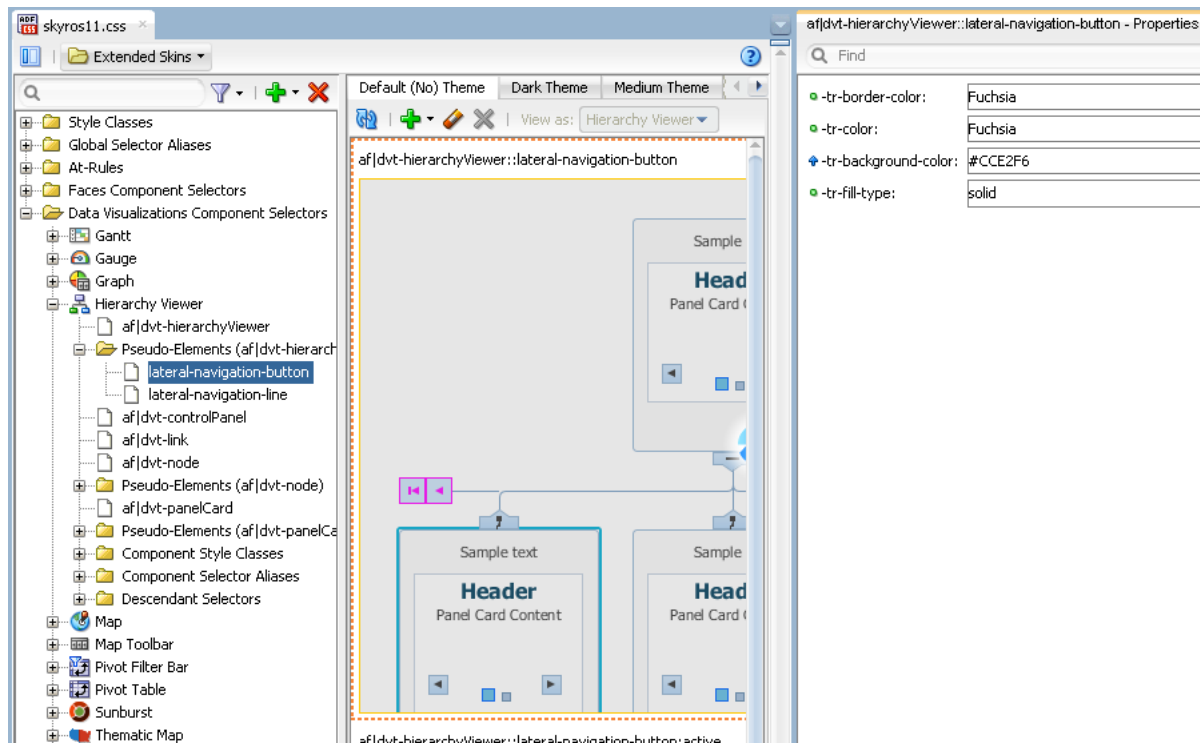
Figure 5–6 Properties for the hierarchyViewer Component lateral-navigation-button Pseudo-Element
