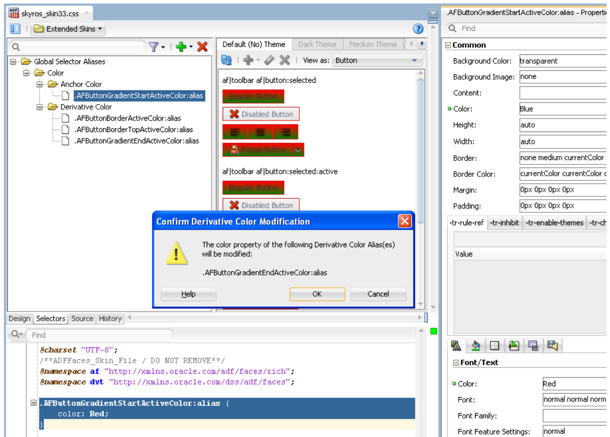
Figure 6–5 Overriding a Derivative Color
