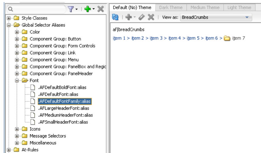
Figure 8–6 Modifying a Global Selector Alias
