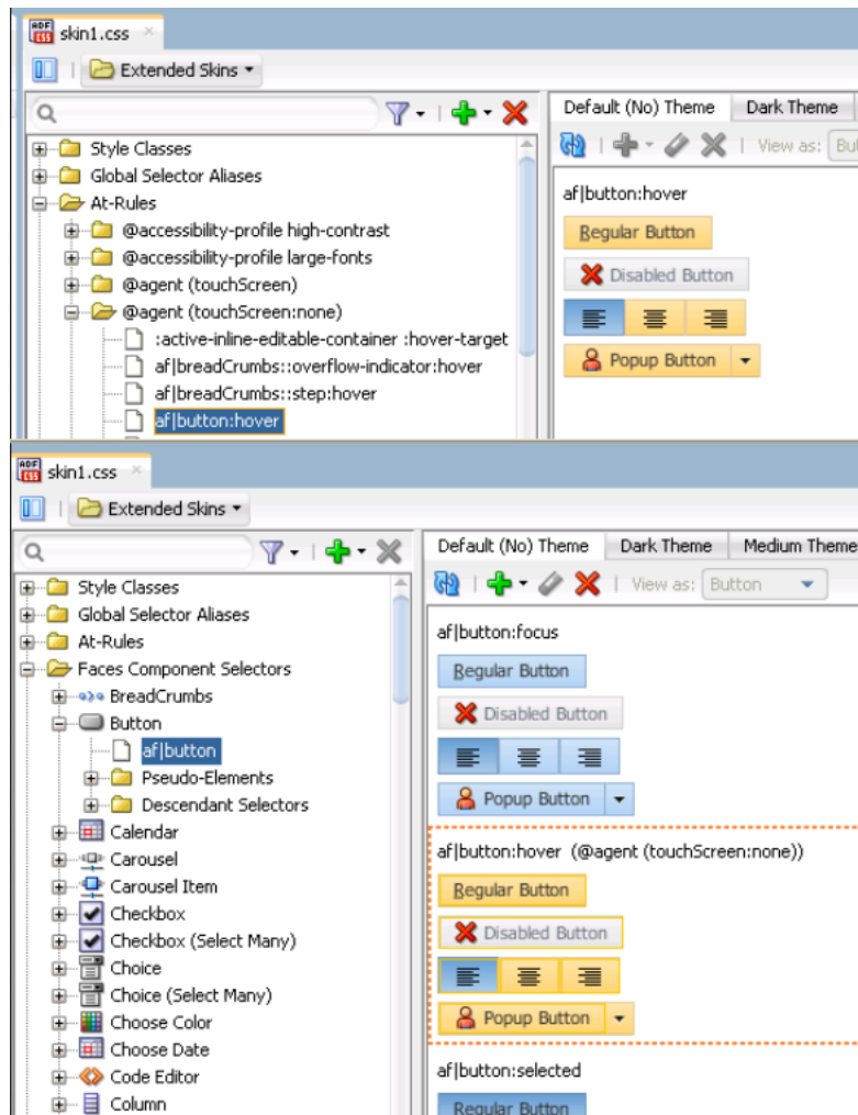
Figure 10–2 @agent (touchScreen:none) at-rule in the Selector Tree
