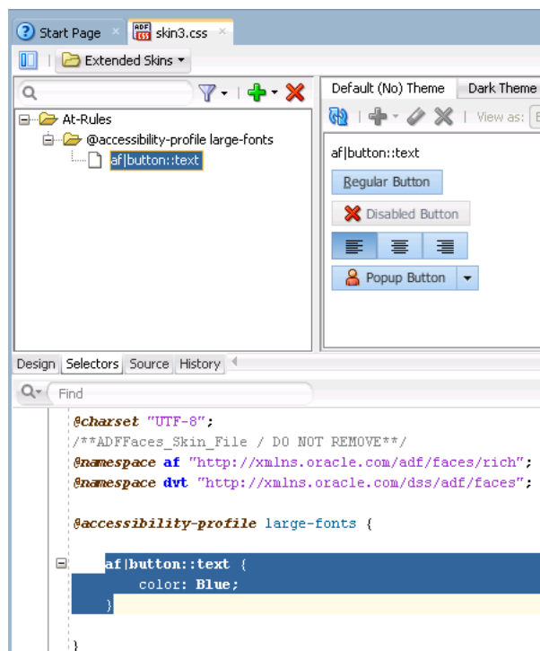
Figure 10-4 At-Rule in the Selector Tree and Source Editor
