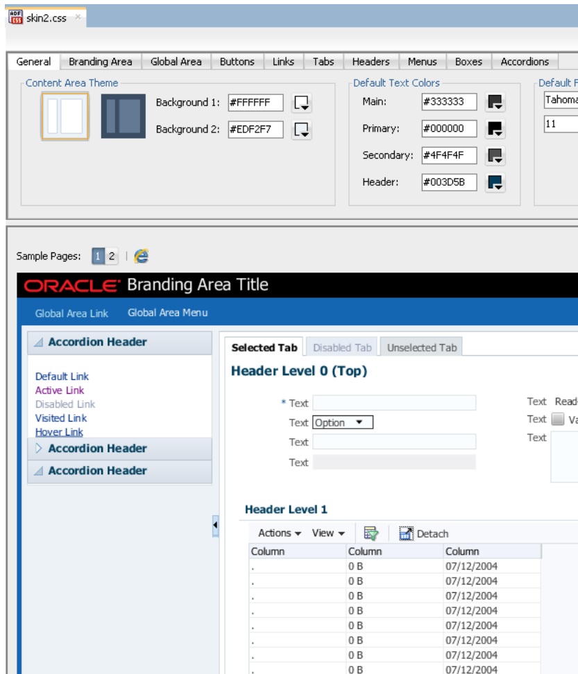
Figure 4–1 Newly-Created ADF Skin in the Design Tab
