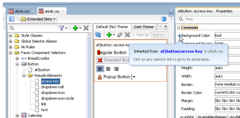
Figure 3–12 Inheriting a Property Value from an Extended Skin
