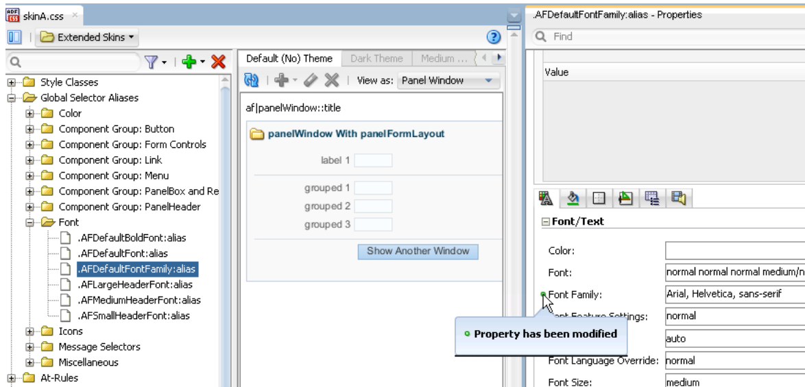
Figure 8–2 ADF Skin Changing a Global Selector Alias
