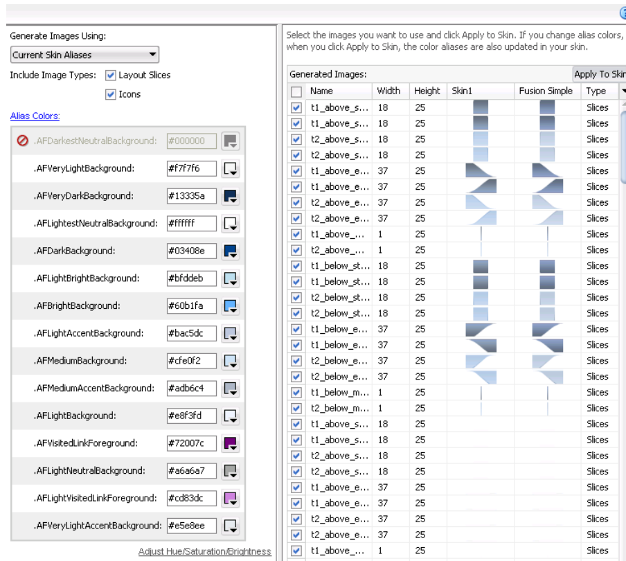
Figure 6–11 Images Editor for an ADF Skin
