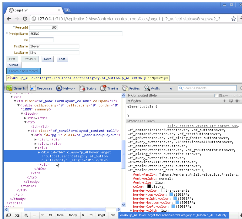
Figure 11–2 Uncompressed CSS from an ADF Skin
