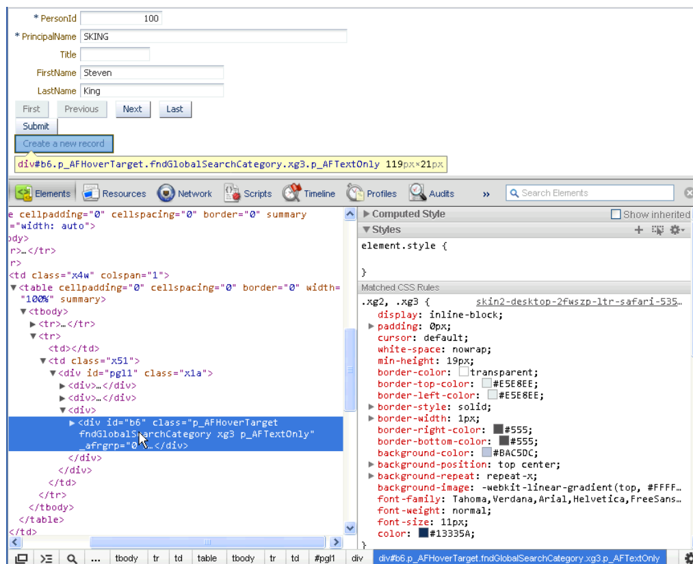
Figure 11–1 Compressed CSS from an ADF Skin
