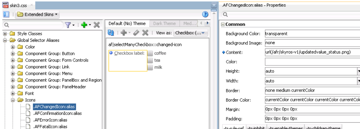
Figure 2–5 Global Selector Aliases for Icons
