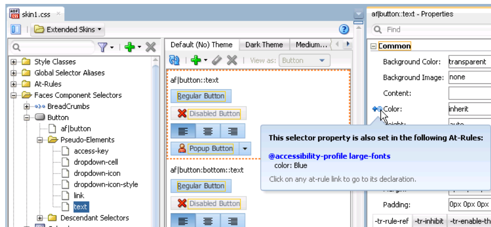
Figure 10–5 Properties Window with an At-Rule set on a Property
