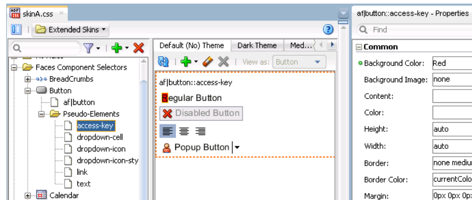
Figure 3–11 Declaration of a Property Value
