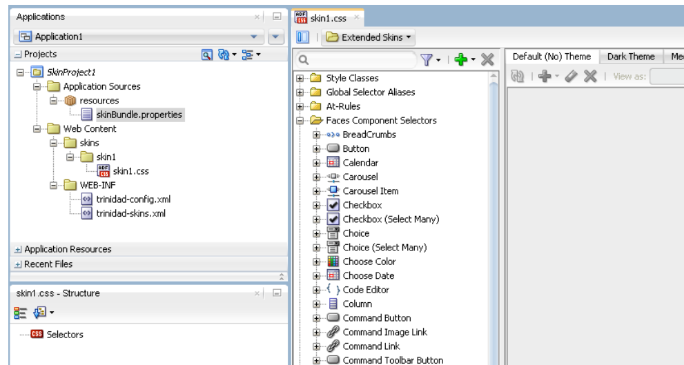
Figure 4–2 Newly-Created ADF Skin in the Selectors Editor
