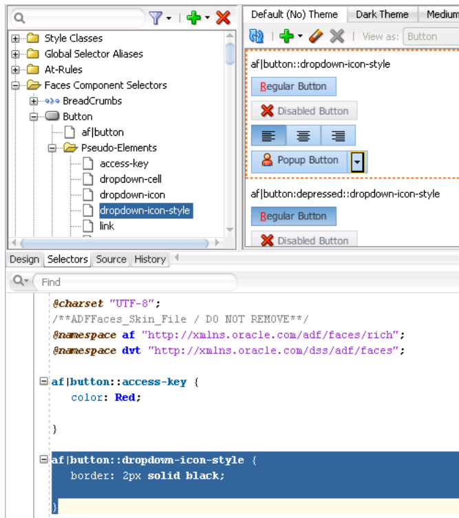
Figure 5–3 Button Component with Modified Selectors
