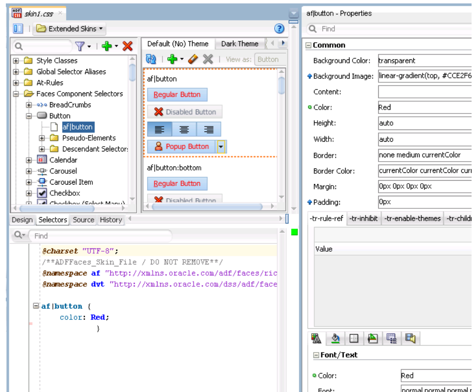
Figure 2–2 Button Component's Skin Selector
