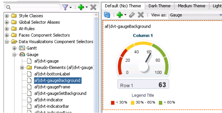
Figure 5–4 ADF Data Visualization Component Selectors
