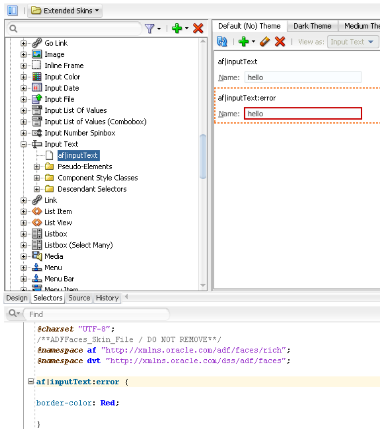
Figure 5-15 Style Properties for an inputText Component's Error Message
