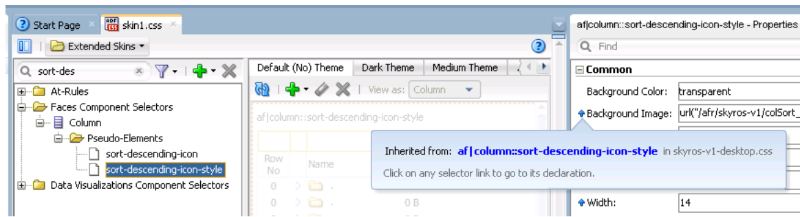
Figure 6–7 Inherited Values for the sort-descending-icon-style Selector
