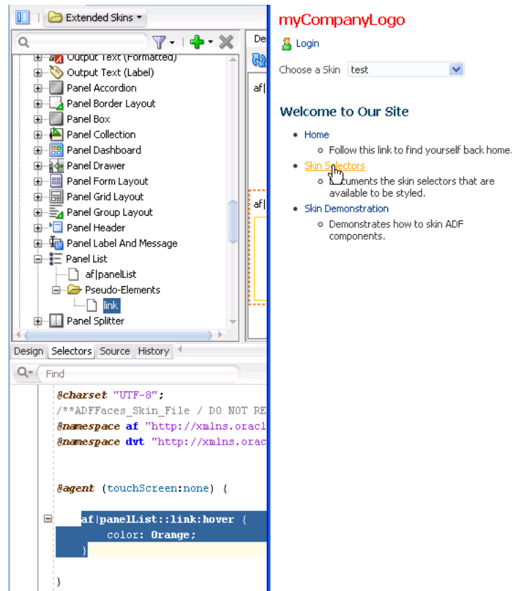
Figure 2–9 Pseudo-Class Syntax and Runtime Behavior for a Panel List Link
