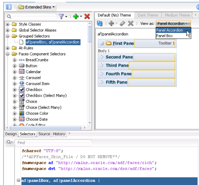
Figure 2–7 Grouped Selectors in the Selector Tree
