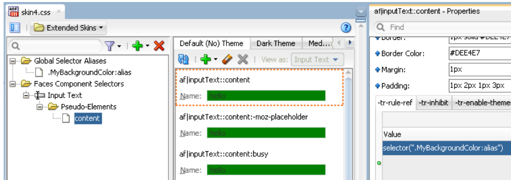
Figure 8-7 inputText Component's content Pseudo-Element
