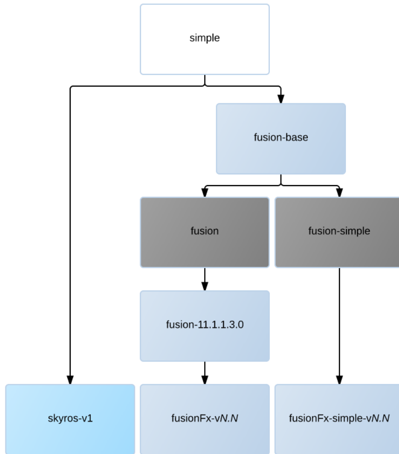
Figure 1–4 Inheritance Relationship of ADF Skin Families Provided by Oracle ADF
