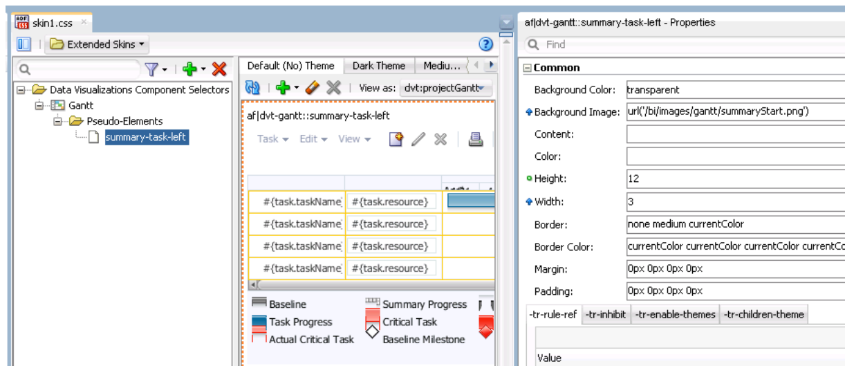
Figure 5–7 Properties for the gantt Component summary-task-left Pseudo-Element
