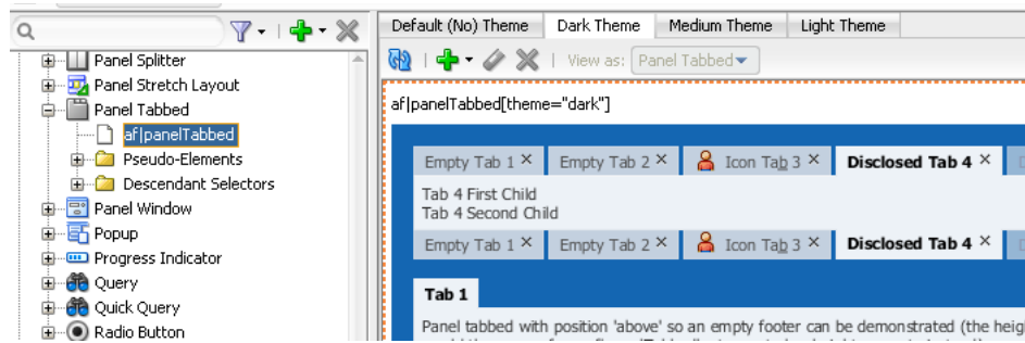
Figure 5–19 Dark Theme in Selectors Editor
