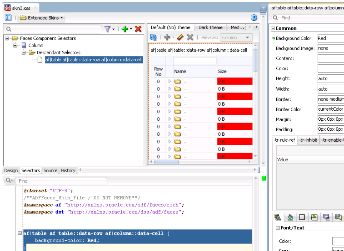
Figure 2–8 Descendant Selectors in the Selector Tree
