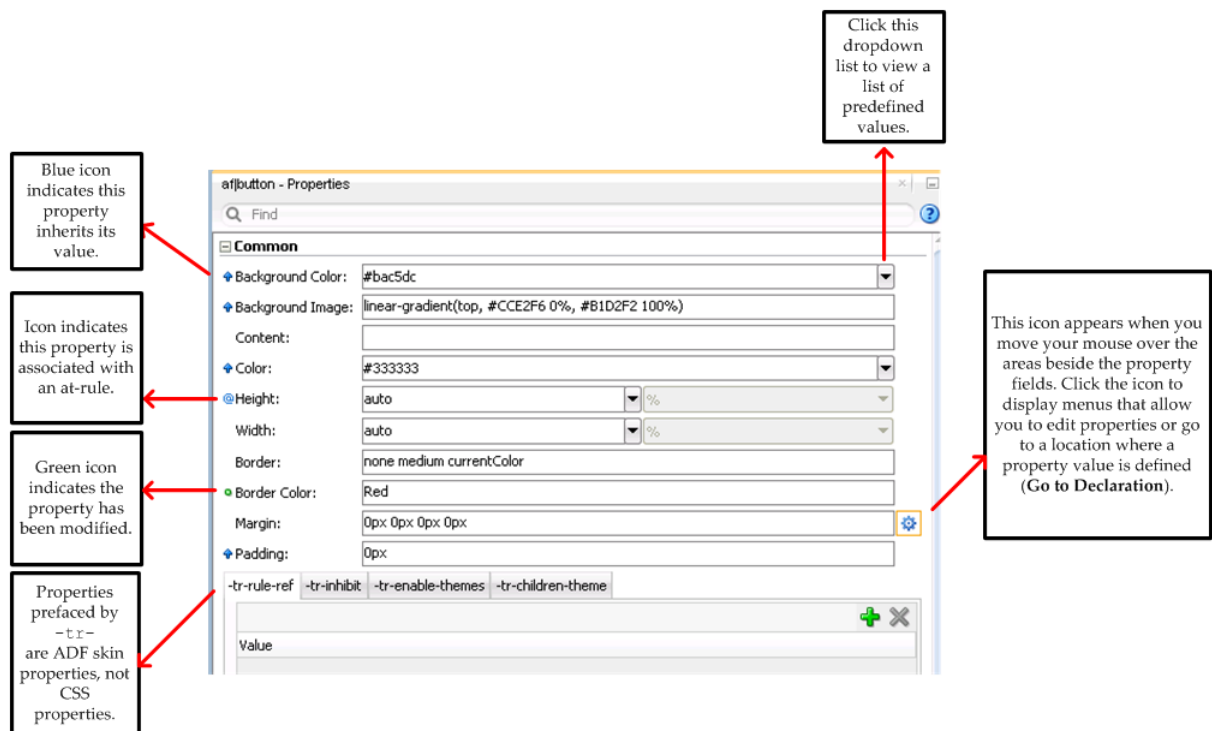
Figure 3-7 Controls in the Properties Window for ADF Skins
