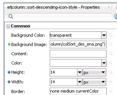
Figure 6–10 Properties Window After Importing an Image into an ADF Skin
