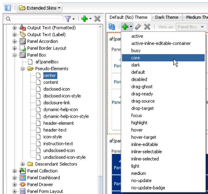
Figure 2–11 Pseudo-classes for the center Pseudo-element
