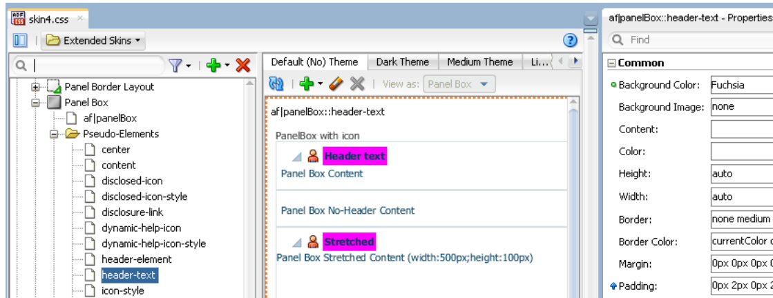
Figure 9-4 Setting Background Color for a panelBox Component
