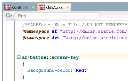
Figure 3–14 Property Value Defined in Extended ADF Skin
