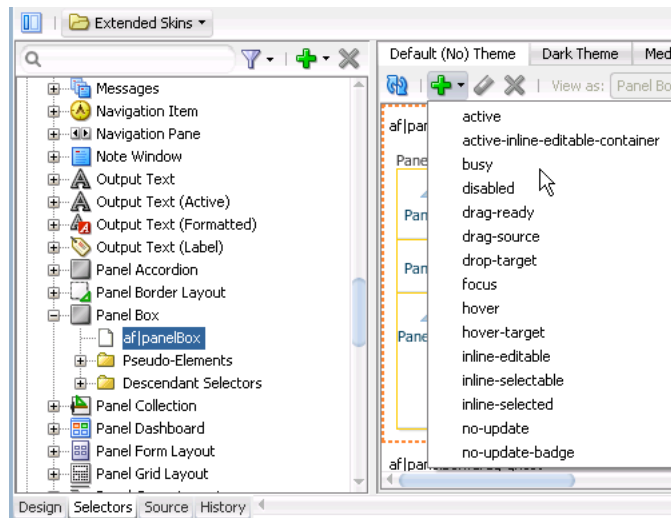
Figure 2–10 Pseudo-classes for the panelBox Component's Selector
