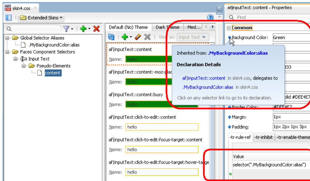
Figure 8–8 Global Selector Alias Applied to inputText Component
