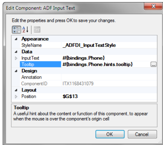
Figure 6-18 Tooltip Property of Input Text Component
