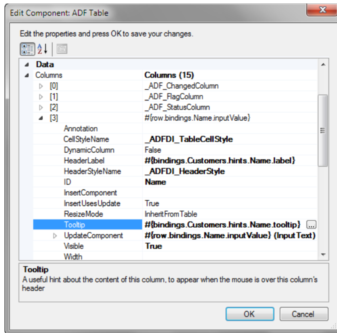
Figure 7–20 Tooltip for ADF Table Column Header at Design-time
