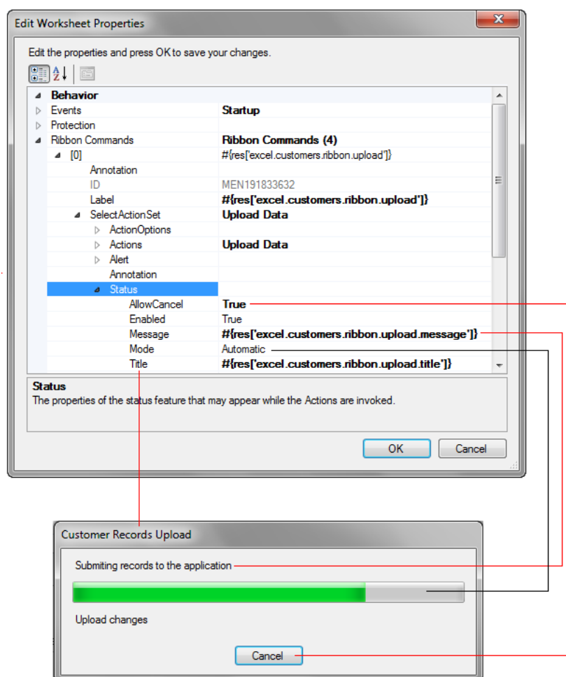
Figure 8–8 Status Message Properties in an Action Set
