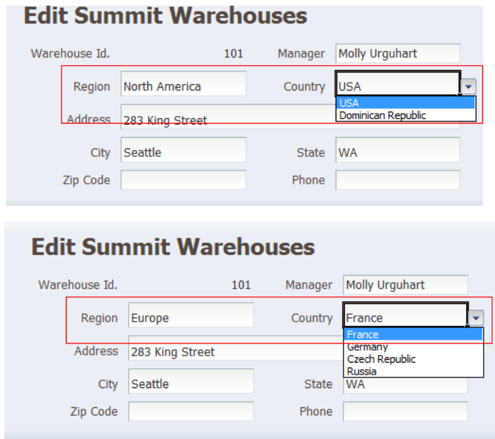
Figure 8–29 List of Values and Dependent List of Values
