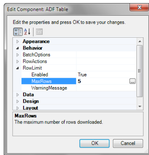
Figure 7–24 Limiting Number of Rows of an ADF Table Component
