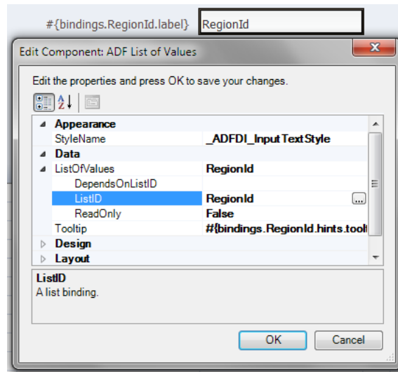
Figure 6–11 ADF List of Values Component
