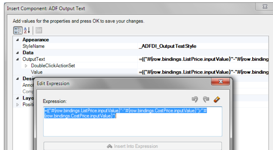
Figure 6–22 ADF Output Text Component Displaying Calculated Data
