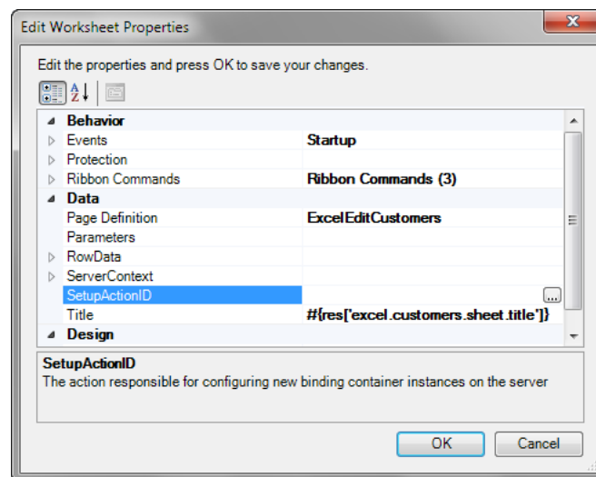
Figure 7-27 SetupActionID Property in Edit Worksheet Properties Dialog
