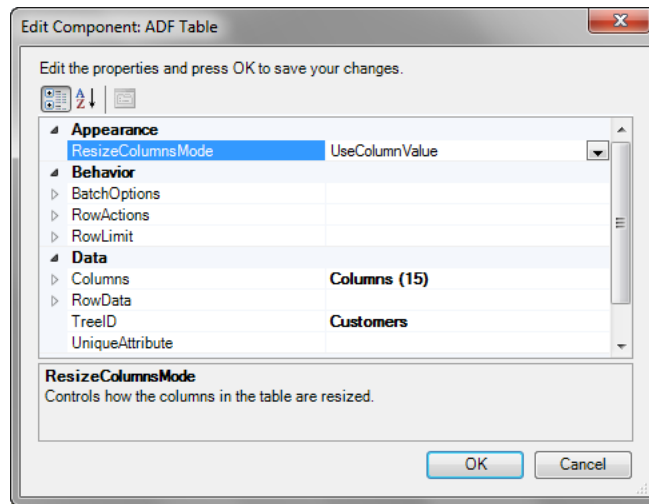
Figure 7–17 ResizeColumnsMode Property in design-time
