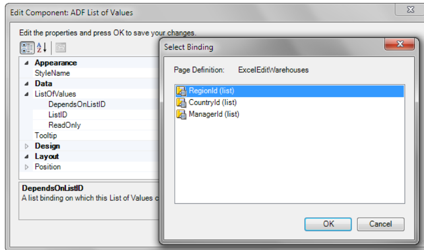
Figure 8–30 Design Time Dependent List of Values in an Excel Worksheet
