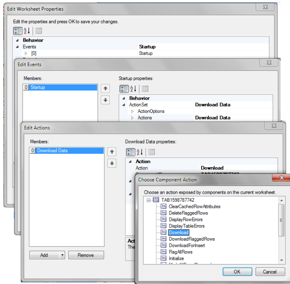
Figure 7-7 Action Set Downloading Data to an ADF Table Component
