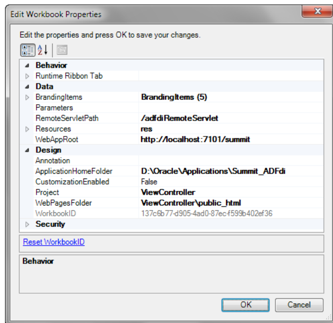
Figure 4–6 Edit Workbook Properties Dialog
