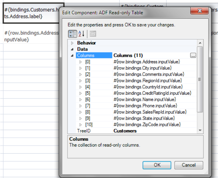
Figure 7-22 ADF Read-only Table Component at Design Time
