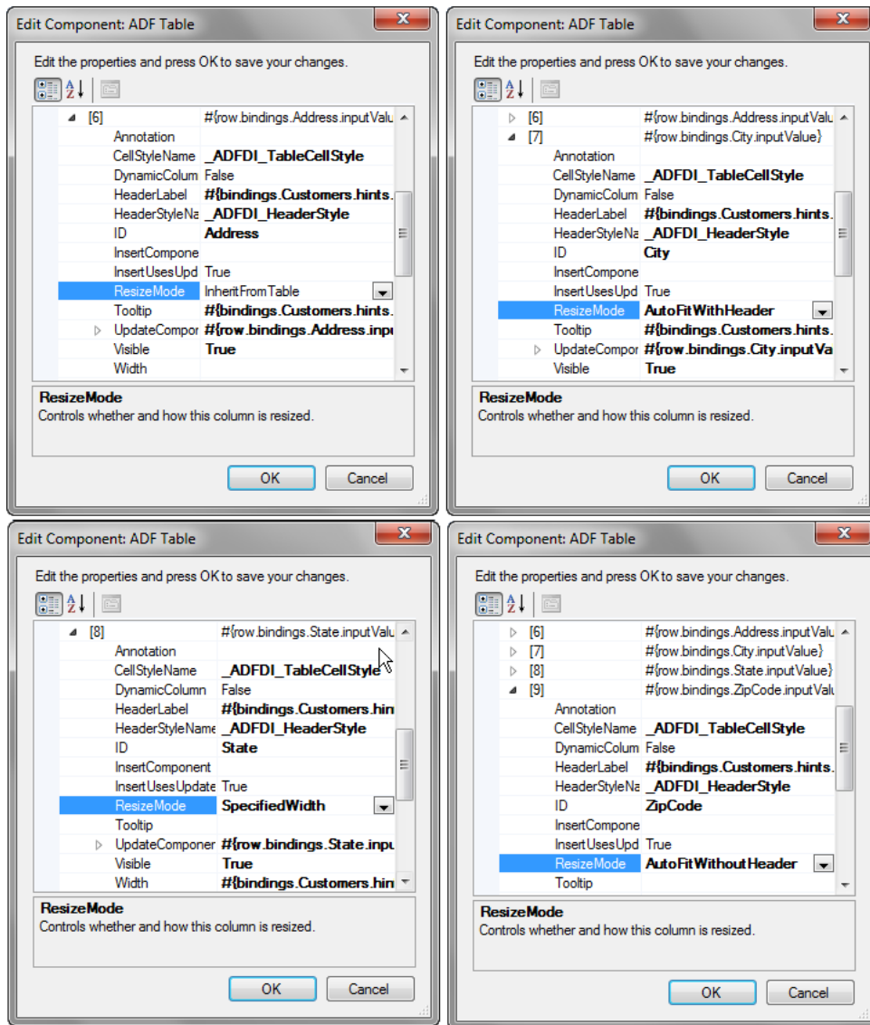
Figure 7–18 ResizeMode Property in design-time
