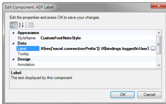
Figure 6–20 ADF Label Component That Displays Output from a Managed Bean at Runtime
