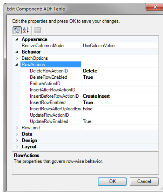
Figure 7-9 ADF Table RowActions Properties to Update Data
