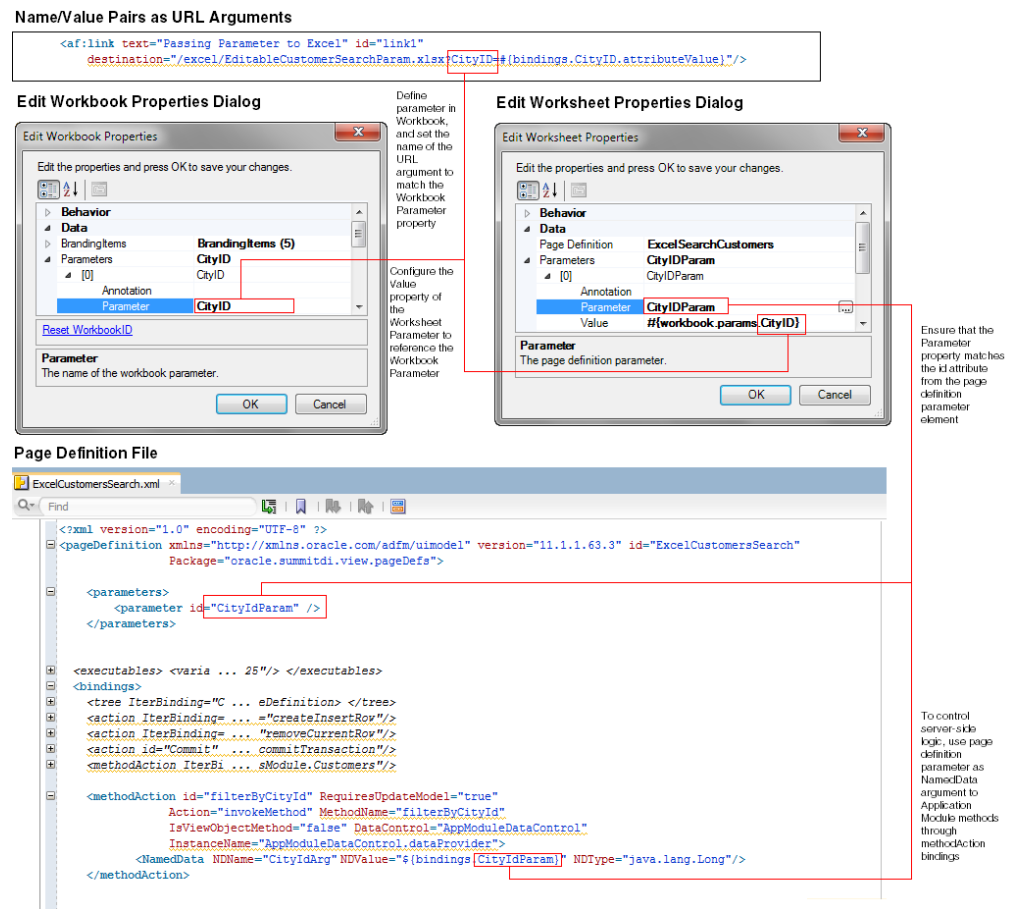
Figure 14-3 Configuring Workbook and Fusion Web Application to Pass Parameters
