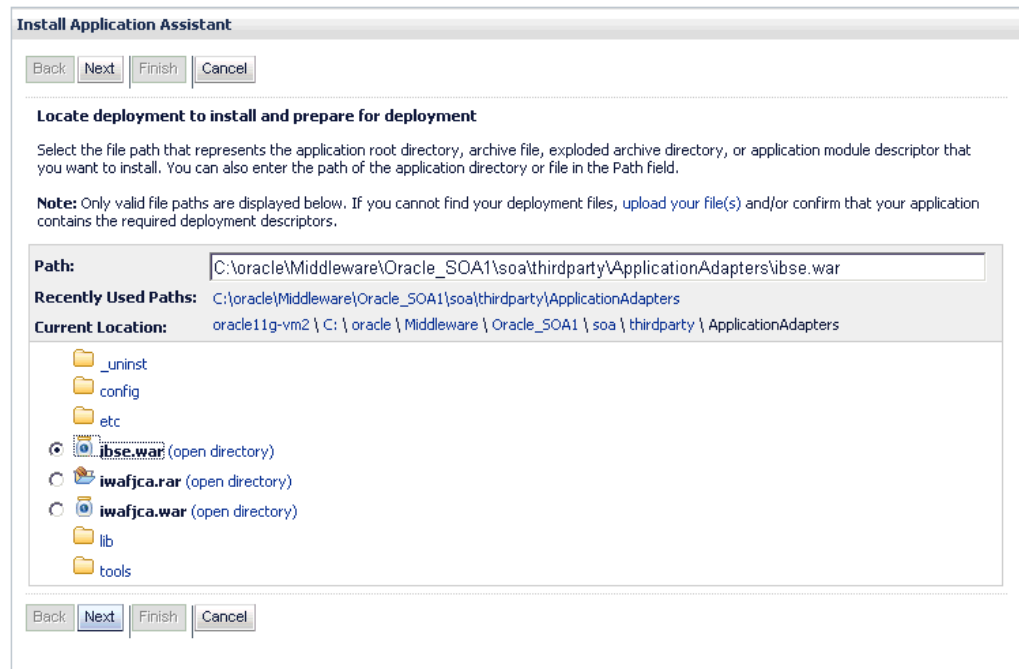
Figure 2–28 Install Application Assistant
