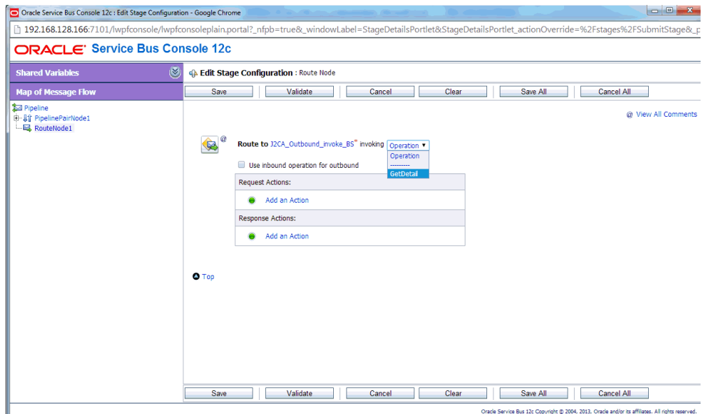
Figure 2–94 Edit Stage Configuration
