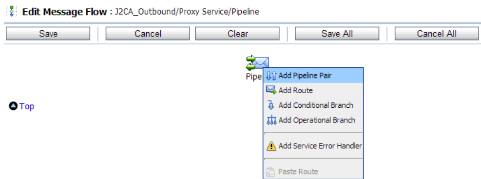
Figure 2–29 Add Pipeline Pair Option
