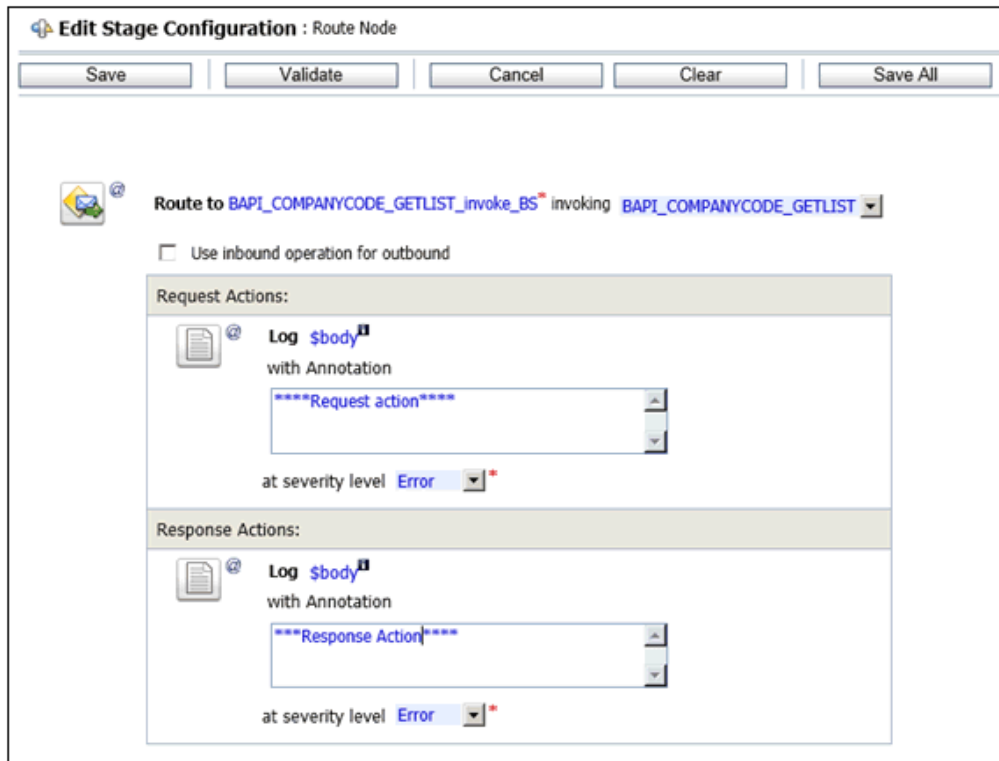
Figure 2–113 Final Pipeline Structure
