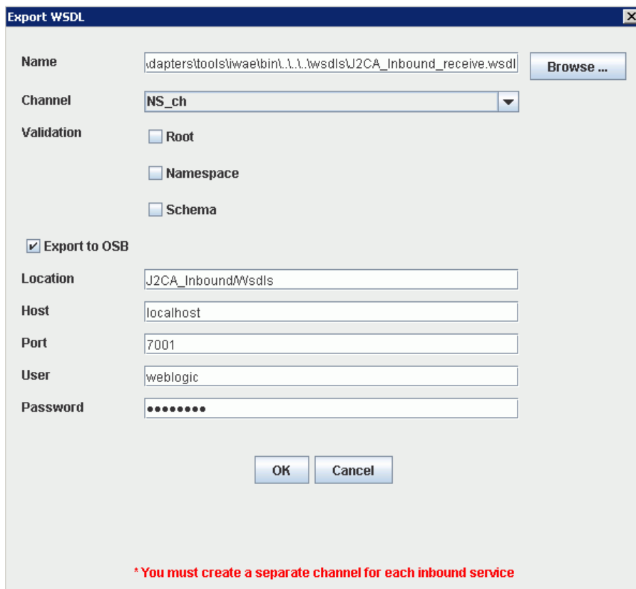
Figure 2–45 Export WSDL Dialog
