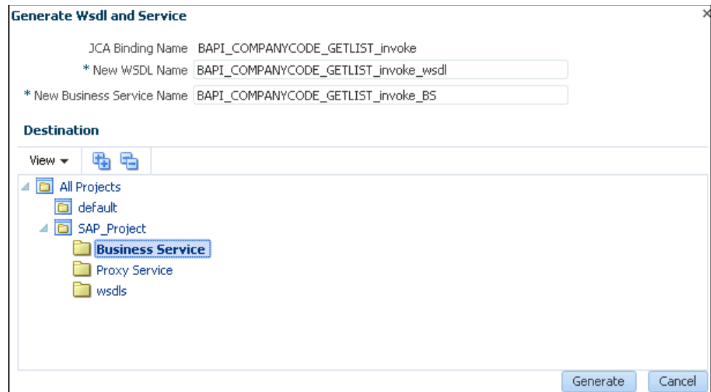
Figure 2–105 Generate WSDL and Service Page
