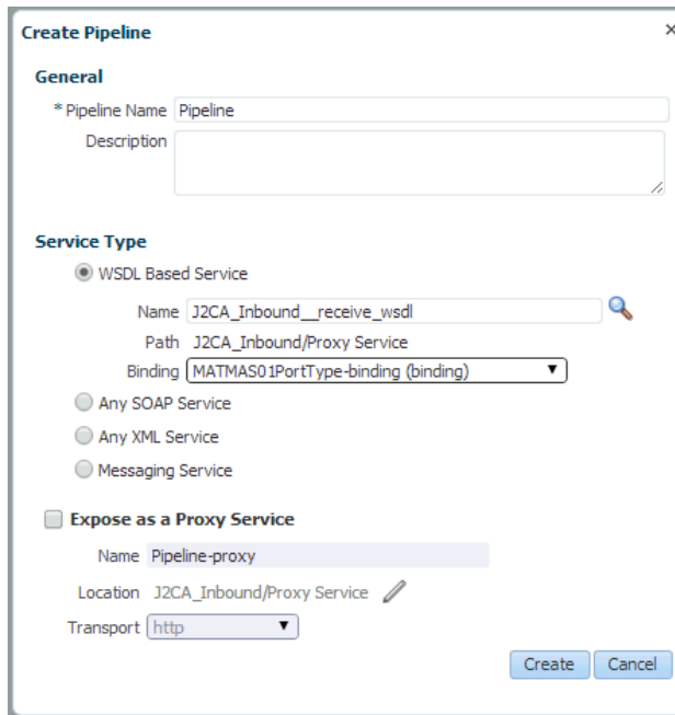
Figure 2–60 Create Pipeline Window
