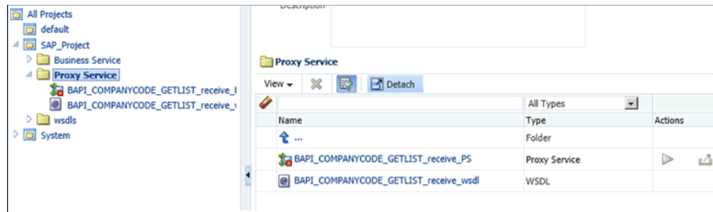
Figure 2–109 Checking the WSDL and Service Resources
