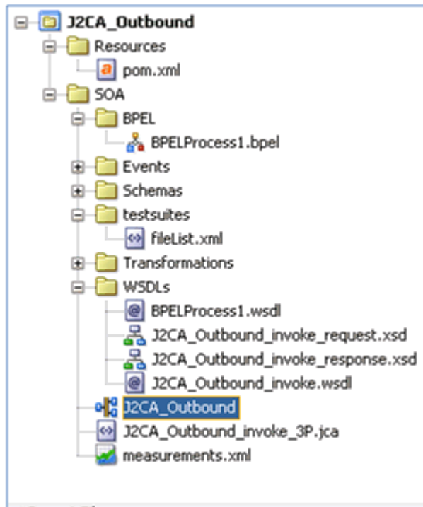
Figure 1–1 Created BPEL Process
