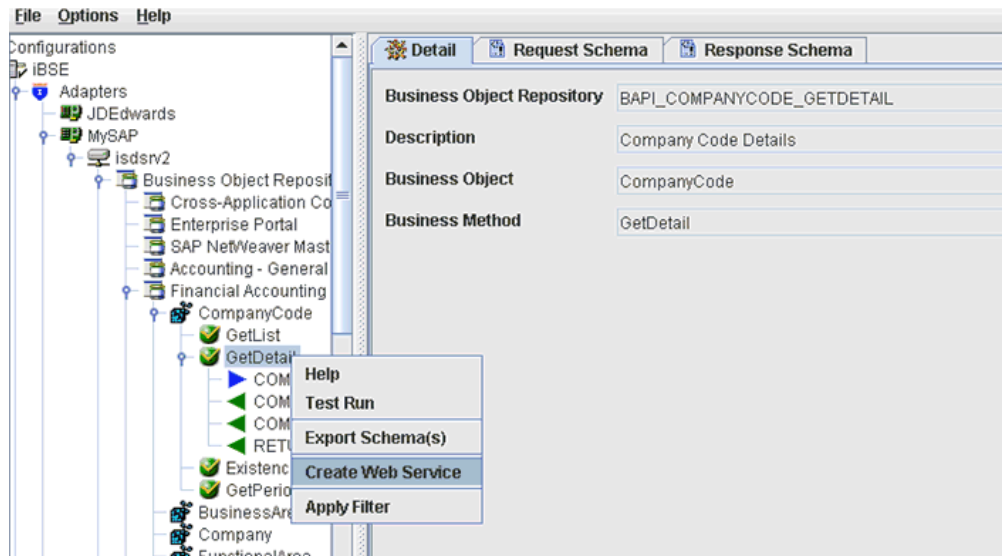
Figure 2–74 Create Web Service Option
