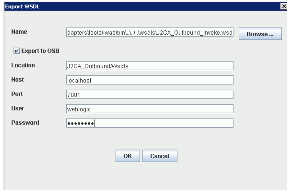
Figure 2–10 Export WSDL Dialog
