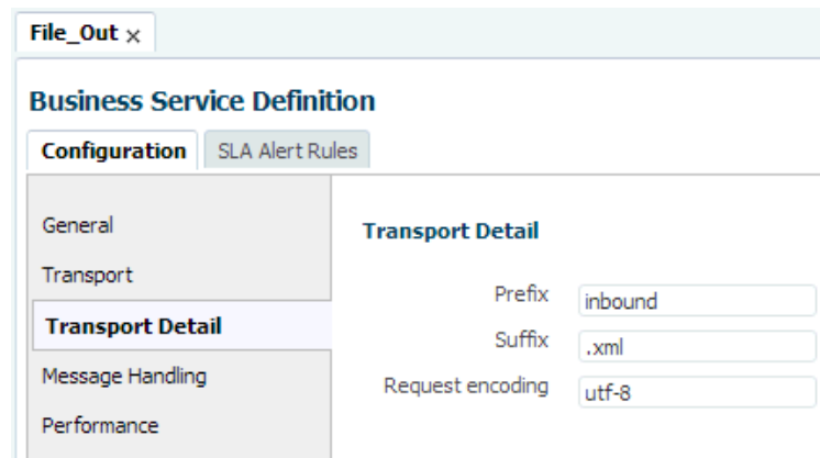
Figure 2-55 Transport Detail Page
