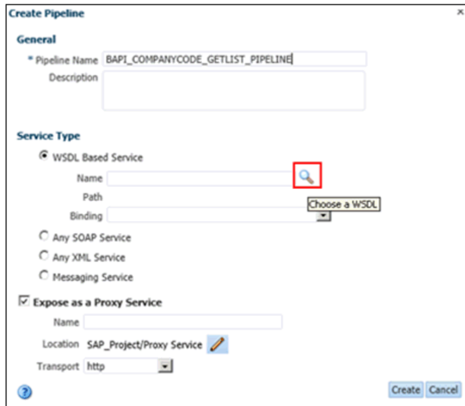
Figure 2–110 Create Pipeline Window
