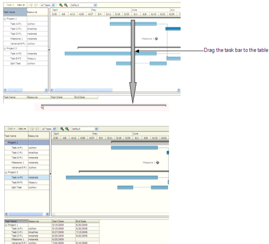
Figure 37-5 Dragging and Dropping an Object
