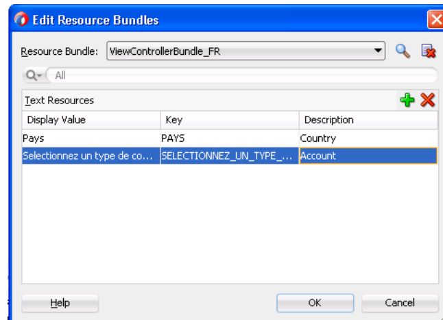
Figure 34-5 Adding Values to a Resource Bundle
