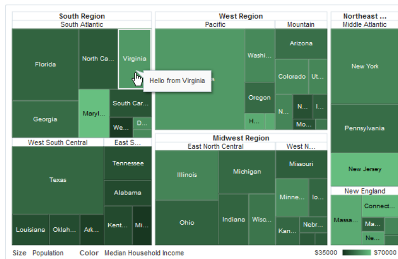
Figure 31-36 Treemap Showing Popup on Mouse Hover
