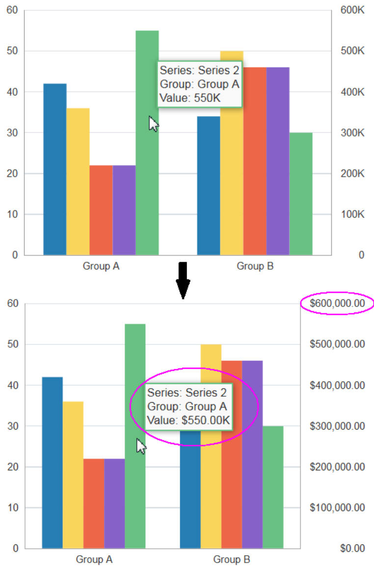
Figure 23-43 Bar Chart Configured to Display Currency Values
