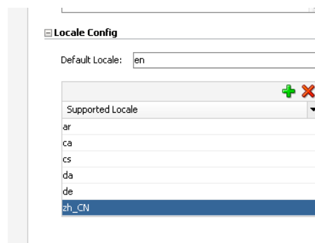
Figure 34-6 Adding a Locale to faces-config.xml
