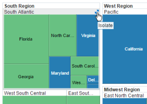
Figure 31-23 Isolate Icon Displayed on Treemap Group Header
