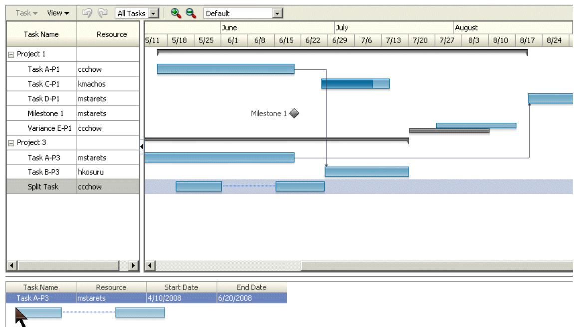
Figure 27-26 Project Gantt Chart as Drag Source
