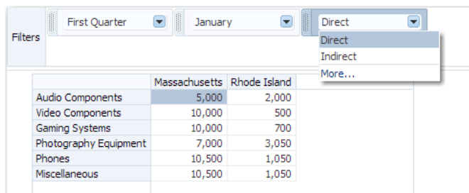
Figure 26-32 Pivot Table and Pivot Filter Bar After Pivot
