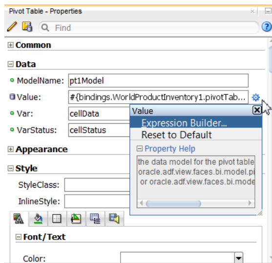
Figure 26-27 Pivot Table Value Attribute Dropdown Menu
