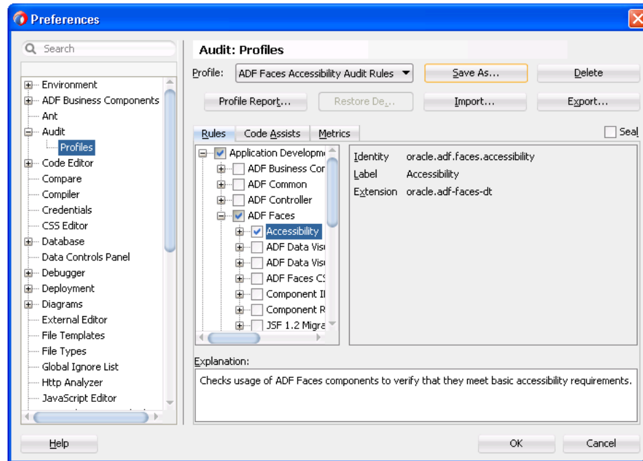
Figure 35-5 Audit Profile Settings for ADF Faces Accessibility
