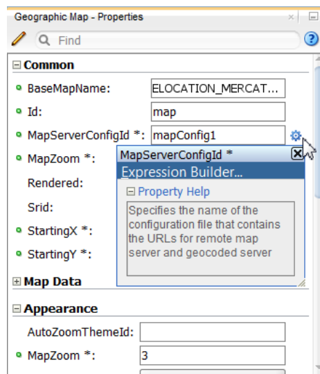
Figure 29-15 Geographic Map MapServerConfigId Attribute Dropdown Menu
