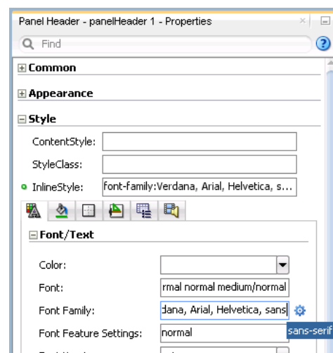
Figure 33-4 Setting an inlineStyle Attribute
