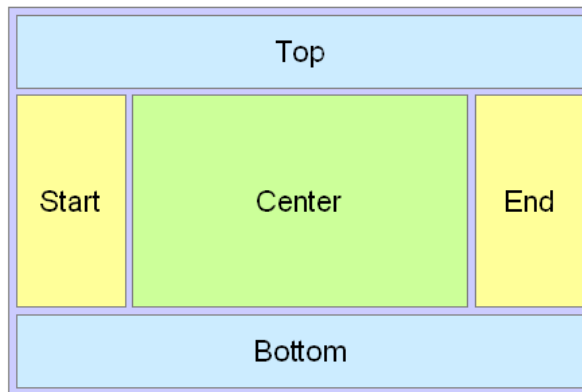
Figure 9-17 Facets in the panelStretchLayout Component
