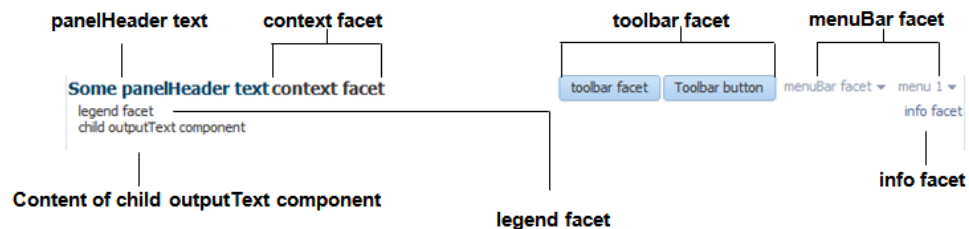
Figure 9-60 panelHeader and Its Facets
