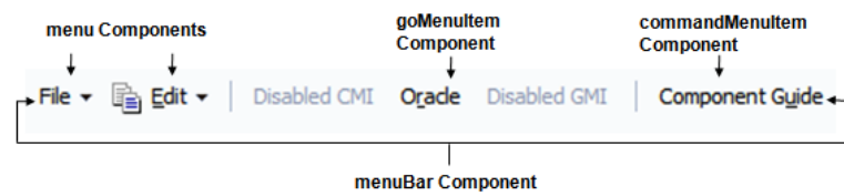
Figure 15-5 menuBar and Child Components
