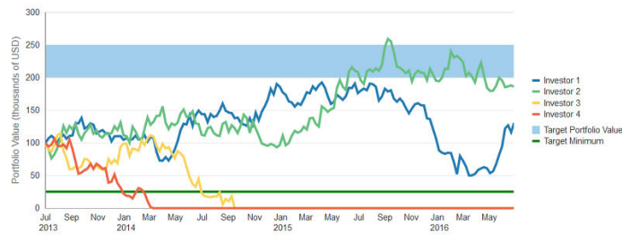
Figure 23-45 Line Chart Configured With Reference Area and Reference Line
