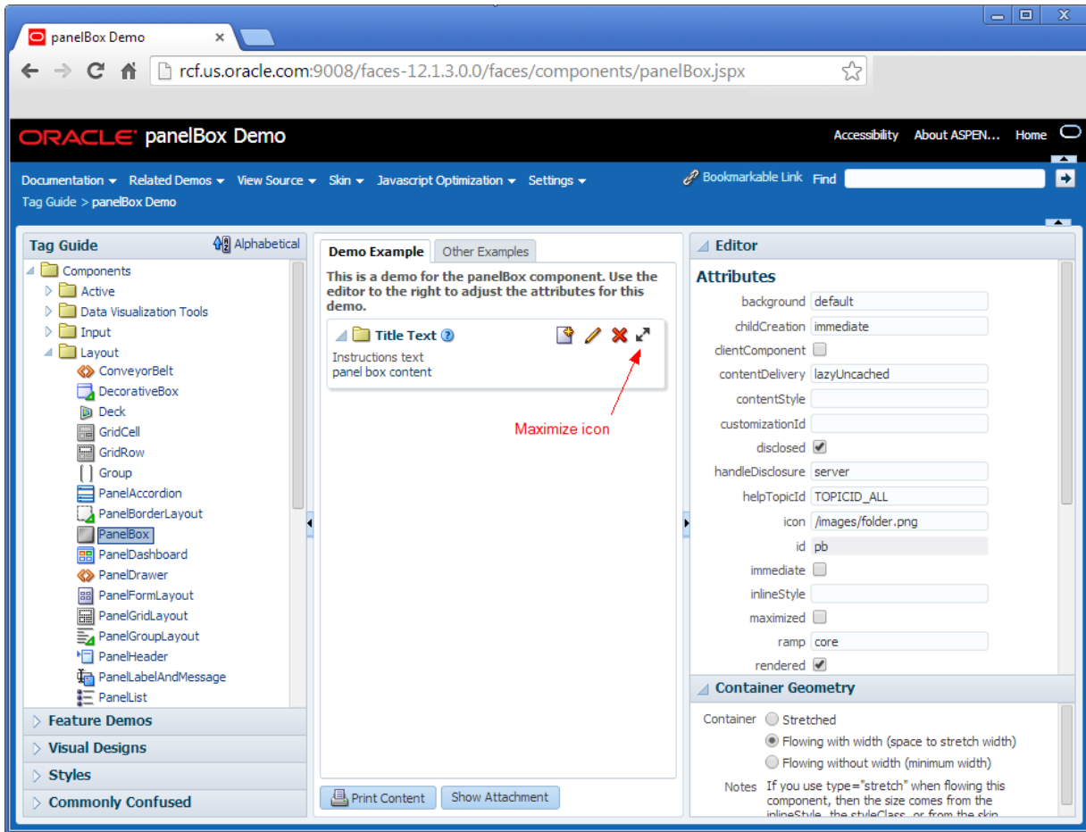
Figure 9-46 panelBox Demo with panelBox at Normal Size
