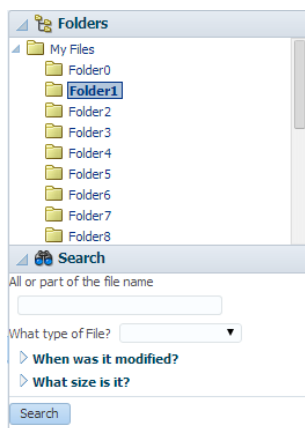
Figure 2-7 Directory Structure Panel and Search Panel
