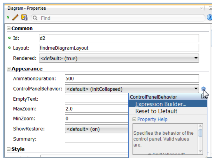
Figure 32-15 Diagram Layout Attribute Dropdown Menu
