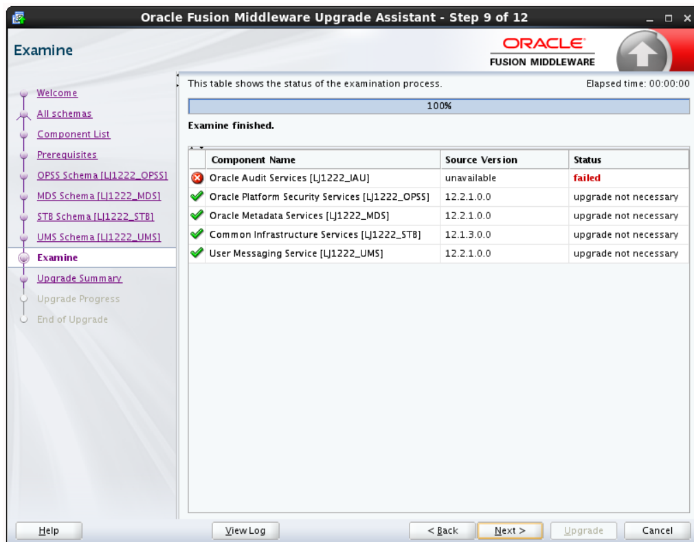
Figure A-18 Examine
