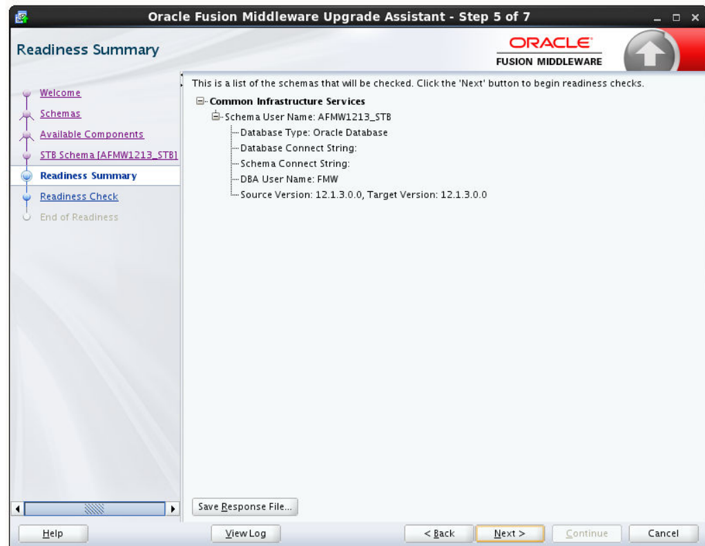
Figure A-32 Readiness Summary
