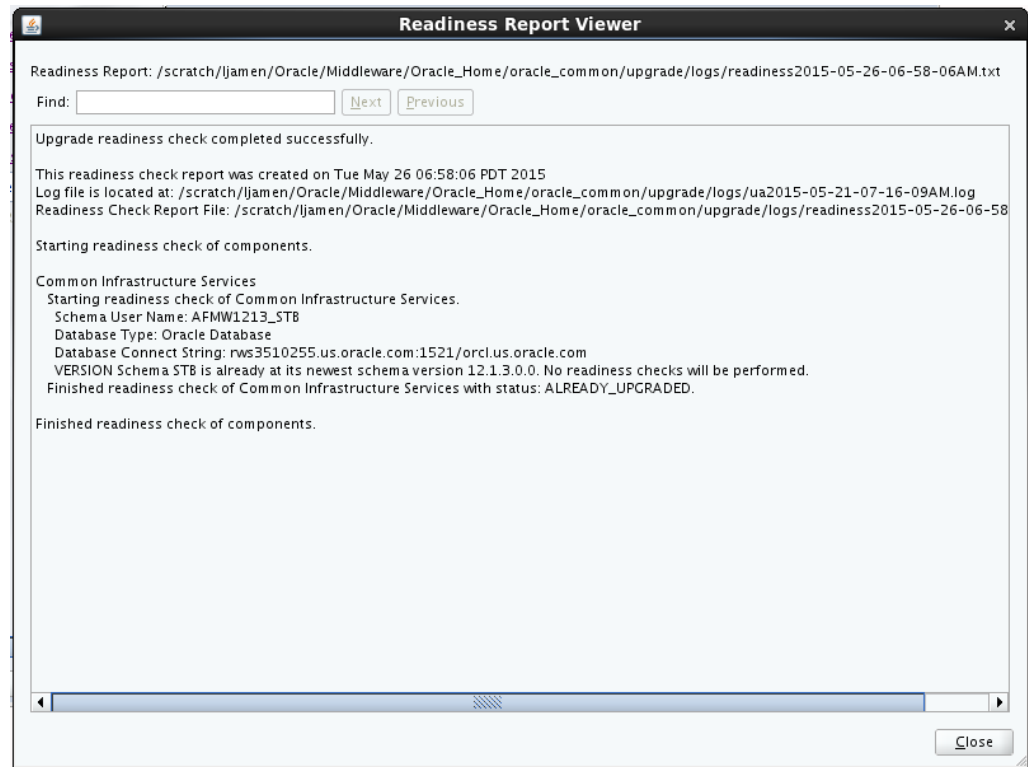
Figure A-36 Readiness Report Viewer
