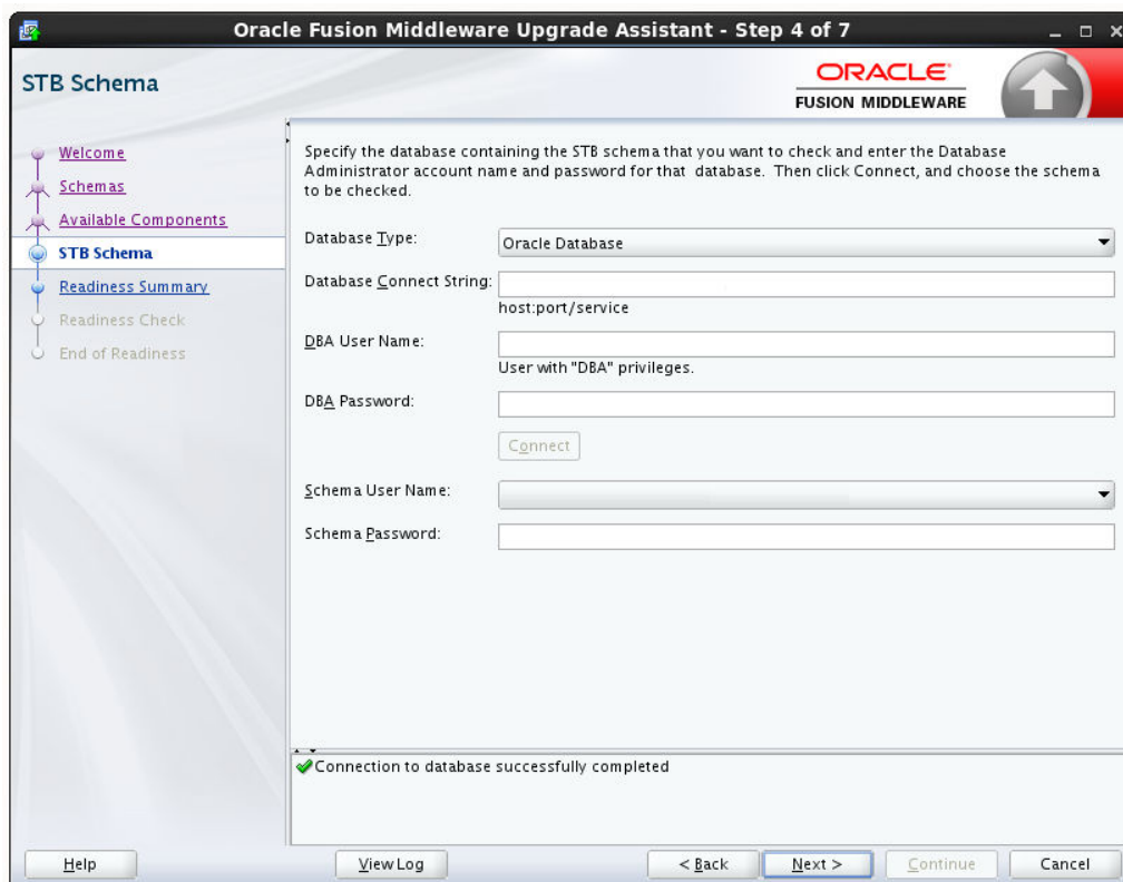
Figure A-31 Schema Credentials
