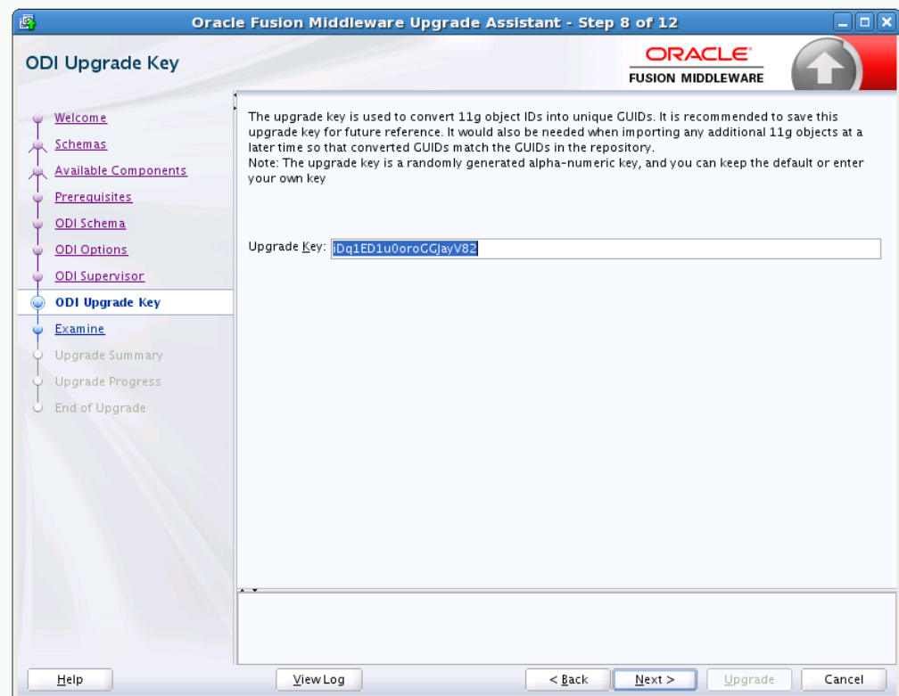
Figure A-12 Oracle Data Integrator (ODI) Upgrade Key
