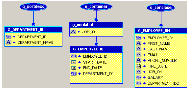
Figure 41–5 Data model with group
