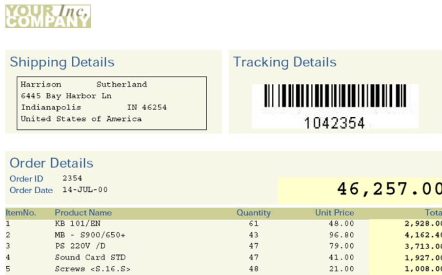
Figure 3–41 Final output of the barcode report with paper layout
