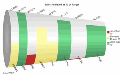
Figure 39–3 Funnel Graph
