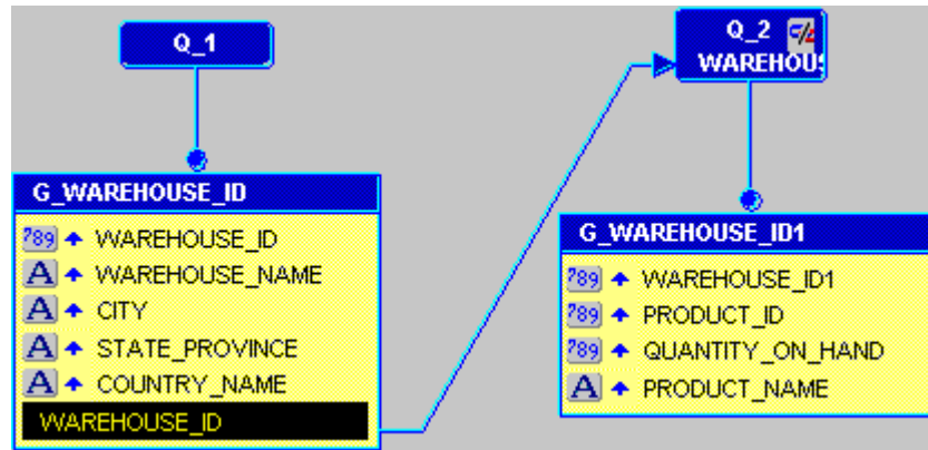
Figure 45–4 Data Model with a data link between a SQL query and an XML query
