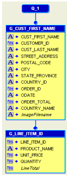
Figure 43–3 Data Model with two new formula columns
