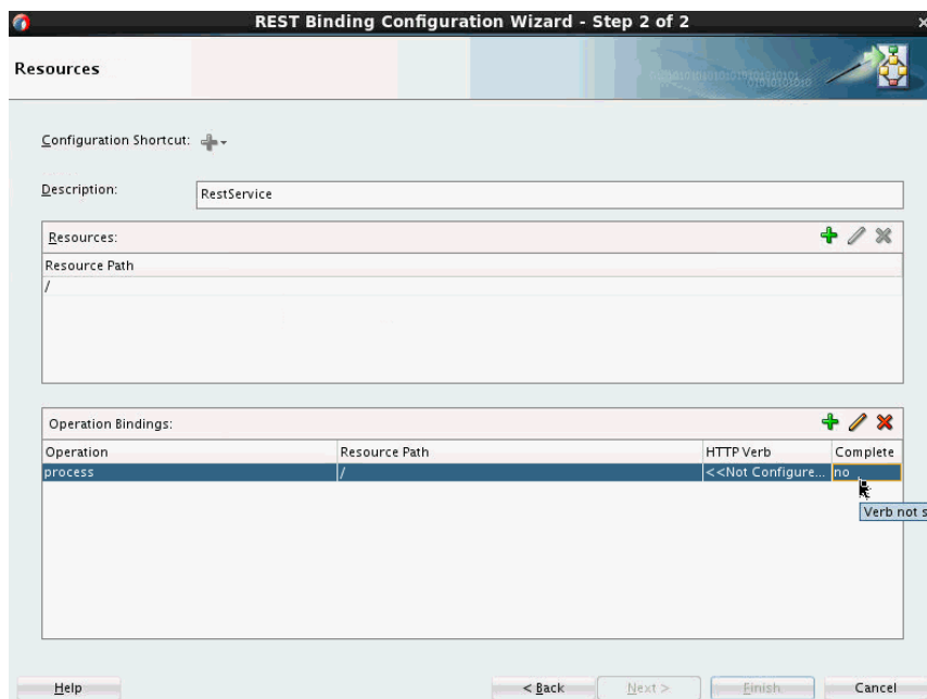
Figure 36-2 Resources Page of the REST Binding Configuration Wizard
