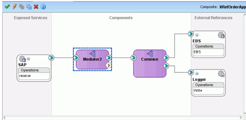
Figure 43-46 XrefOrderApp Use Case in
