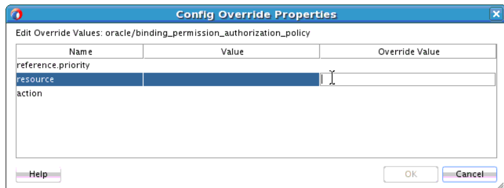
Figure 46-10 Server Policy Override Value
