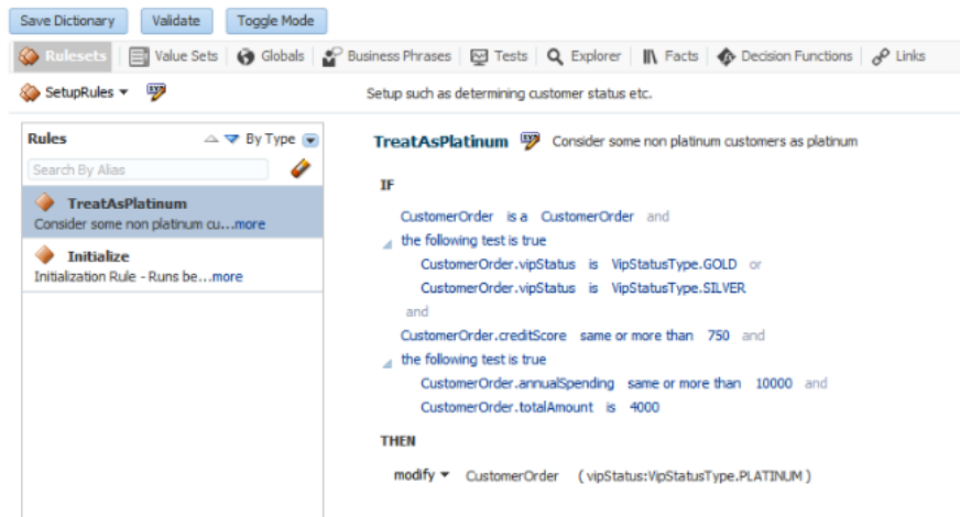
Figure 26-34 Rules Dictionary Editor Application
