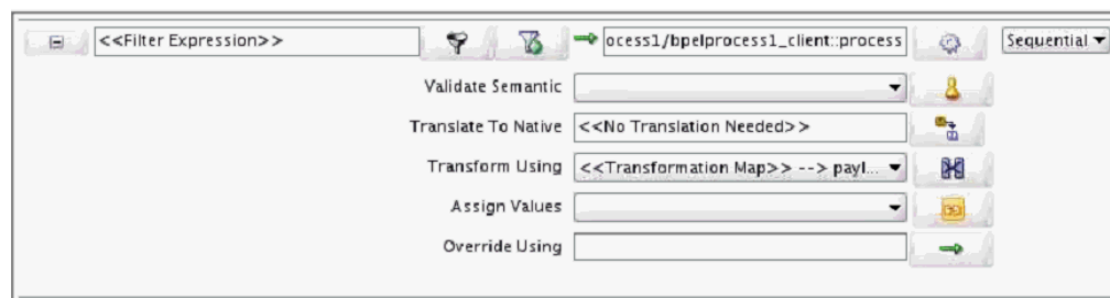
Figure 20-23 Translate To Native Option
