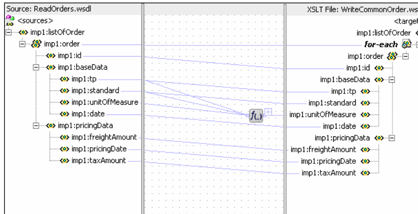
Figure 44-19 Complete impl:listOfOrder To impl:listOfOrder Transformation
