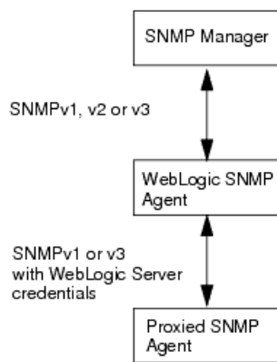
Figure 4–1 Separate Conversations for Proxied SNMP Communication
