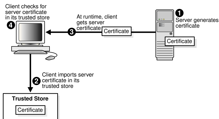
Figure 4-51 Establishing Trust
