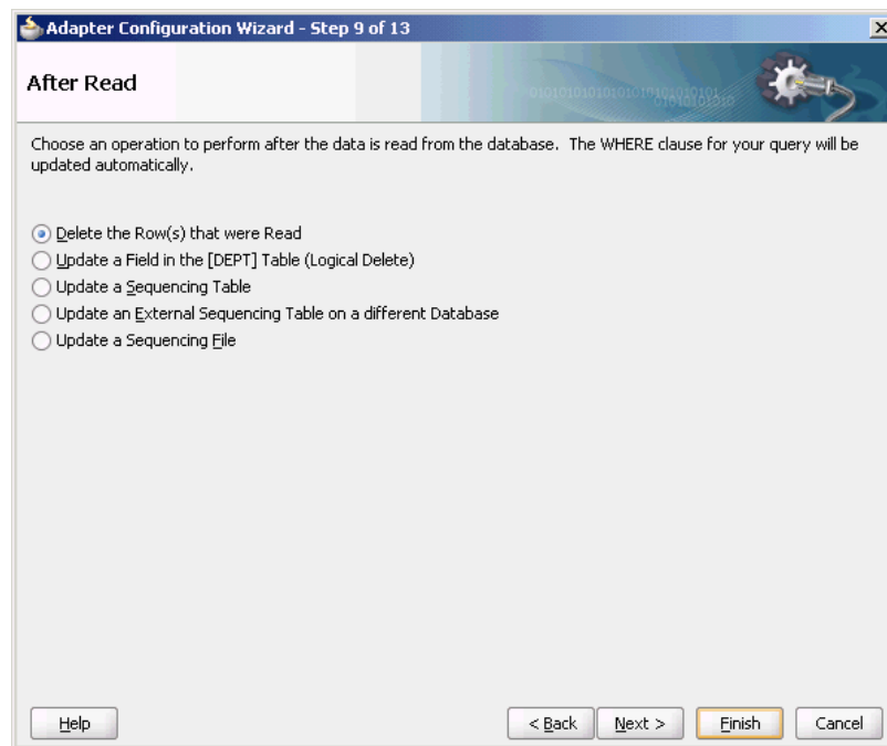
Figure 9-9 Polling Operations
