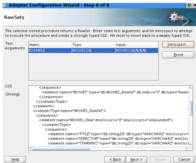
Figure 9-53 RowSets Page
