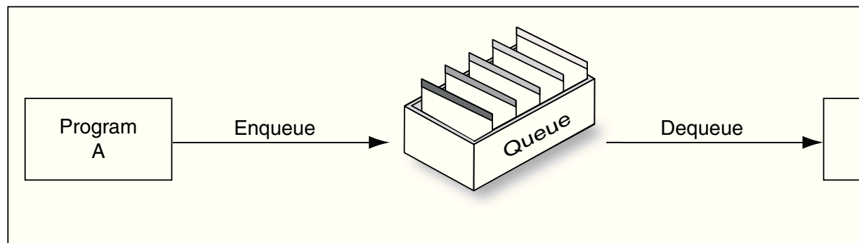
Figure 10-1 Enqueue/Dequeue
