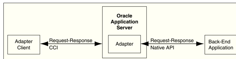
Figure 1-16 Request-Response Service
