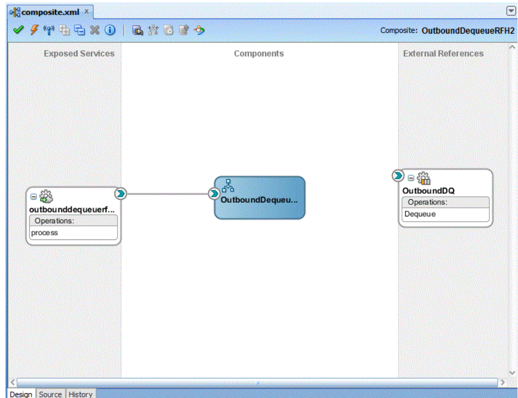
Figure 10-103 The JDeveloper-composite.xml
