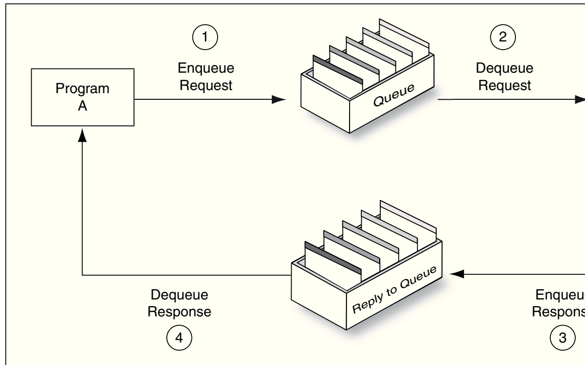
Figure 10-2 Request/Response Interaction
