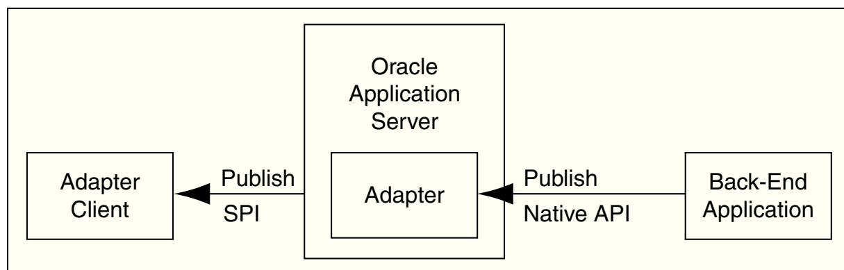
Figure 1-17 Event-Notification Service
