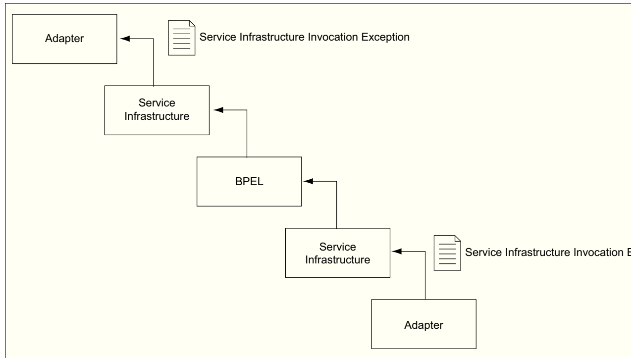
Figure 2-13 Fault Propagation
