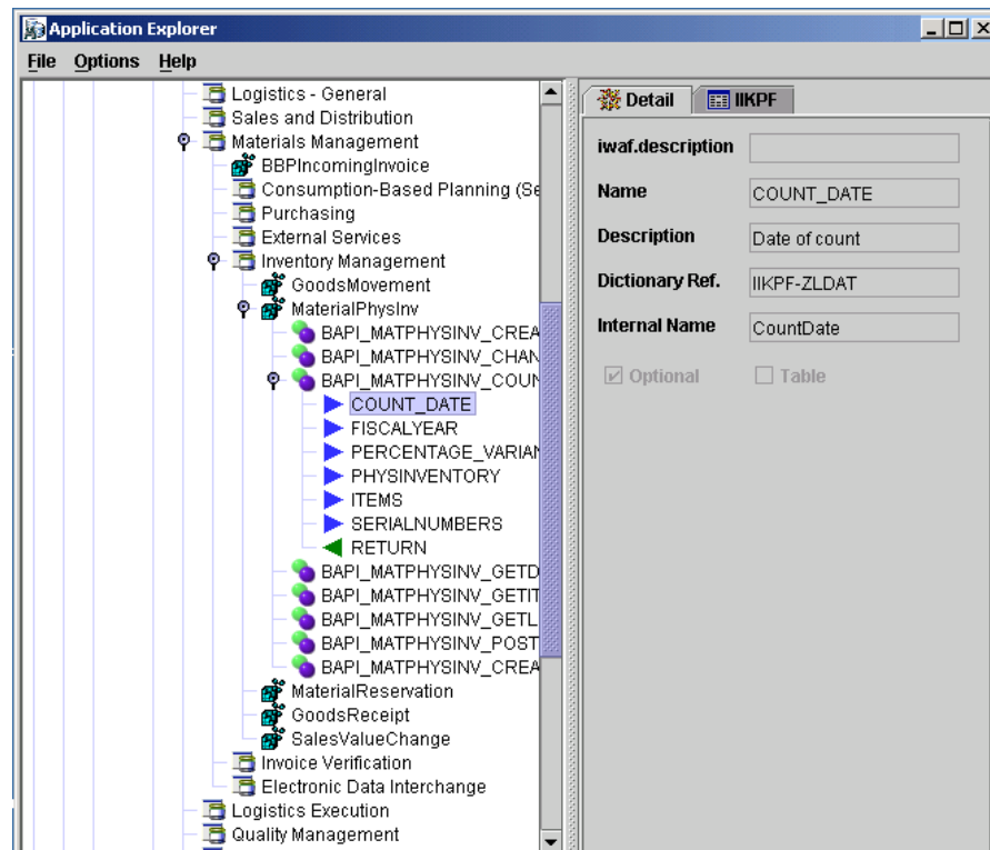
Figure 1-12 Application Explorer
