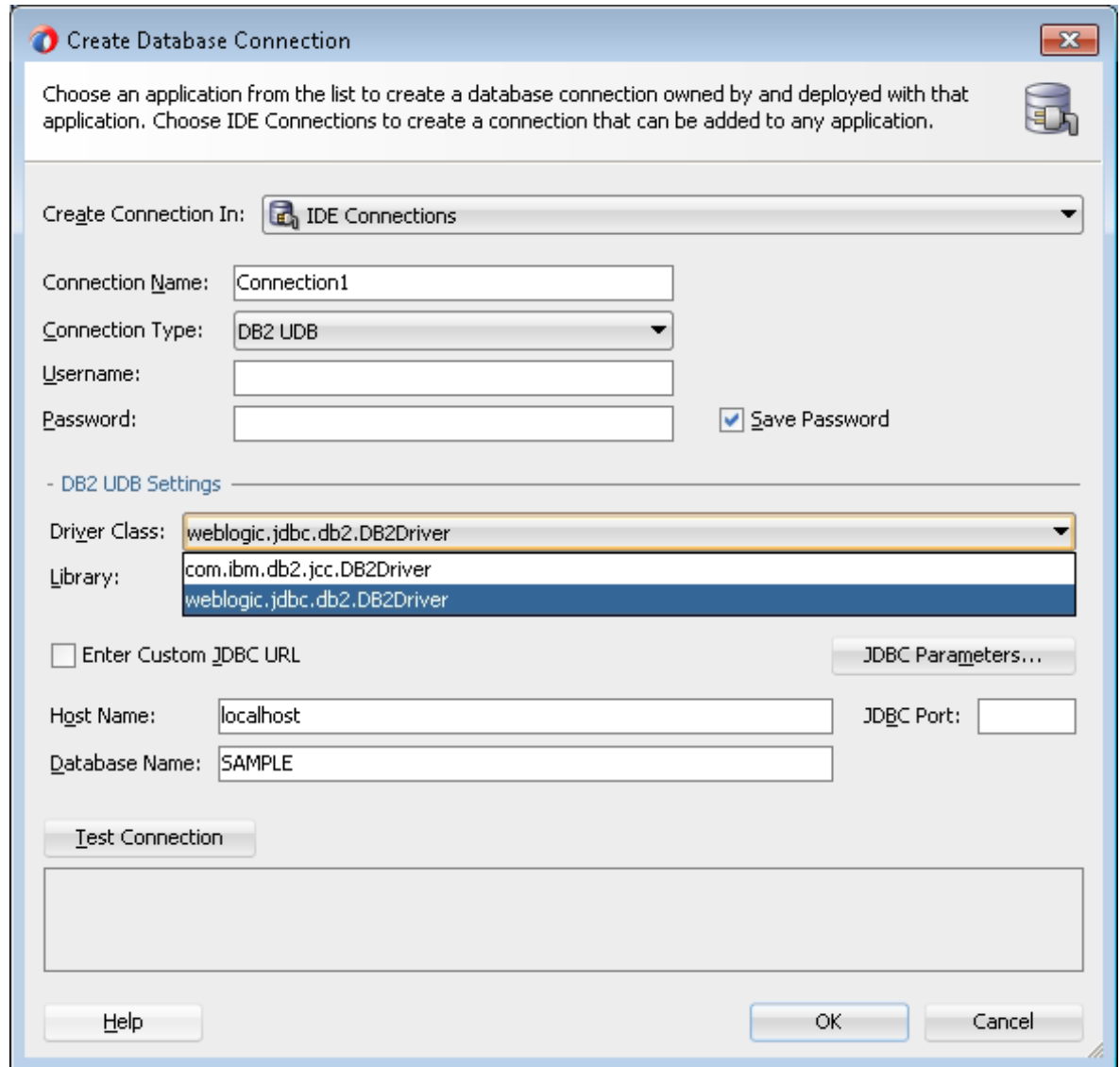
Figure 25-3 Drivers Available
