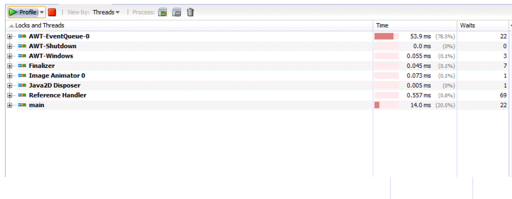
Figure 10-6 Locks Session
