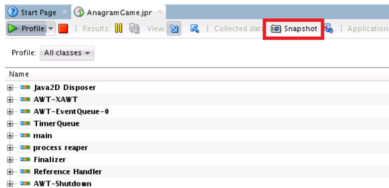
Figure 10-9 Snapshot Icon
