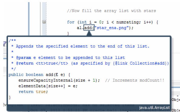
Figure 7-1 Code Peek
