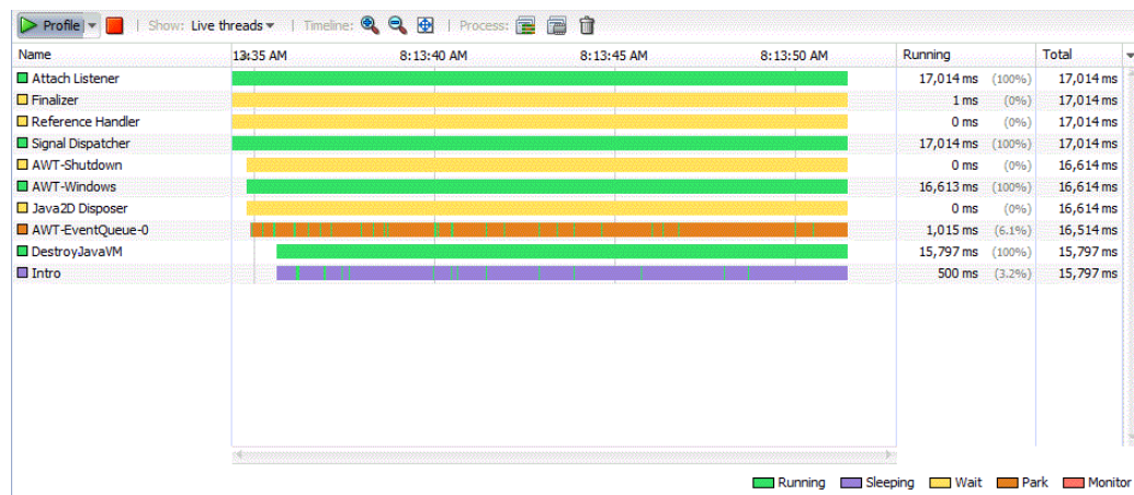
Figure 10-5 Threads Session
