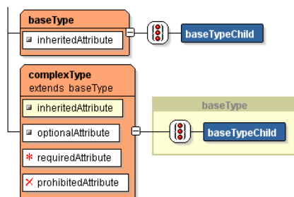
Figure 20-8 complexType Component
