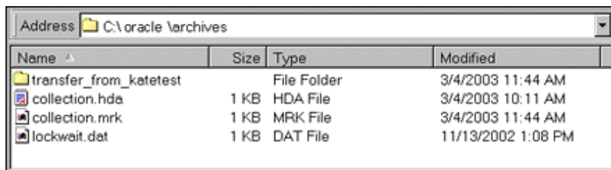
Figure 26-3 Collection Structure
