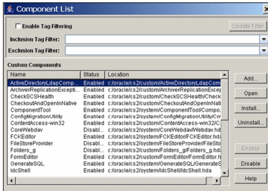
Figure 9-1 Components List
