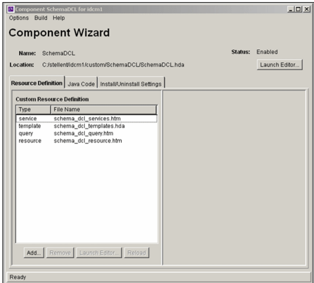
Figure 9-2 Component Wizard
