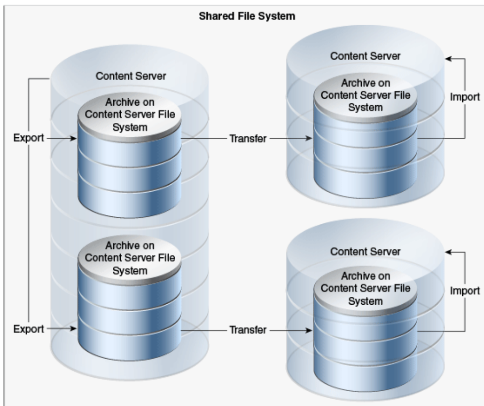
Figure 35-13 One-to-Many Archiving: On Shared File System
