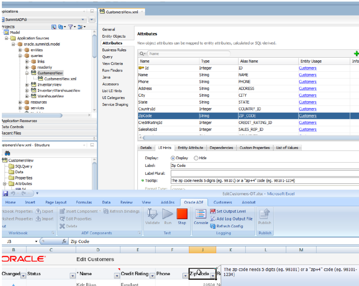
Figure 10-13 Attribute Control Hint Tooltip that Renders Tooltip in ADF Table Column Header
