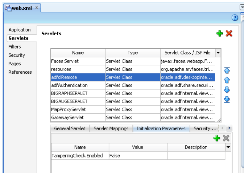
Figure 17-7 Disabling the Metadata Tamper Check In JDeveloper
