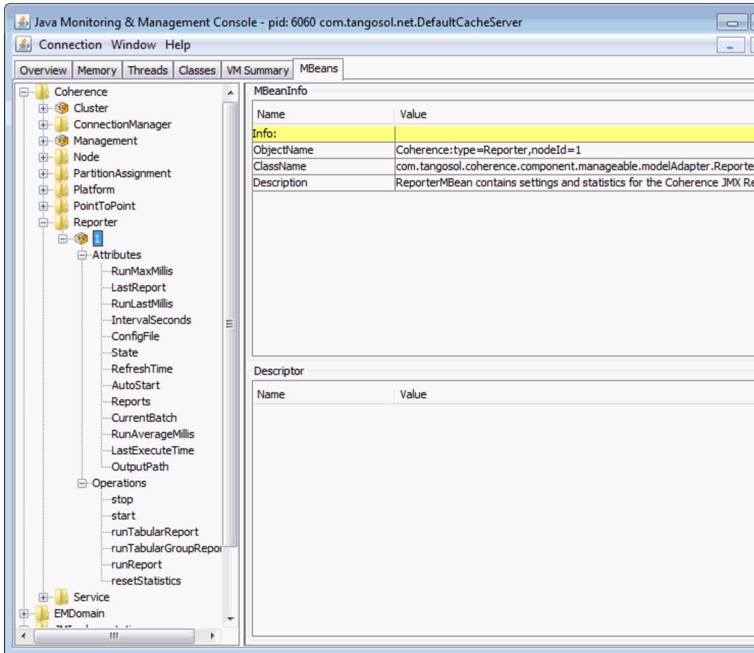
Figure 4-1 ReporterMBean MBean in JConsole
