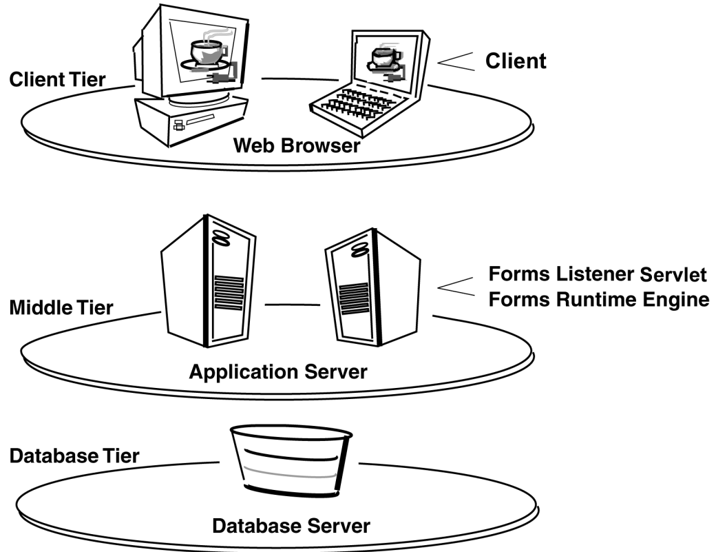
Figure 15-2 Oracle Forms Web Architecture
