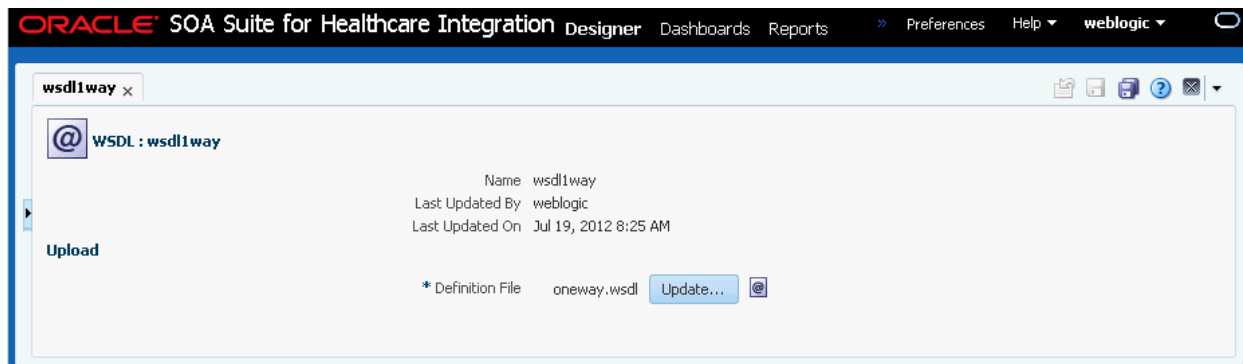
Figure 15-1 Uploaded WSDL
