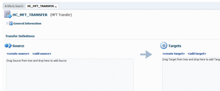
Figure 4-26 MFT Transfer Page
