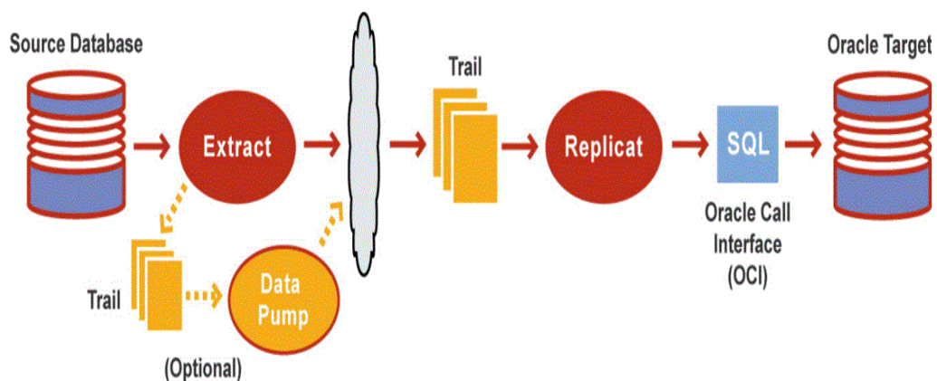
Figure 24–2 Nonintegrated Replicat Configuration
