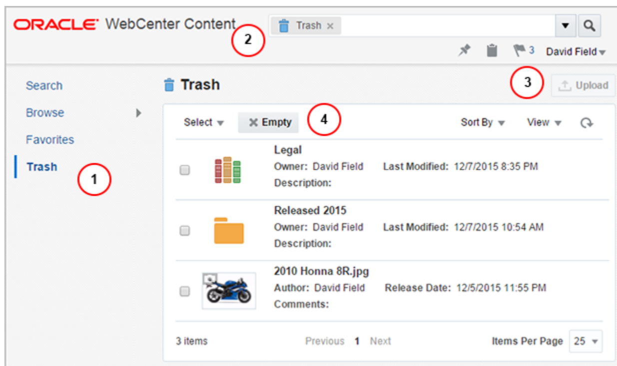
Figure 15-2 Trash Page
