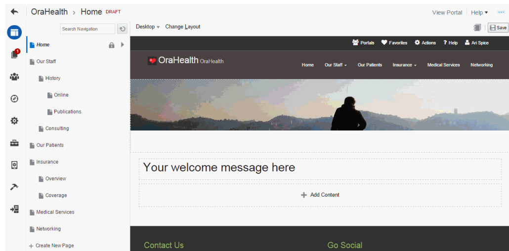
Figure 8-17 Portal Editor
