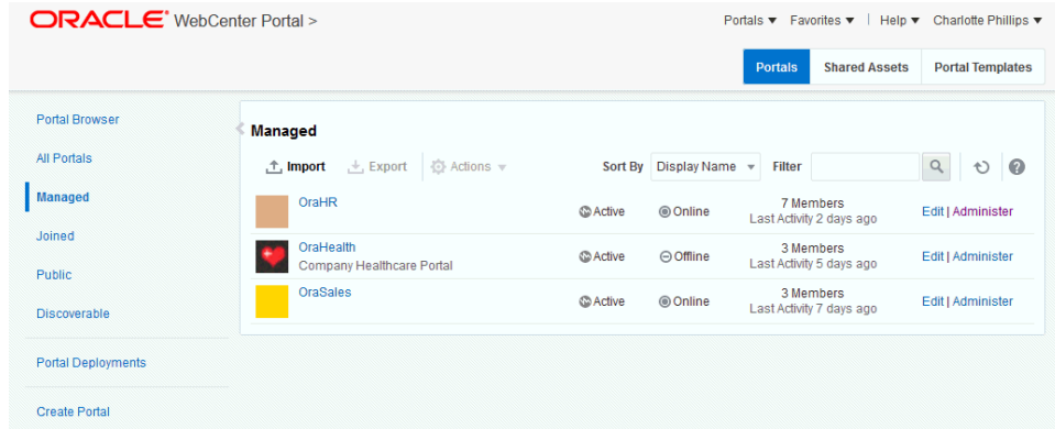
Figure 6-47 Managed Portals
