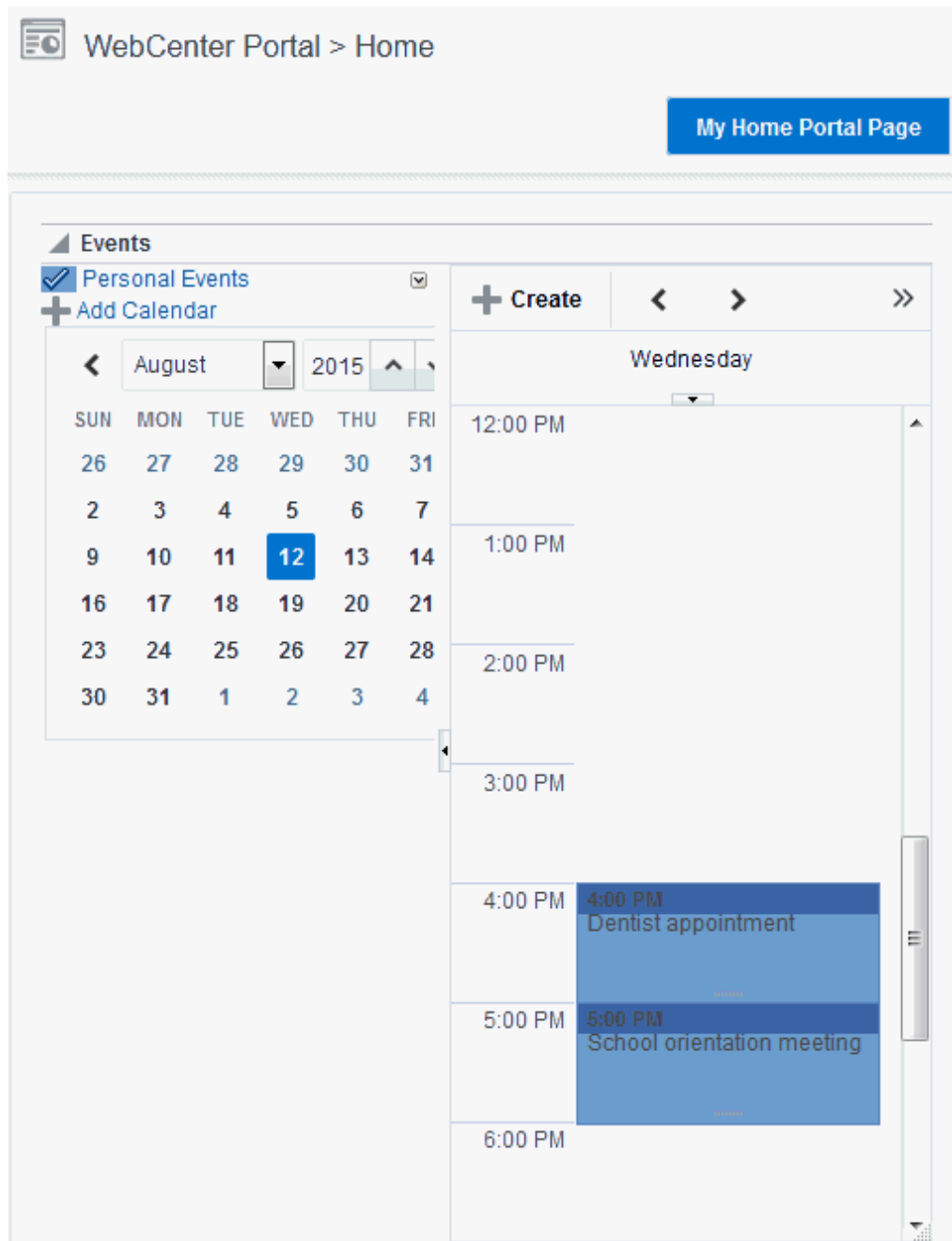
Figure 46-8 Personal Calendar
