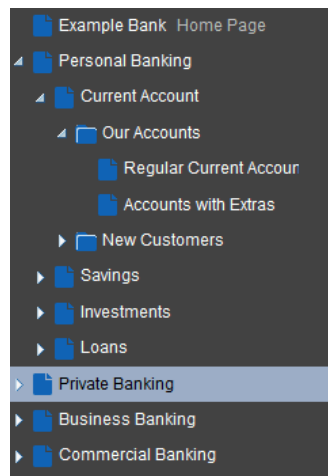
Figure 16-13 Sample Navigation
