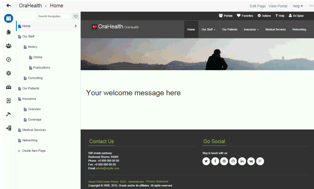
Figure 5-5 Portal Editor
