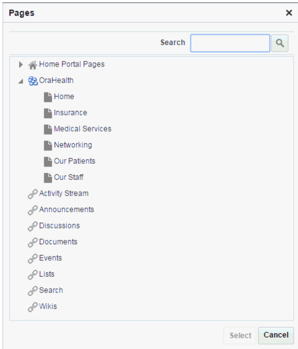
Figure 5-7 Pages Dialog
