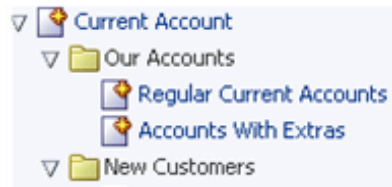
Figure 16-21 Show Icons
