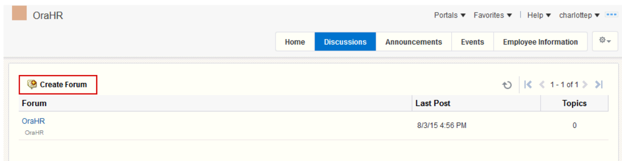
Figure 48-21 Create Forum
