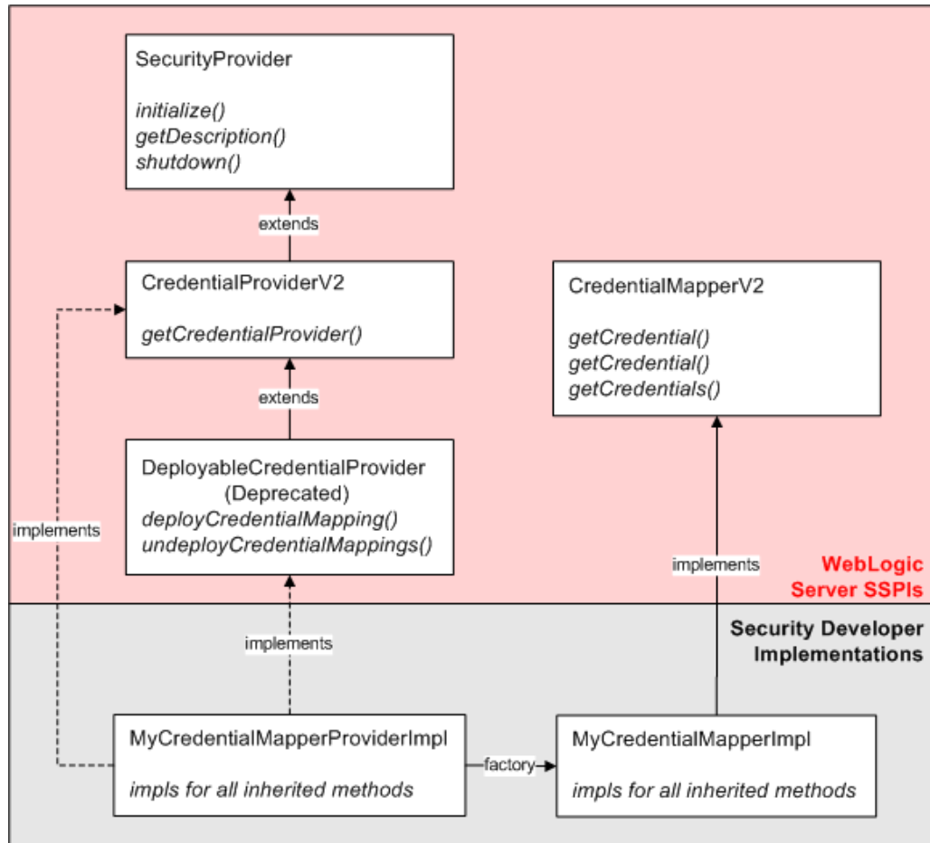
Figure 3-4 Credential Mapping SSPIs and Two Runtime Classes
