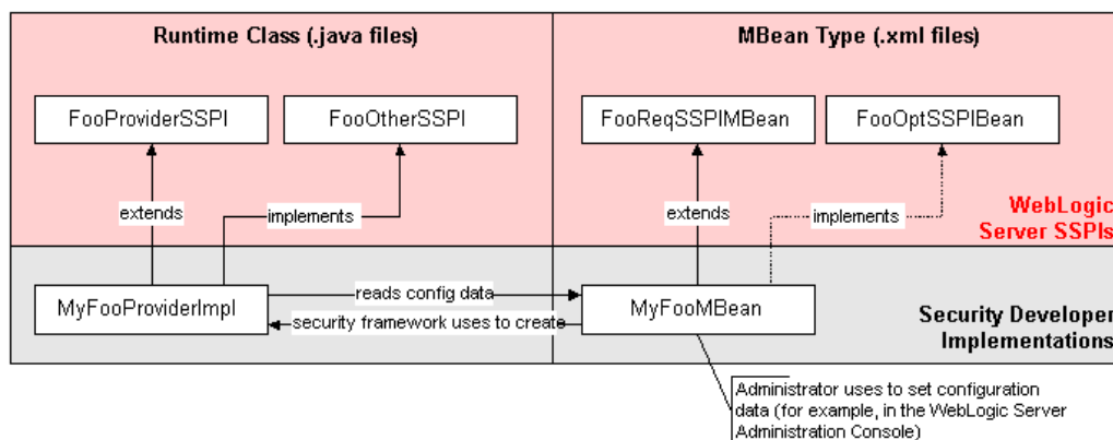
Figure 3-1 Security Provider Architecture
