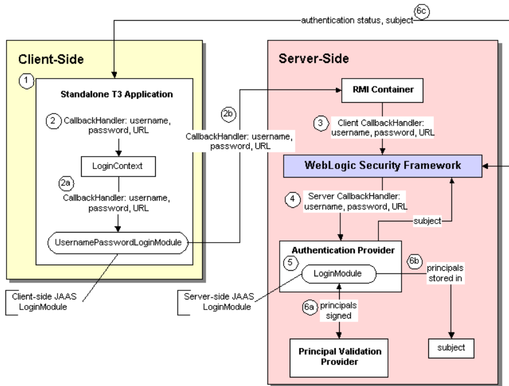
Figure 4-3 Authentication Using JAAS Classes and WebLogic Server
