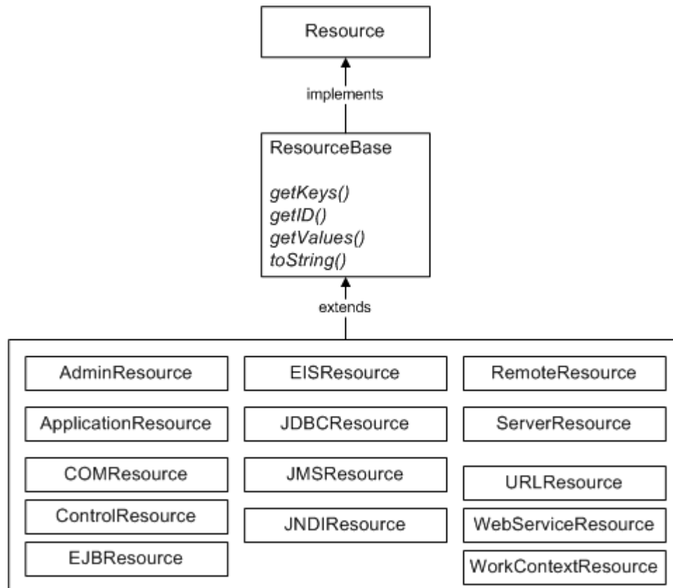
Figure 3-10 Architecture of WebLogic Resources
