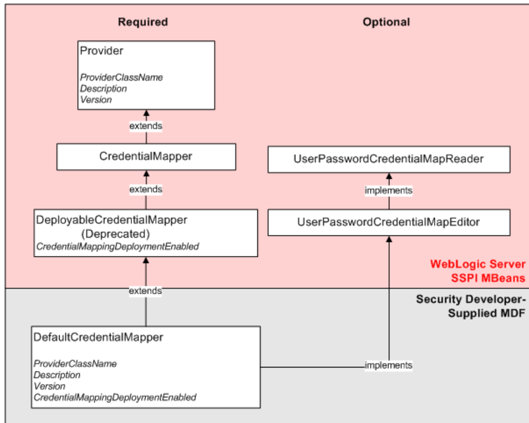
Figure 3-5 SSPI MBean Hierarchy for Credential Mapping Providers
