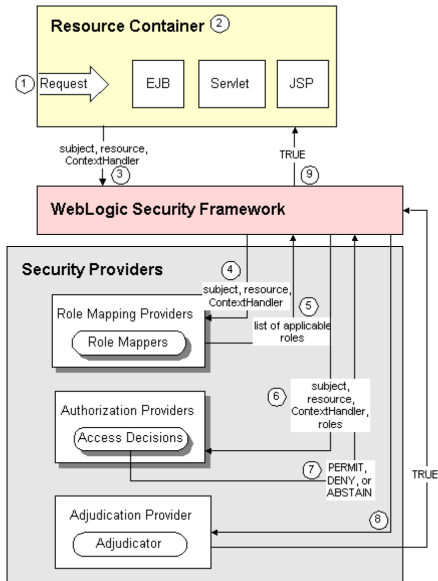
Figure 7-1 Authorization Providers and the Authorization Process
