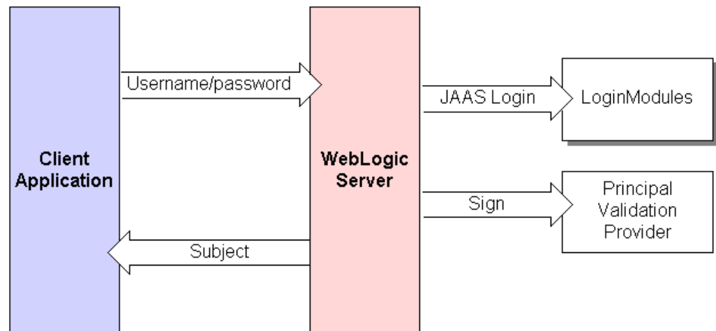
Figure 4-4 The Authentication Process
