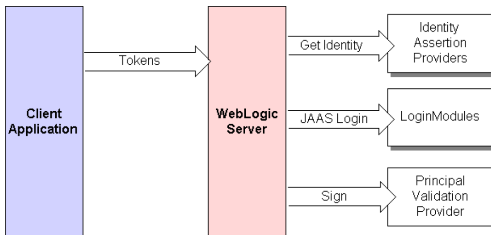
Figure 5-2 Perimeter Authentication
