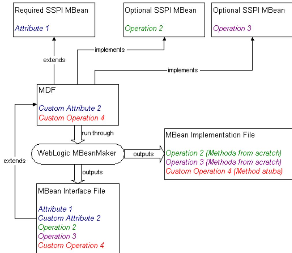
Figure 3-7 What the WebLogic MBeanMaker Provides
