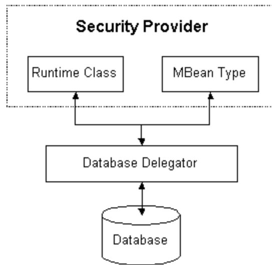
Figure 3-11 Positioning of the Database Delegator Class
