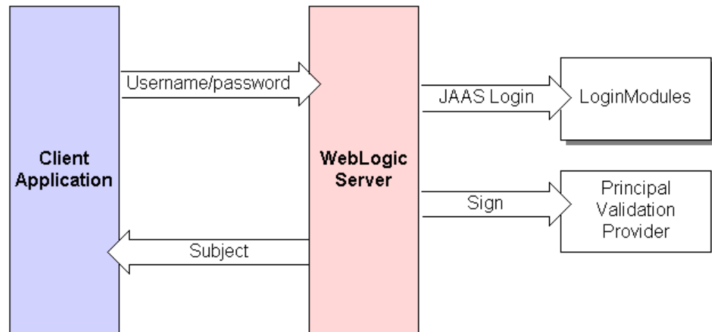
Figure 6-1 The Principal Validation Process
