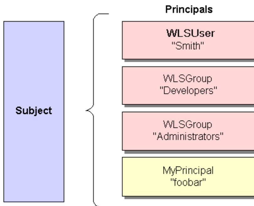
Figure 4-1 Relationships Among Users, Groups, Principals and Subjects
