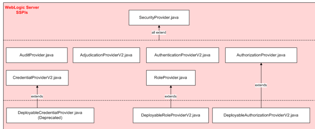
Figure 3-2 "Provider" SSPIs
