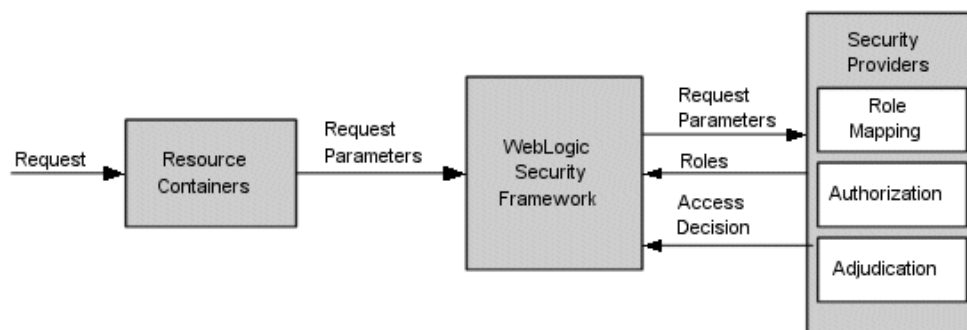
Figure 5-5 Authorization Process
