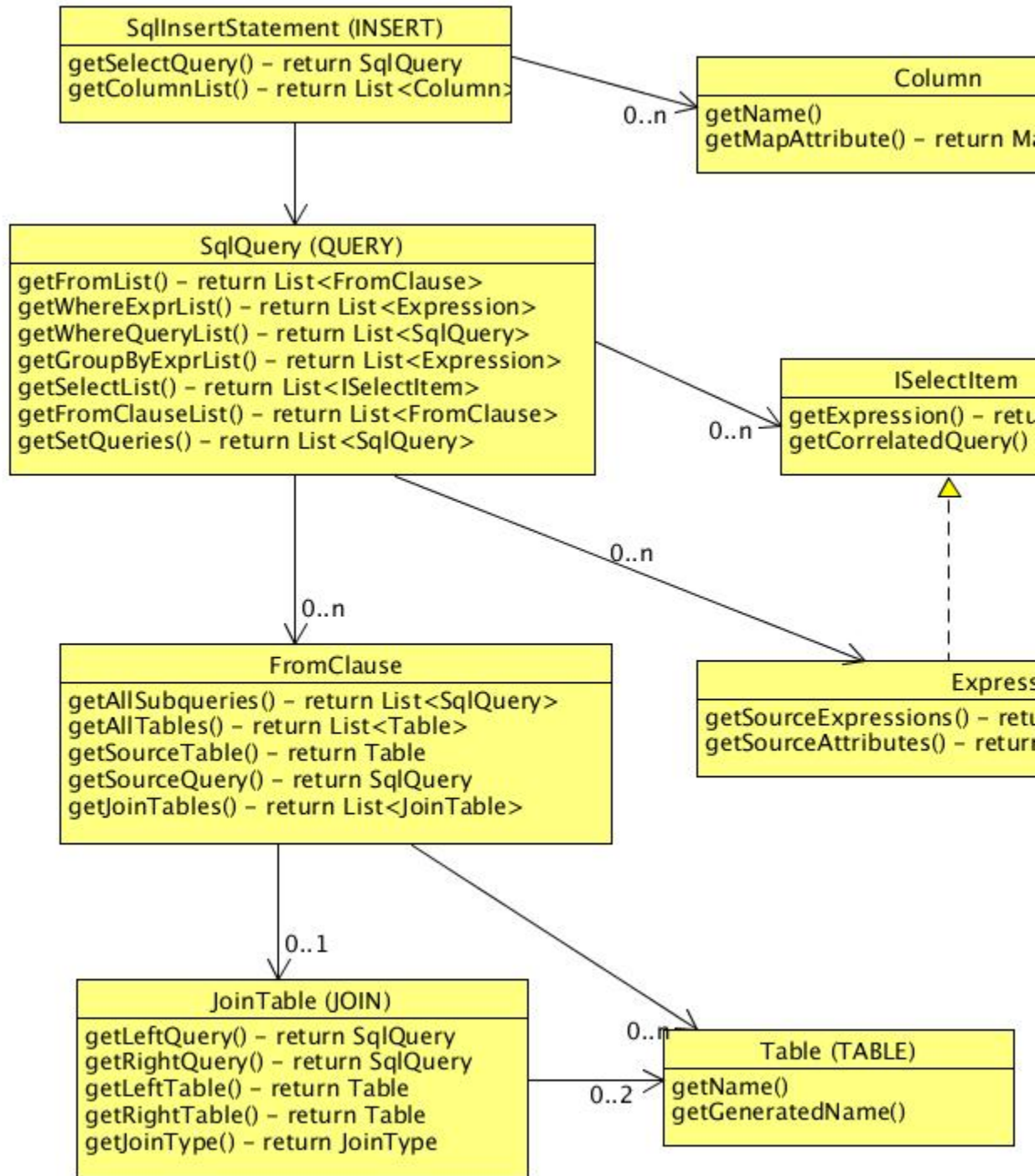
Figure 3-1 Structured Substitution API
