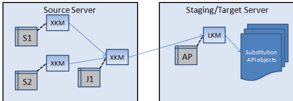
Figure 1-7 Extract Knowledge Modules (XKM)
