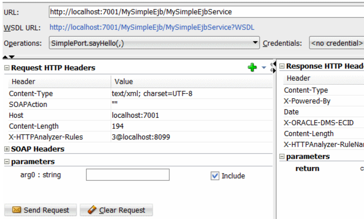
Figure 14-3 HTTP Analyzer Test Window
