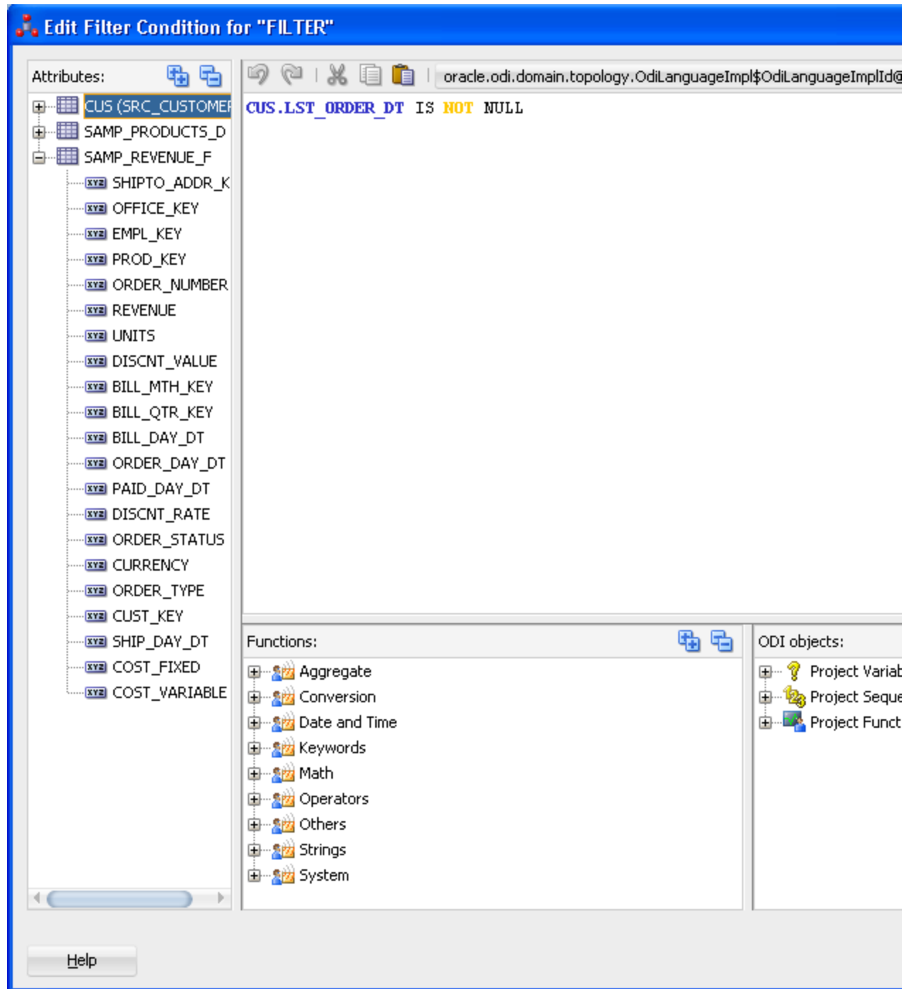
Figure 8-2 Example Expression Editor
