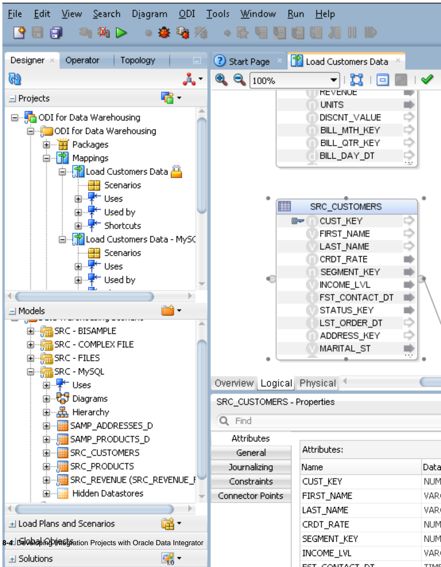
Figure 8-1 Mapping Editor
