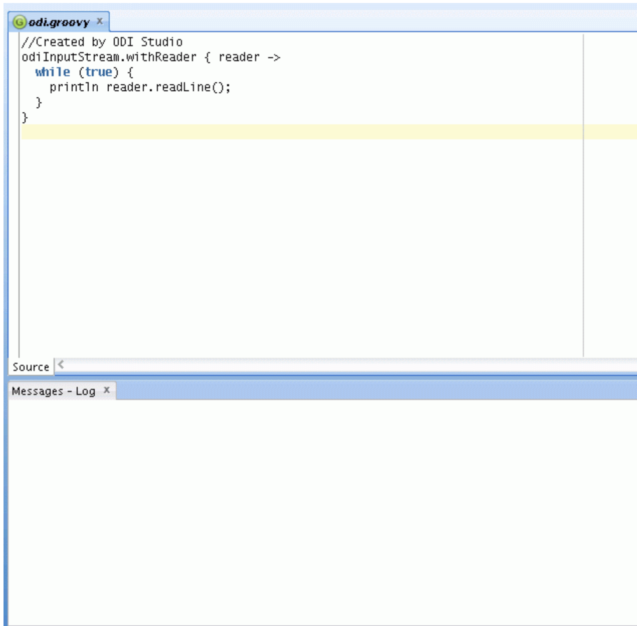
Figure 16-1 Groovy Editor
