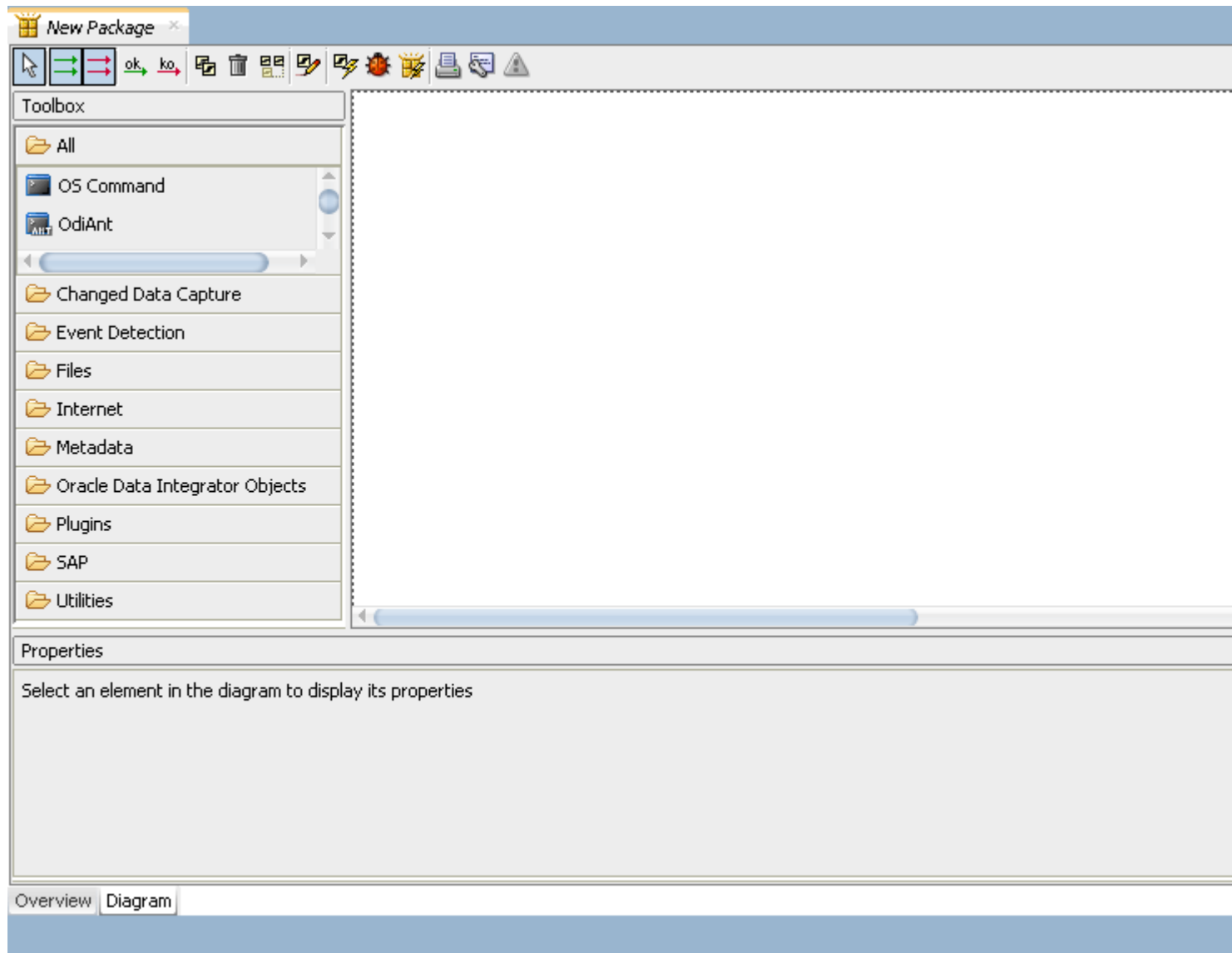
Figure 7-2 Package editor
