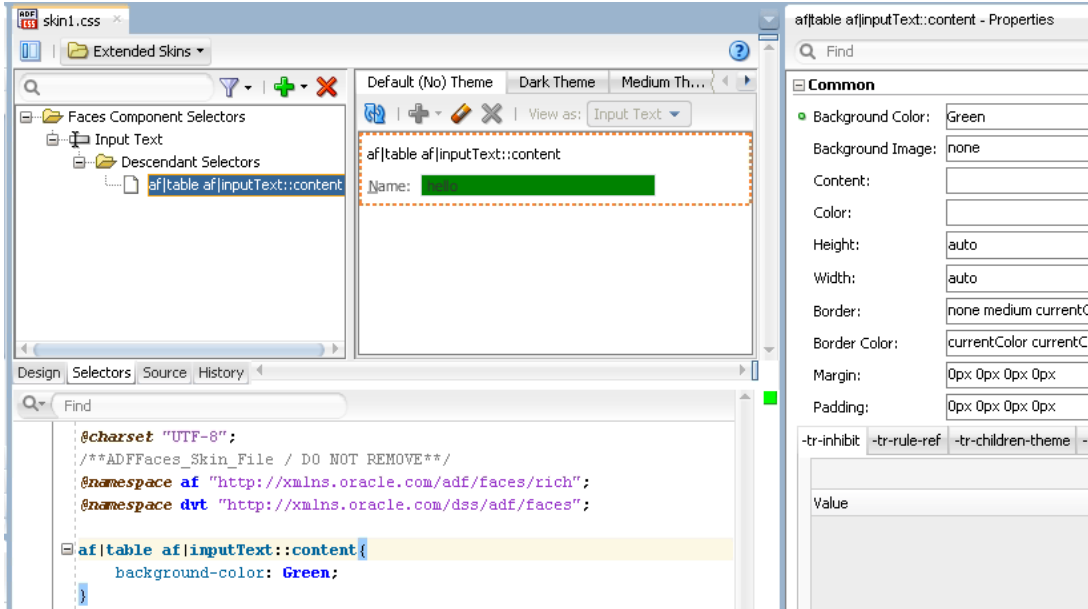
Figure 3-8 Descendant Selectors in the Selector Tree
