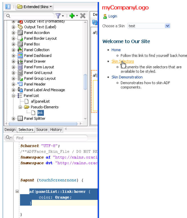
Figure 3-9 Pseudo-Class Syntax and Runtime Behavior for a Panel List Link
