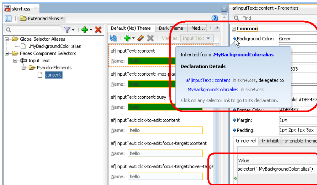
Figure 9-8 Global Selector Alias Applied to inputText Component
