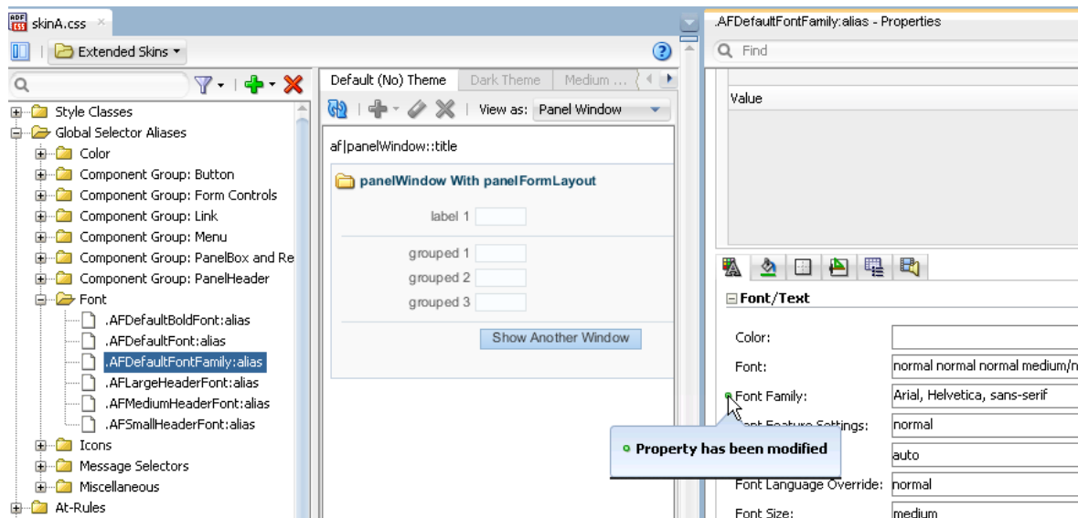
Figure 9-2 ADF Skin Changing a Global Selector Alias
