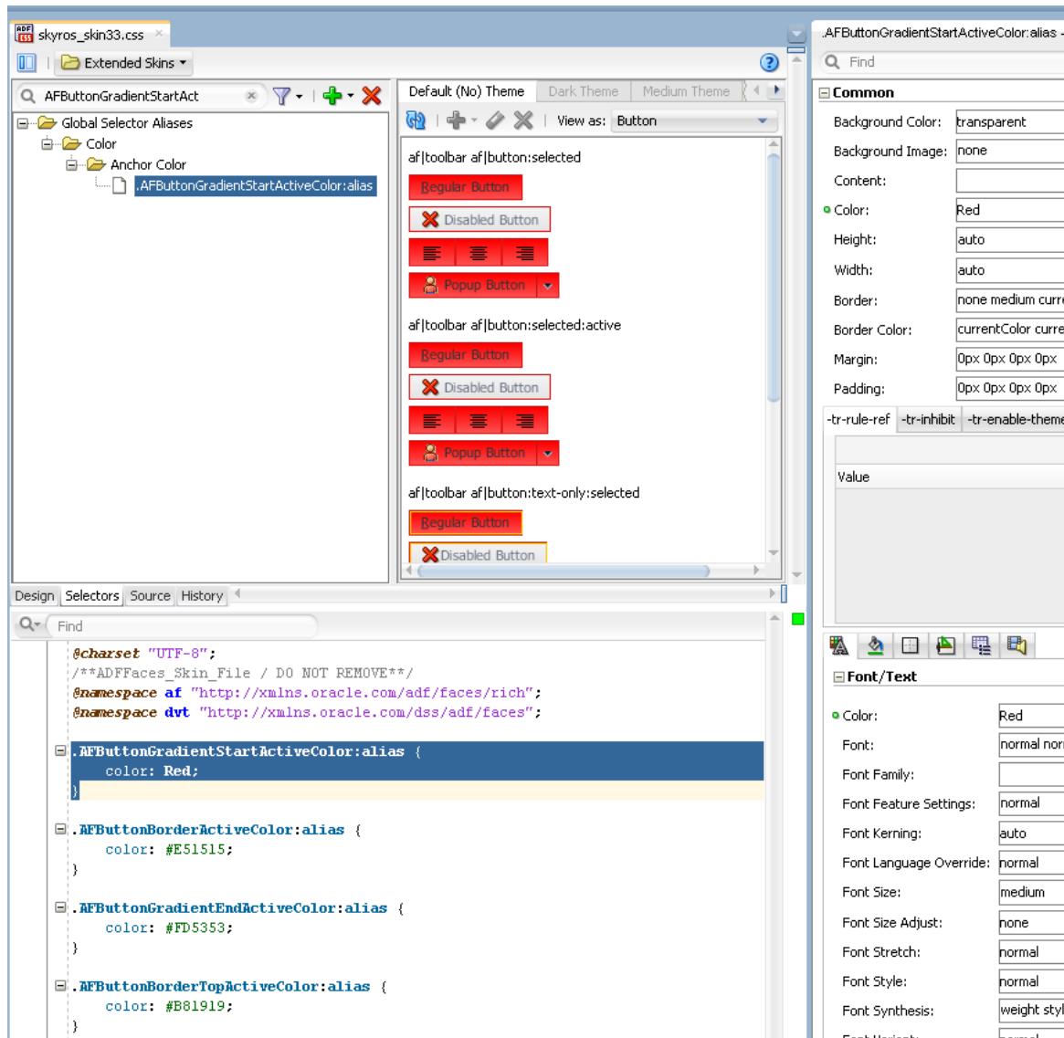
Figure 7-4 Modified Anchor Color and Effect on Derivative Colors
