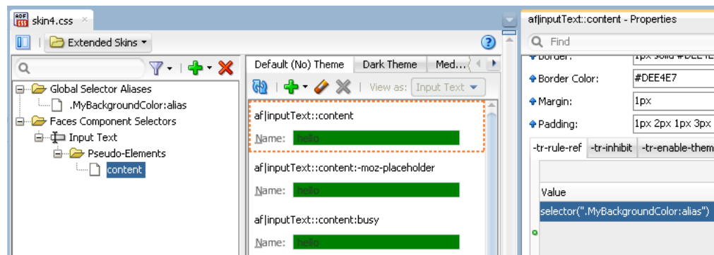
Figure 9-7 inputText Component's content Pseudo-Element
