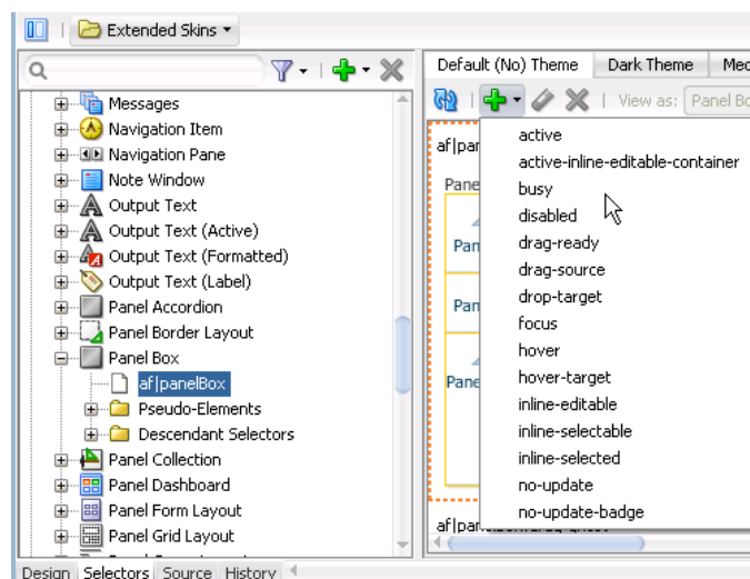
Figure 3-10 Pseudo-classes for the panelBox Component's Selector
