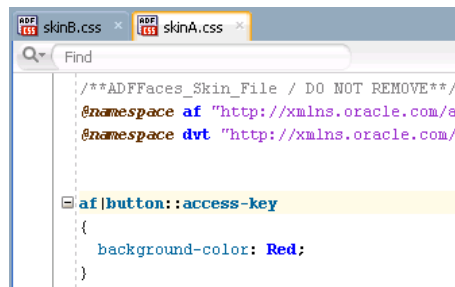
Figure 4-14 Property Value Defined in Extended ADF Skin
