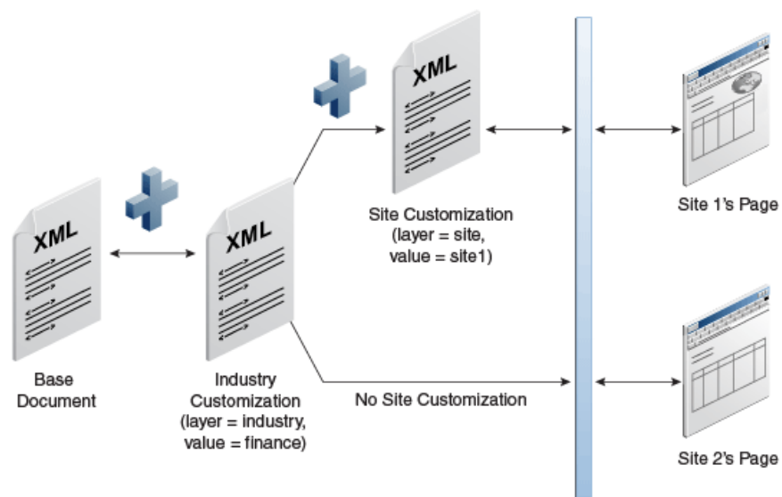
Figure 9-2 Base Application and Customization Layers
