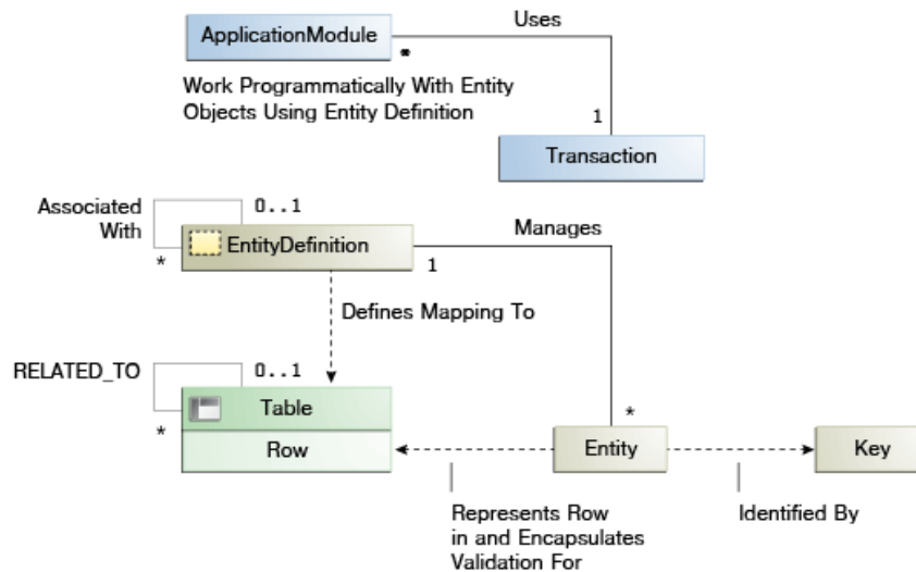
Figure 4-5 Entity Object Within the ADF Business Component Architecture
