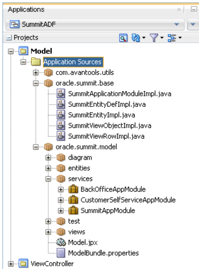
Figure 2-7 Applications Window with Model Project
