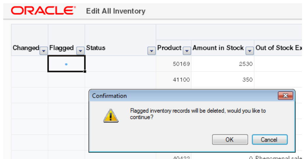
Figure 9-16 Confirmation Dialog
