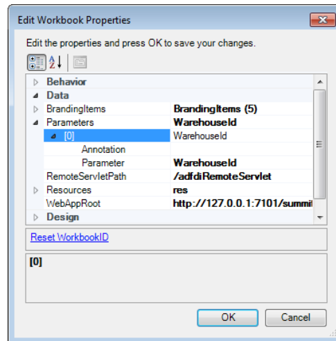
Figure 15-5 Workbook Parameters
