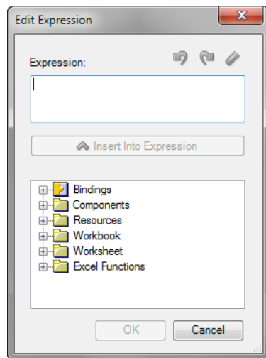
Figure 5-10 Expression Builder
