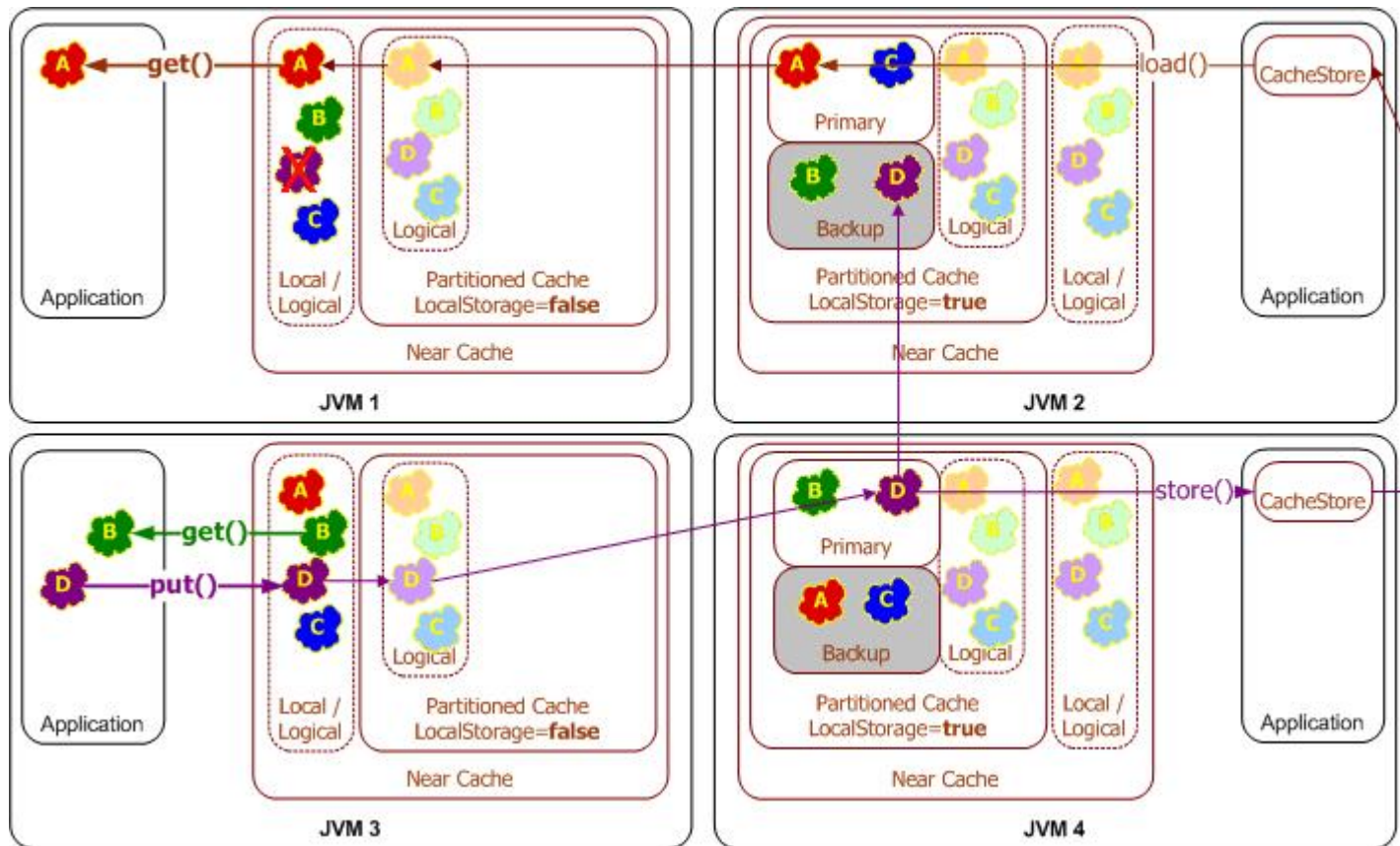
Figure 14-2 Write-Through Caching
