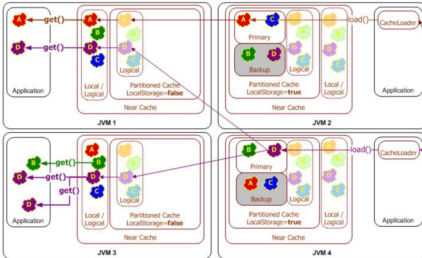
Figure 14-1 Read-Through Caching
