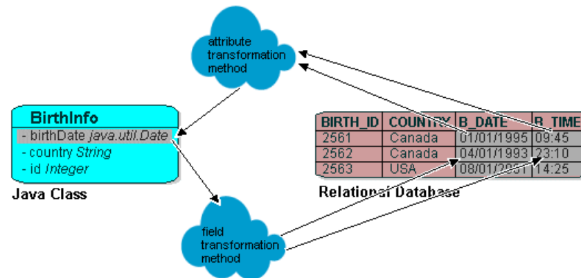
Figure 6–7 Transformation Mappings
