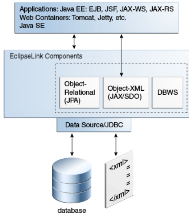
Figure 1–1 EclipseLink Components
