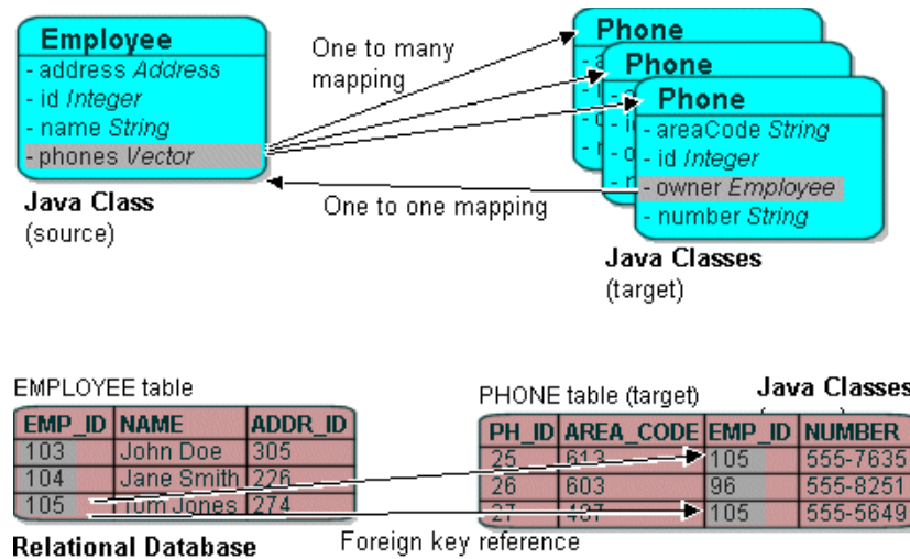
Figure 6–12 One-to-Many Relationships
