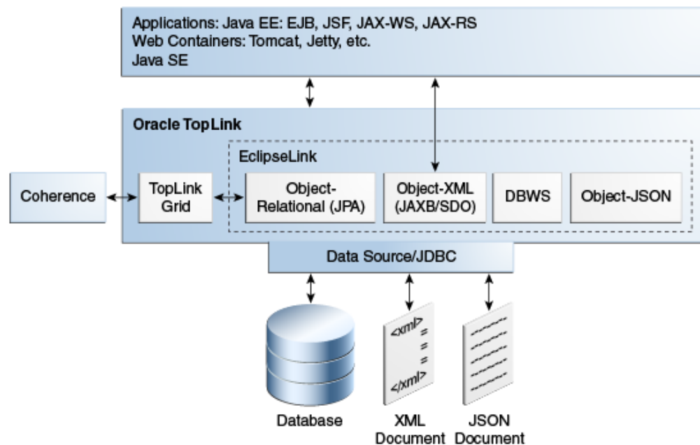
Figure 1–2 TopLink Components
