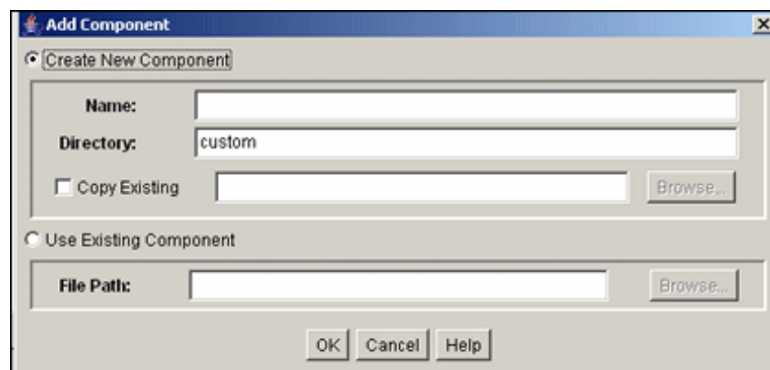
Figure 9-3 Add Component
