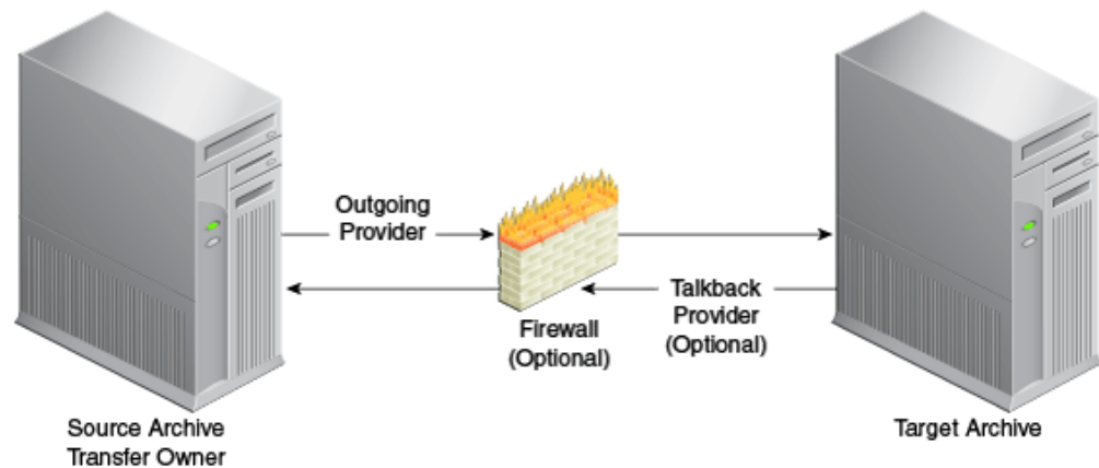
Figure 29-3 Push Transfer
