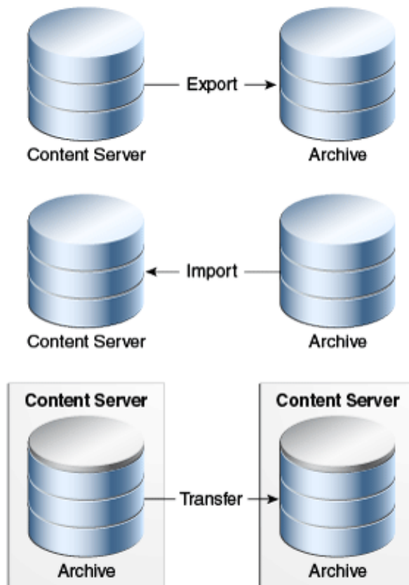
Figure 23-1 Archiver Functions
