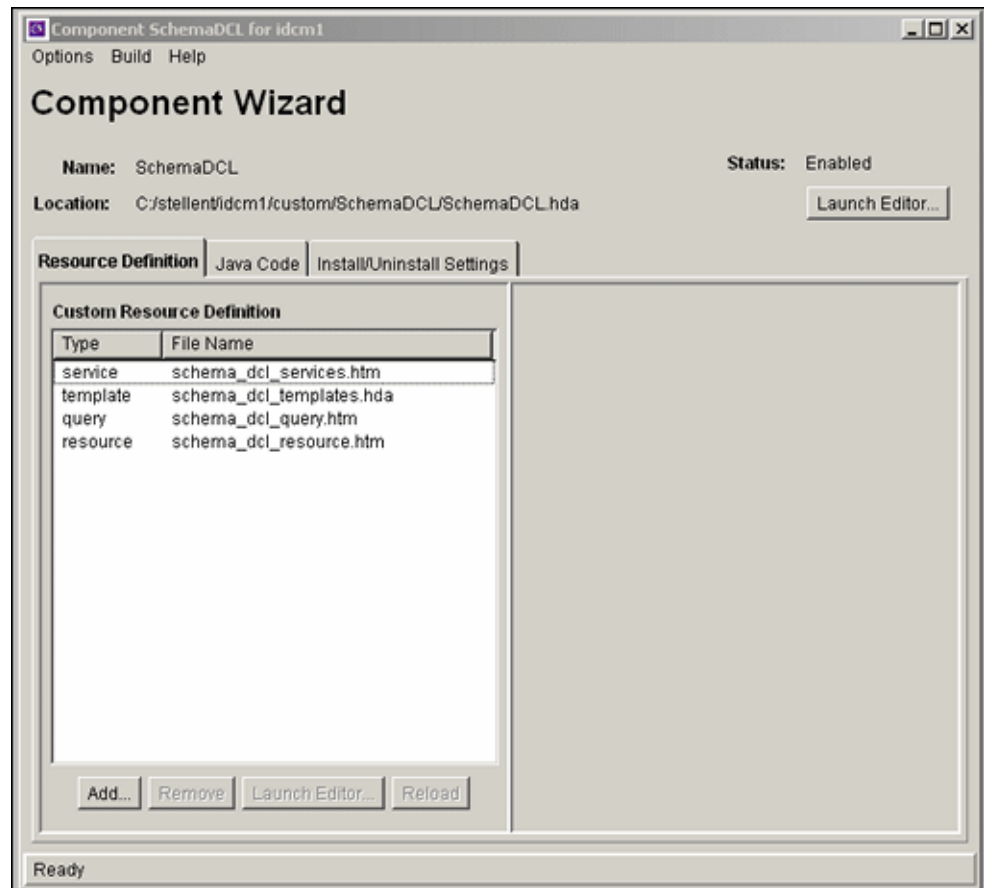
Figure 9-2 Component Wizard
