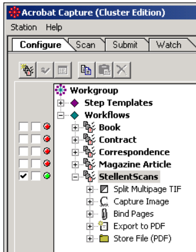
Figure C-3 Workflow Example
