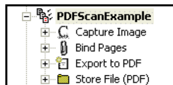
Figure C-6 Workflow Example
