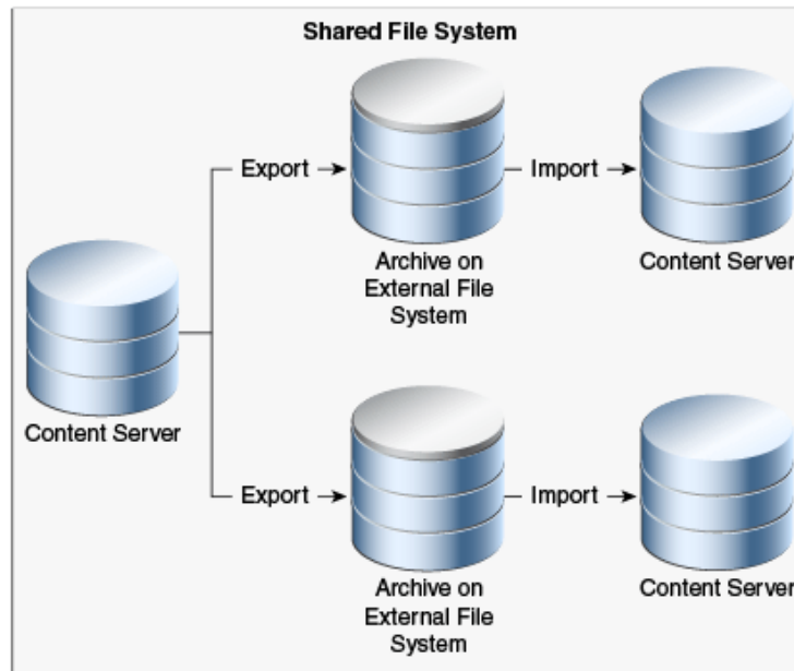
Figure 35-14 One-to-Many Archiving: On Shared External File System
