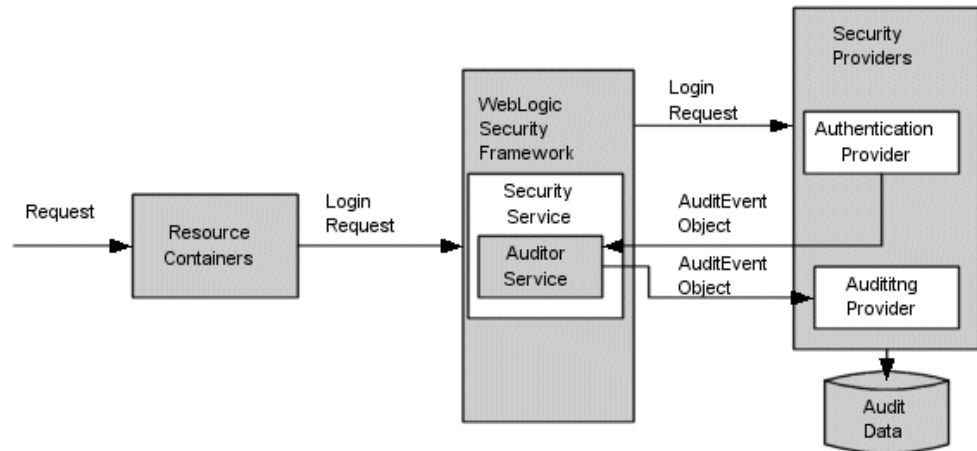
Figure 5-7 Auditing Process
