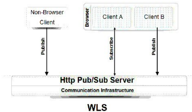
Figure 12-1 HTTP Publish-Subscribe Server of WebLogic Server
