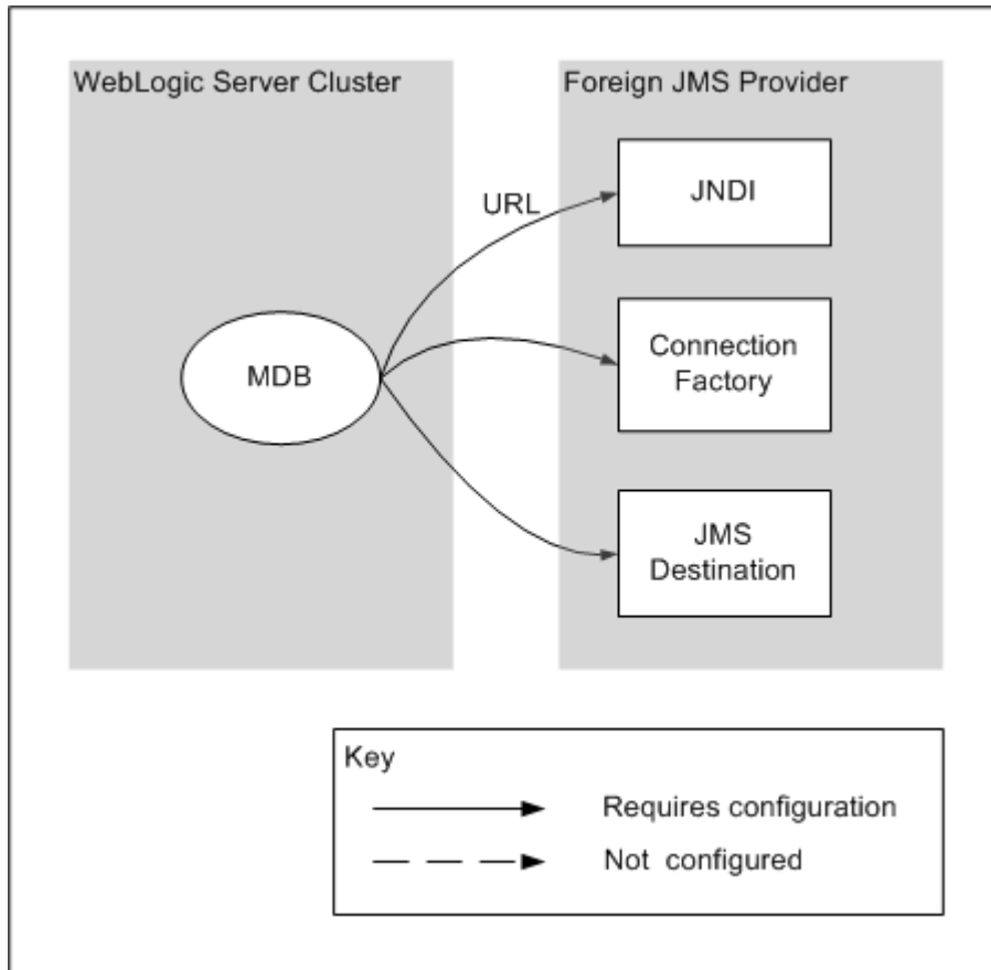
Figure 6-3 C. Destination on Foreign JMS Server—No Mappings
