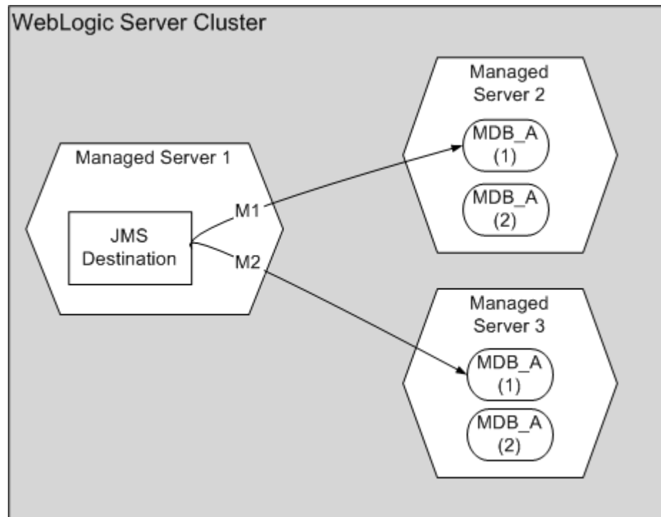
Figure 4-3 Non-Collocated Application, Non-Distributed Destination
