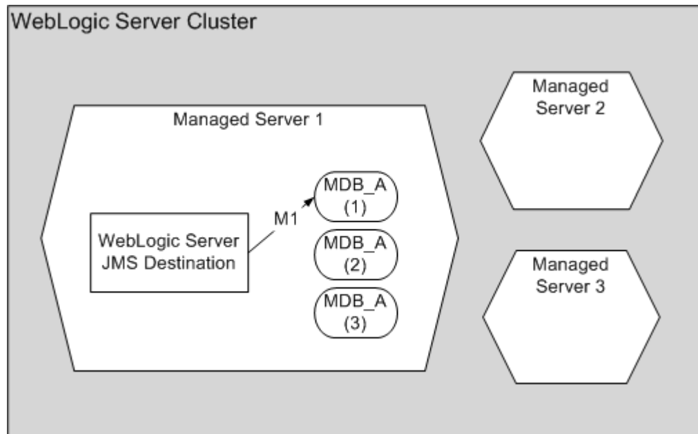
Figure 4-2 Collocated Destination/MDBs, Non-Distributed Destination
