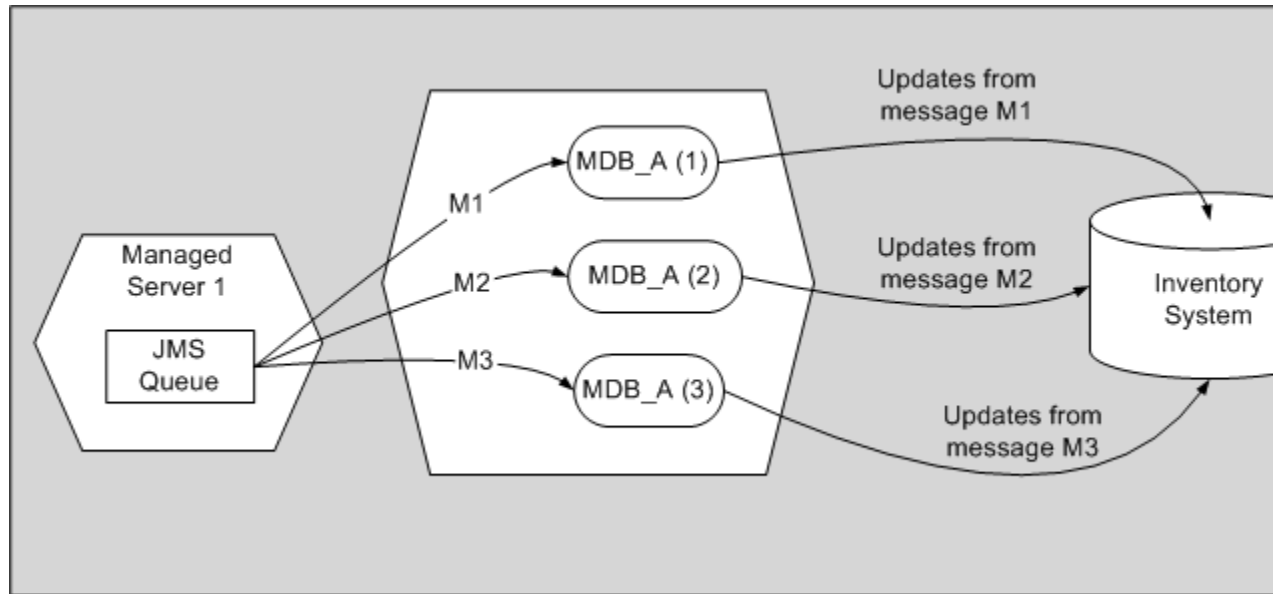
Figure 3-1 Point-to-Point Model
