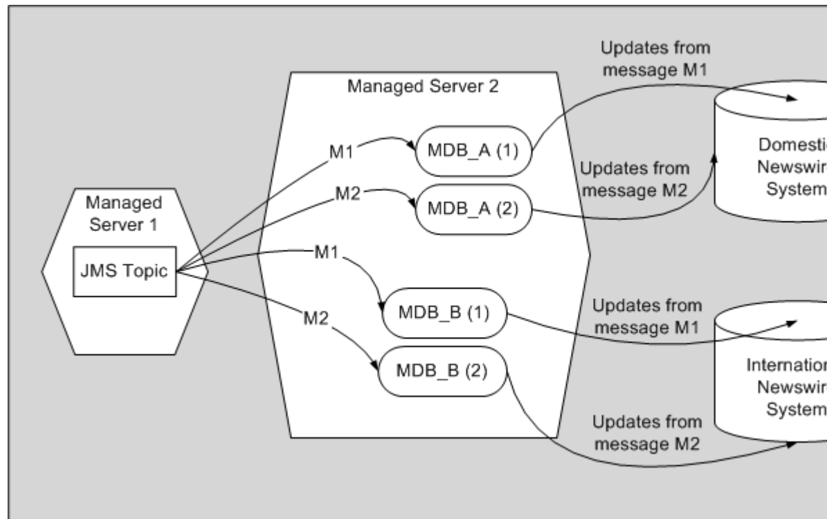
Figure 3-2 Publish/Subscribe Model
