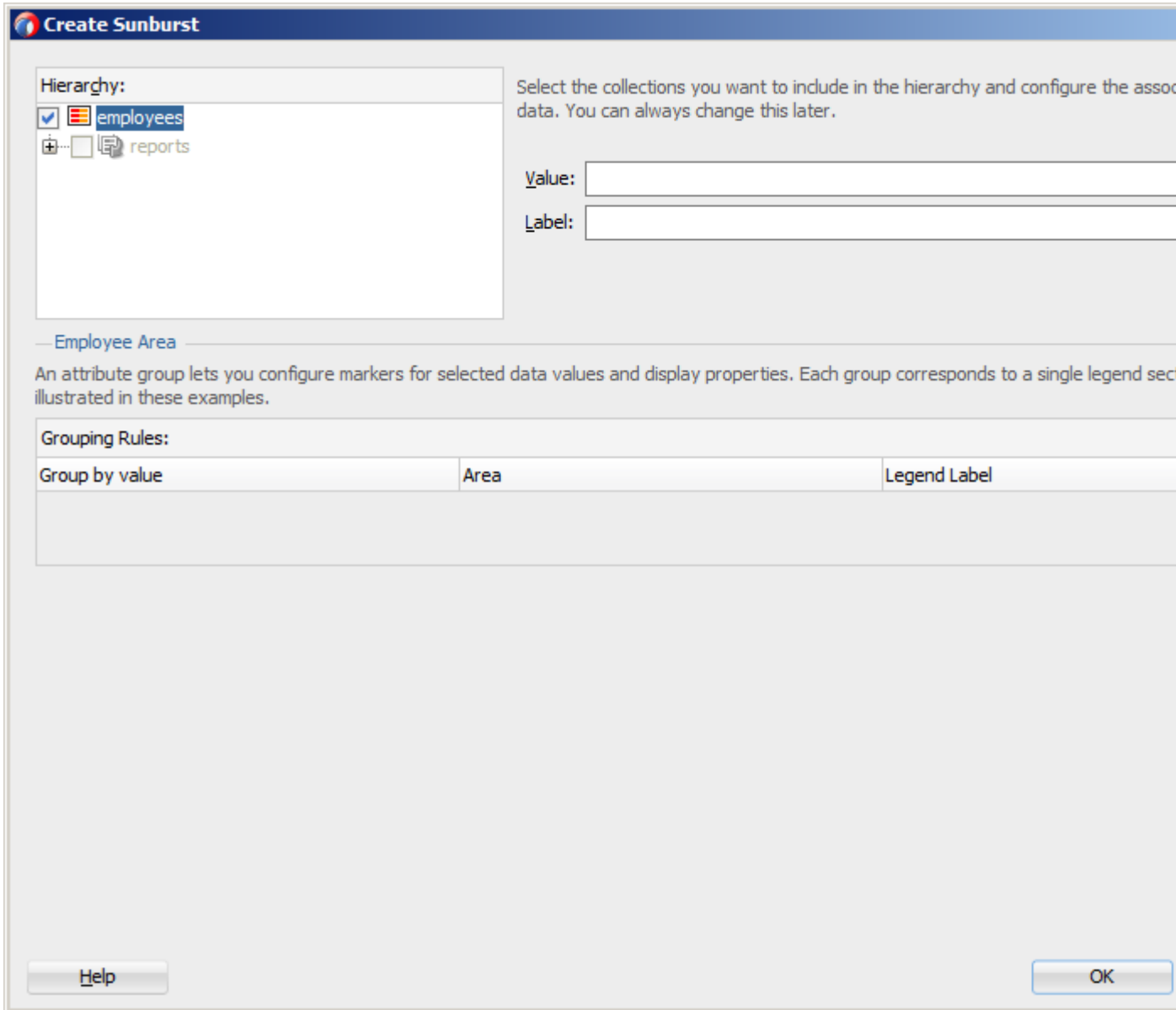
Figure 13-108 Creating Databound Sunburst
