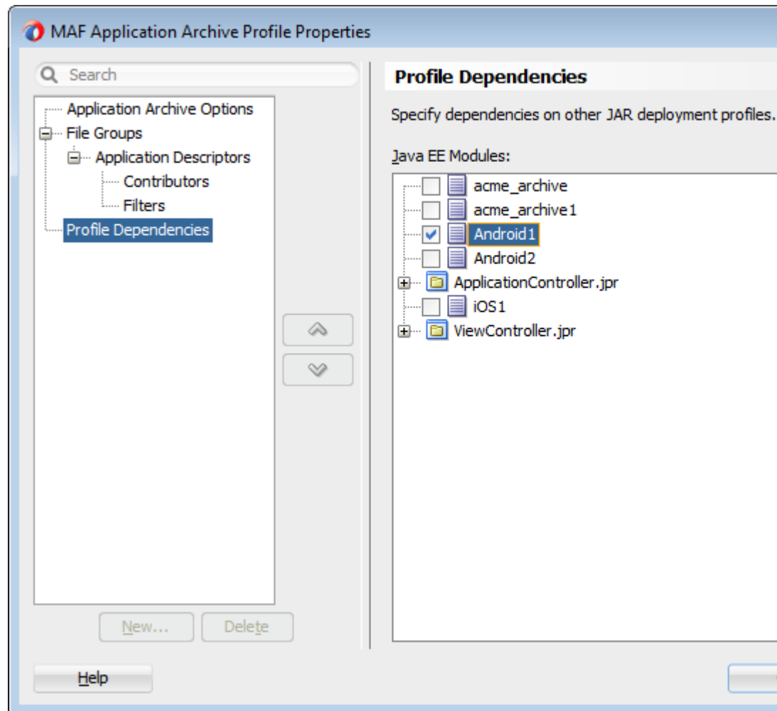
Figure 27-38 Selecting Deployment Profiles
