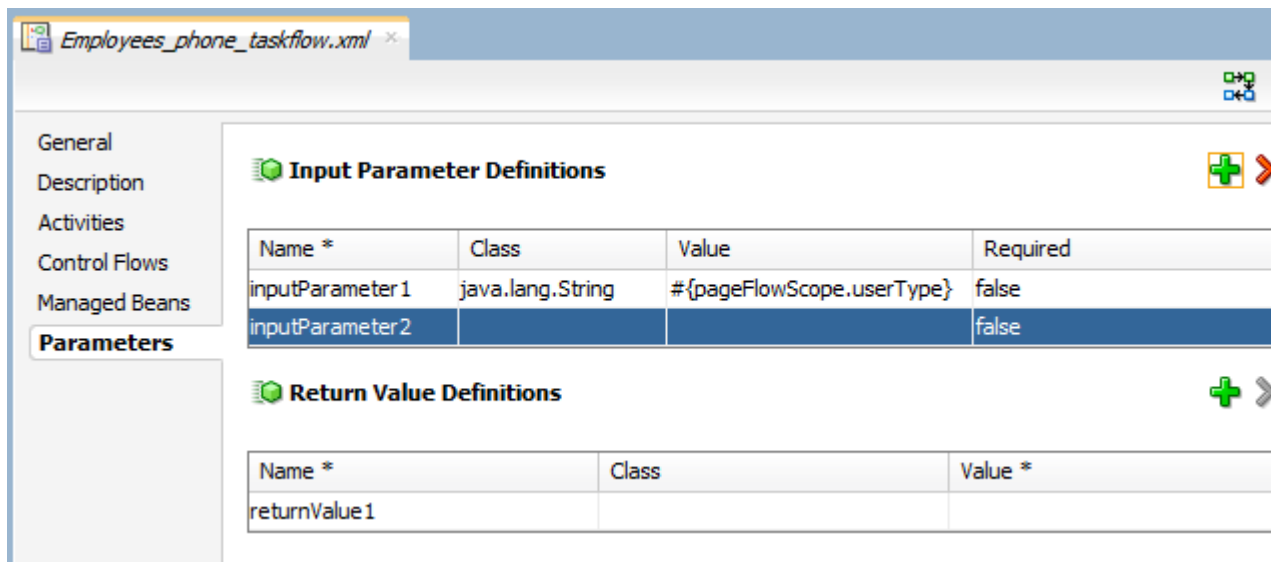
Figure 12-26 Input Parameters in Task Flow
