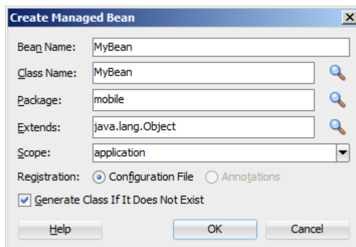
Figure 12-19 Setting Managed Bean Name and Class
