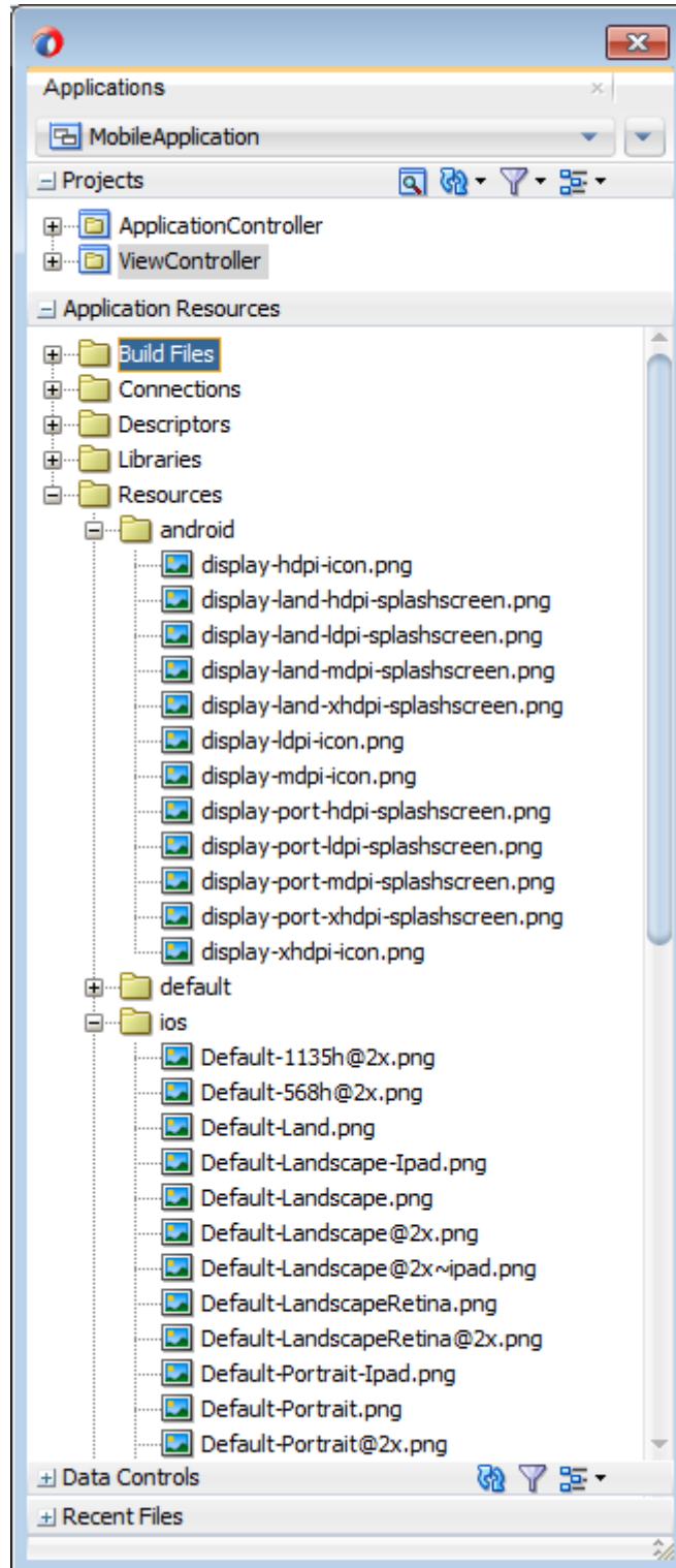
Figure C-1 MAF Application Artifacts Accessed from the Application Resources Pane
