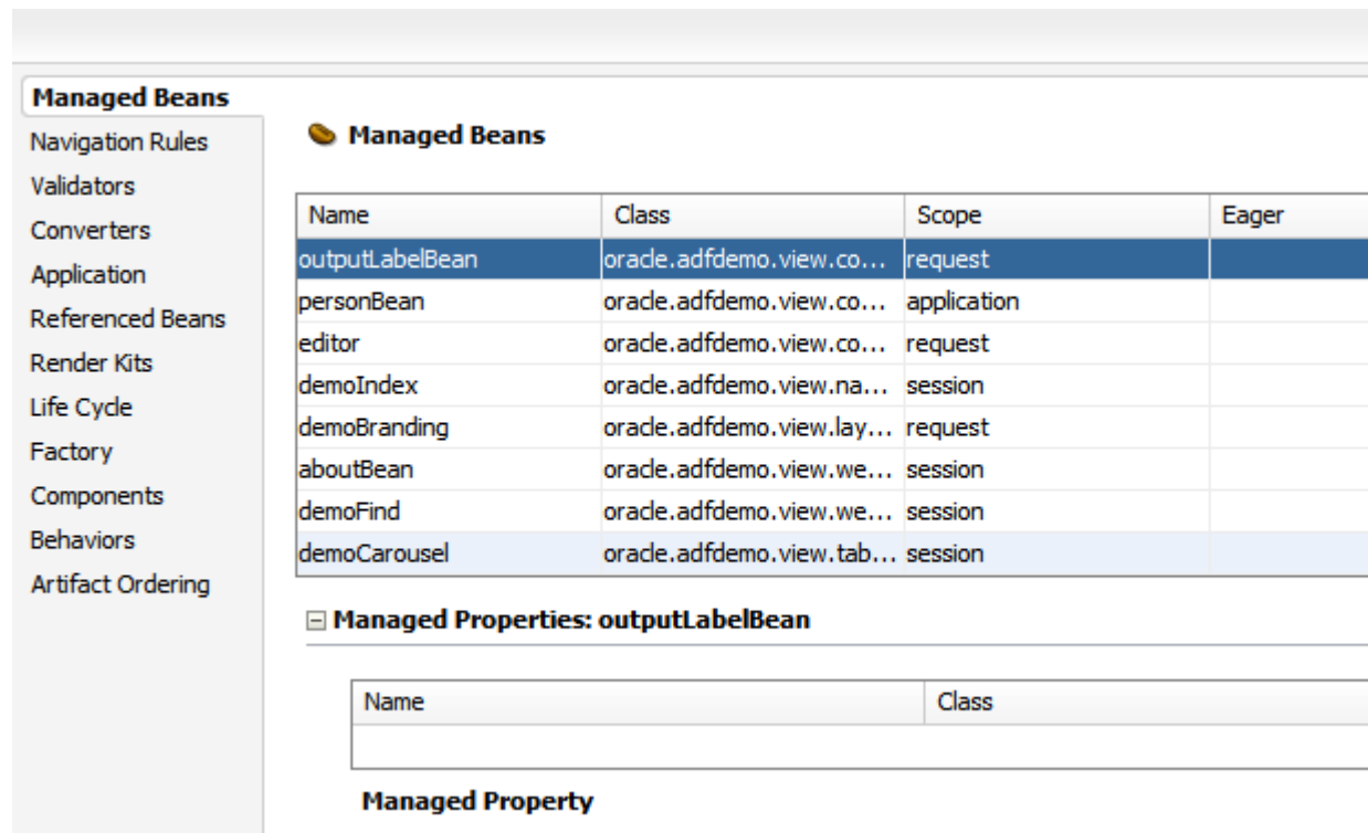
Figure 14-3 Managed Beans in the adfc-mobile-config.xml File
