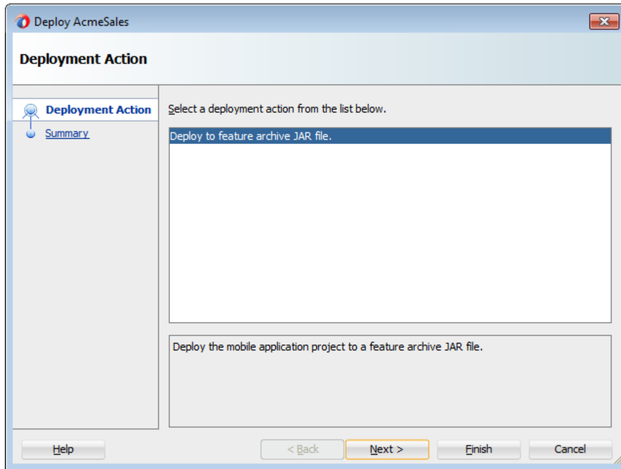
Figure 27-30 Deployment Actions
