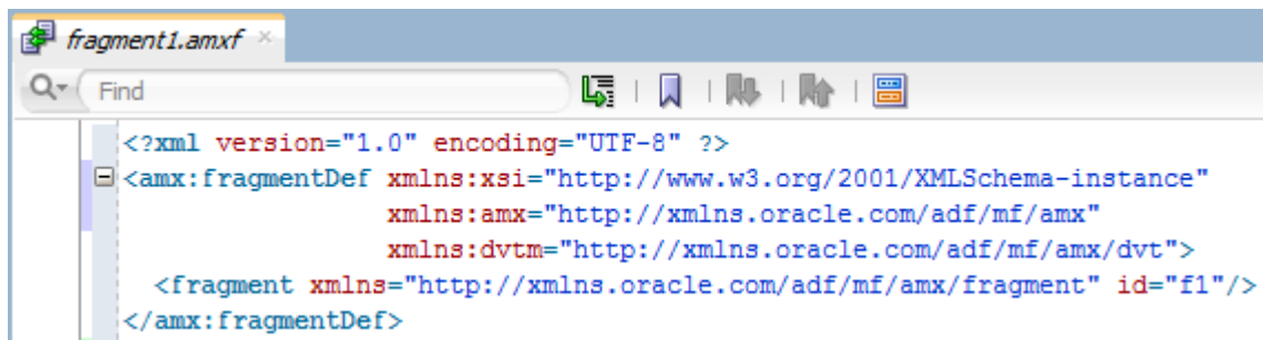
Figure 12-44 Fragment File
