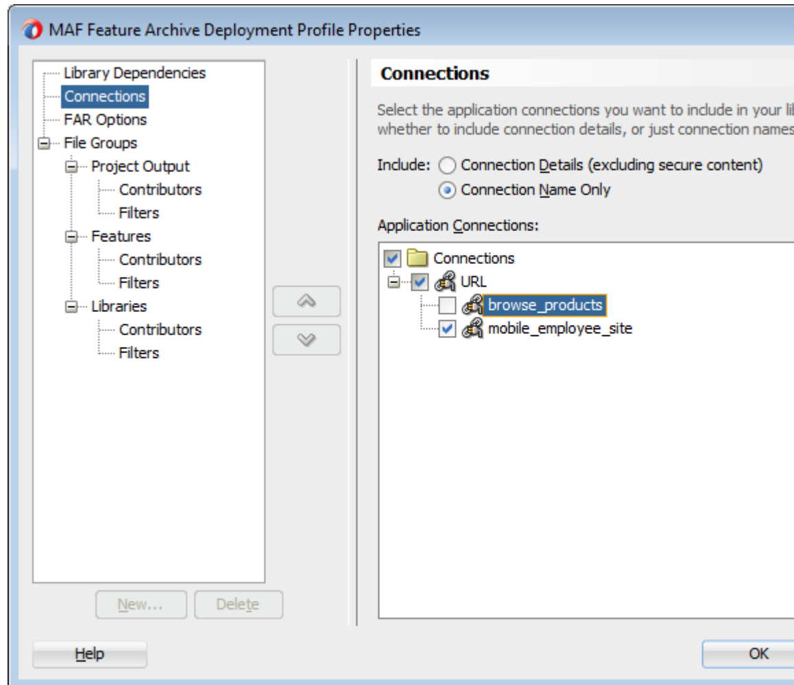
Figure 27-29 Selecting a Connection for the FAR
