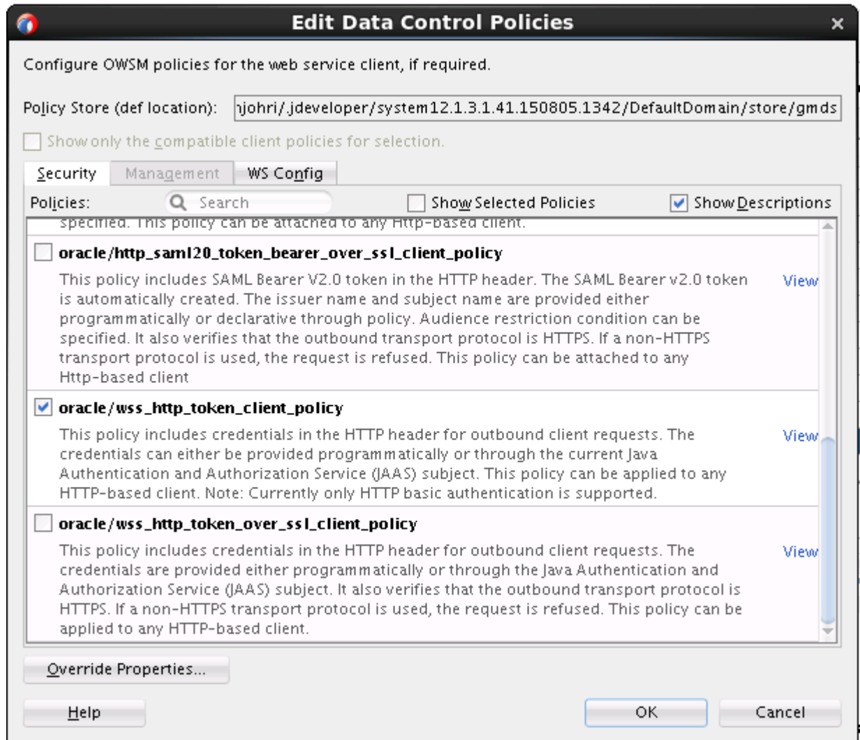
Figure 15-7 Editing Web Service Data Control Policies
