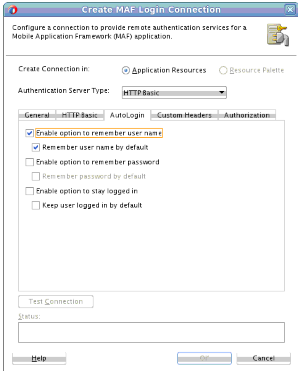
Figure 29-16 Caching User Credentials
