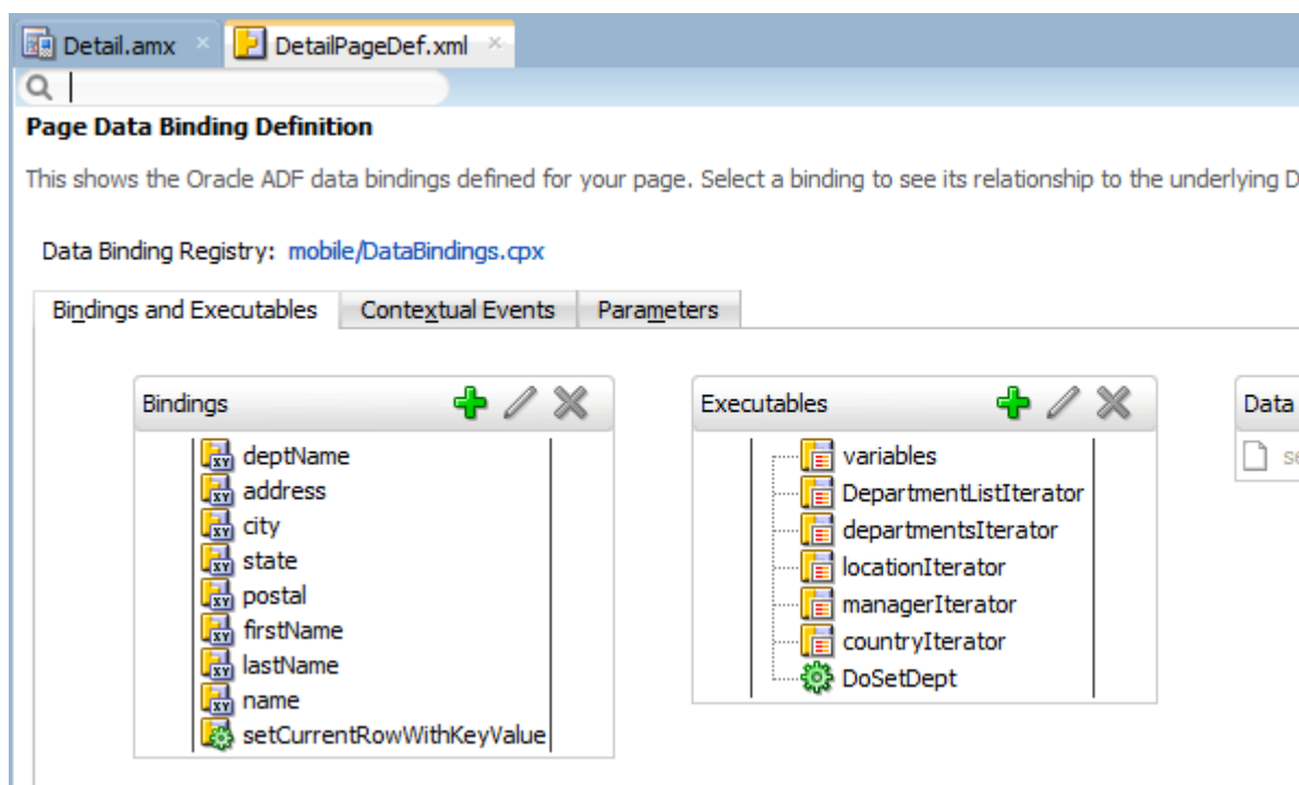
Figure 12-37 Page Definition File Accessed Through Go To Page Definition
