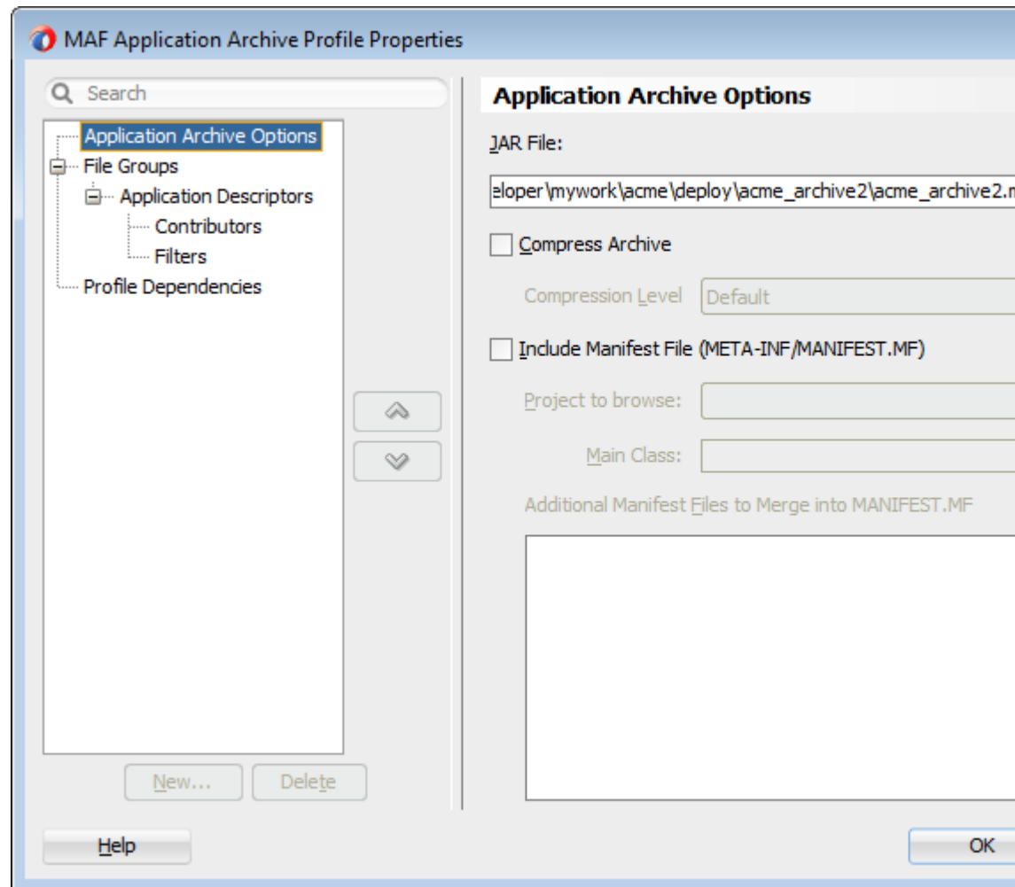
Figure 27-34 Entering a Name and Path for the Mobile Application Archive File
