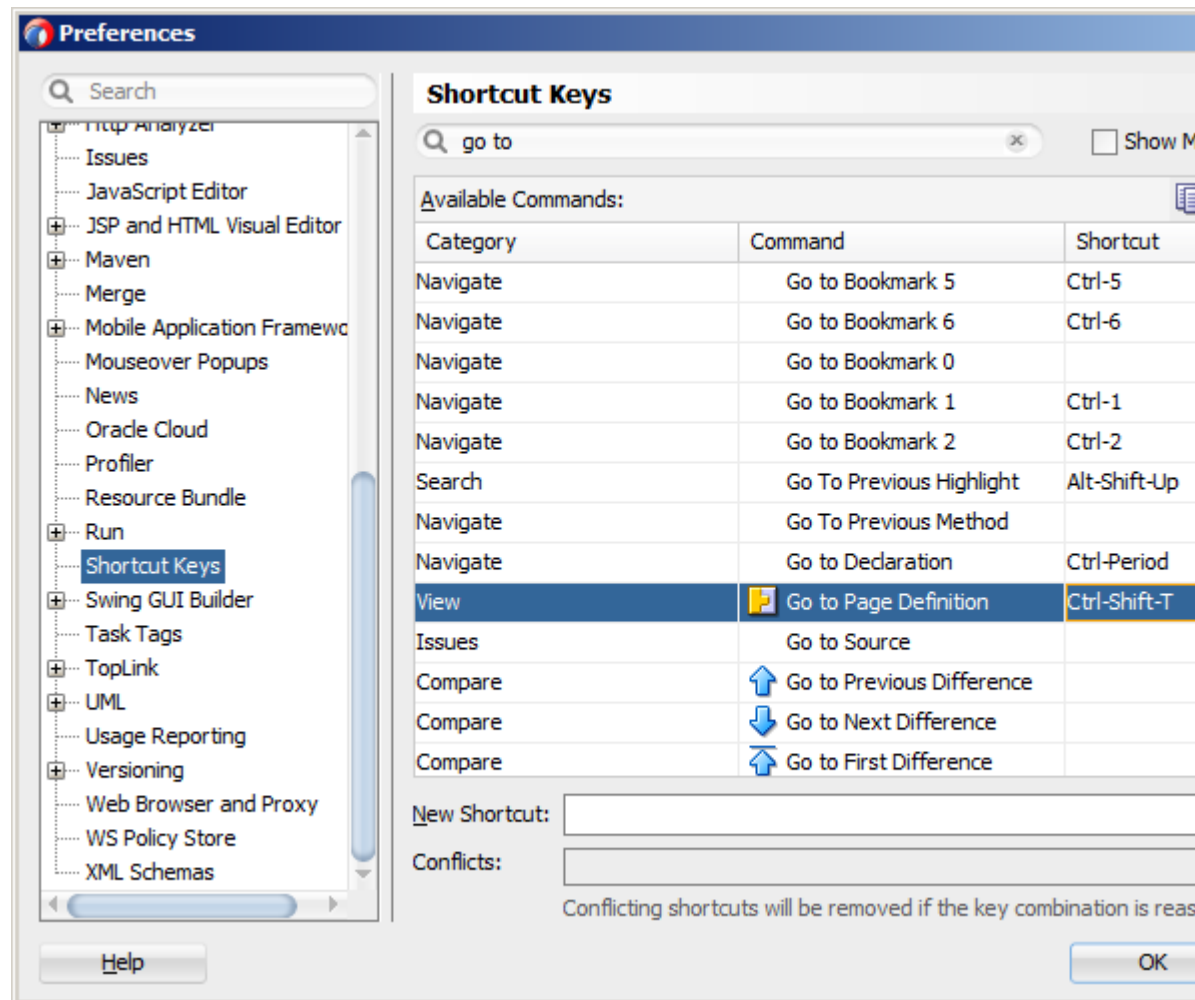
Figure 12-41 Opening Page Definition from Preferences
