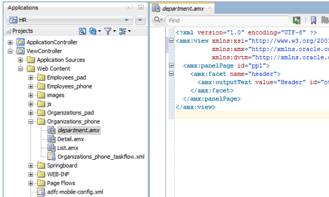
Figure 12-31 MAF AMX File in Applications Window
