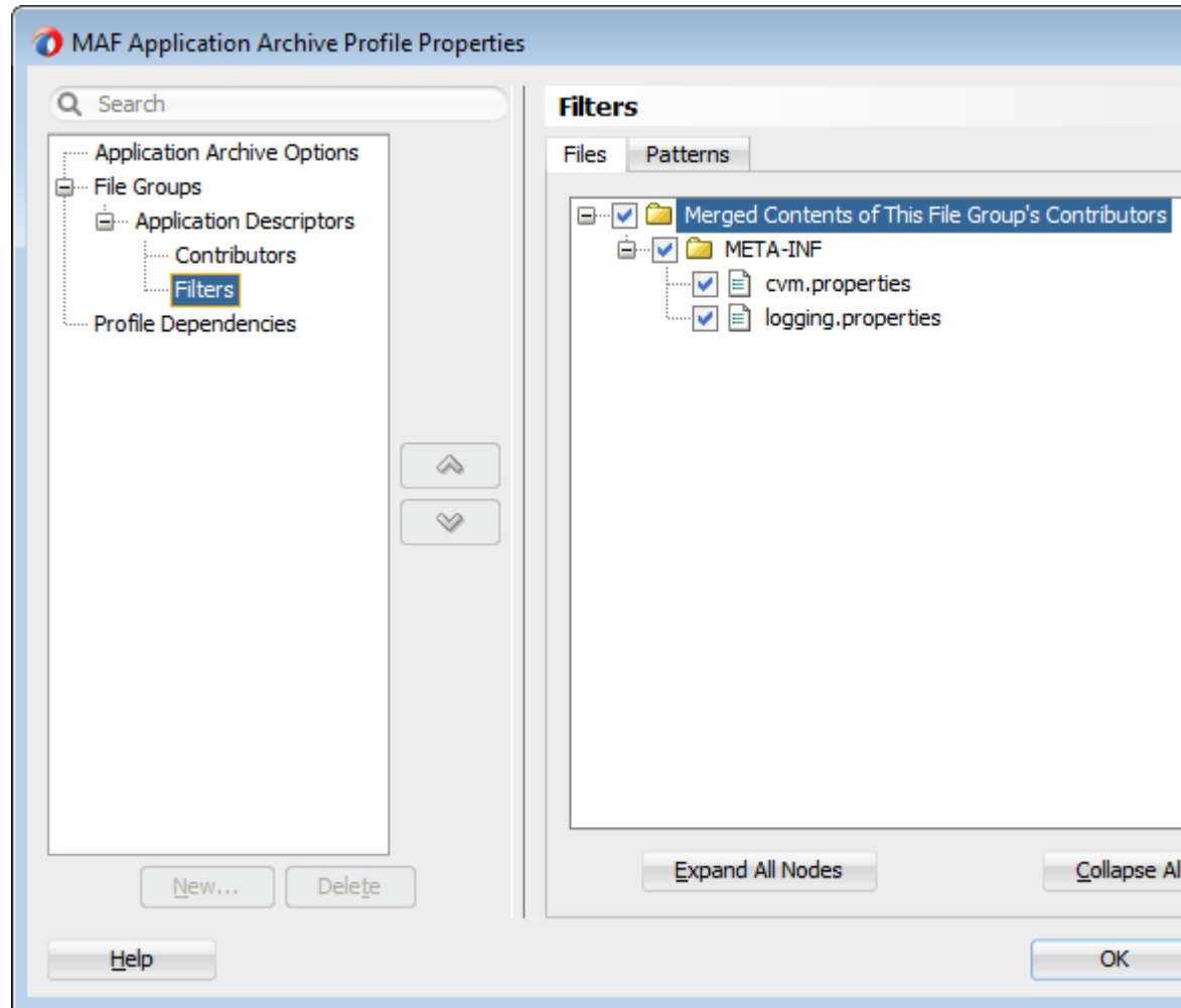
Figure 27-37 Including (or Excluding) Files and Directories
