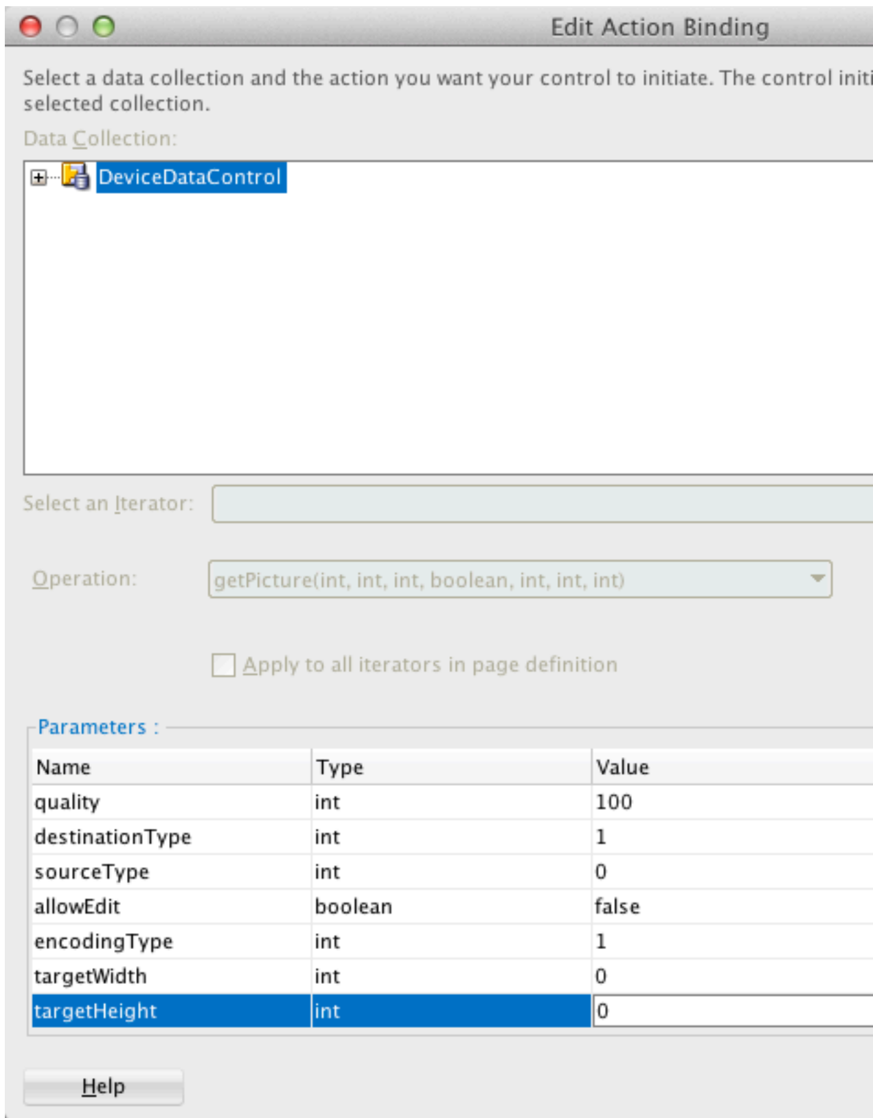
Figure 14-13 Bindings for Displaying an Image from the Photo Library at Design Time
