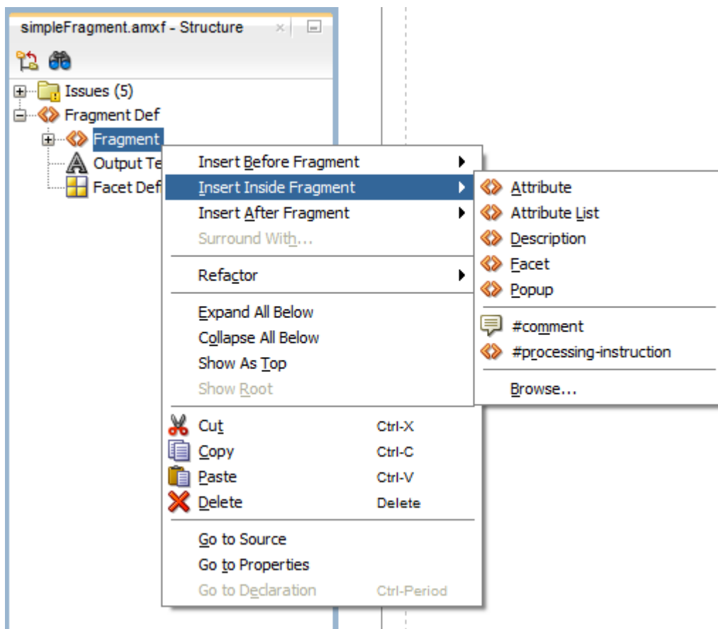
Figure 12-45 Populating Fragment
