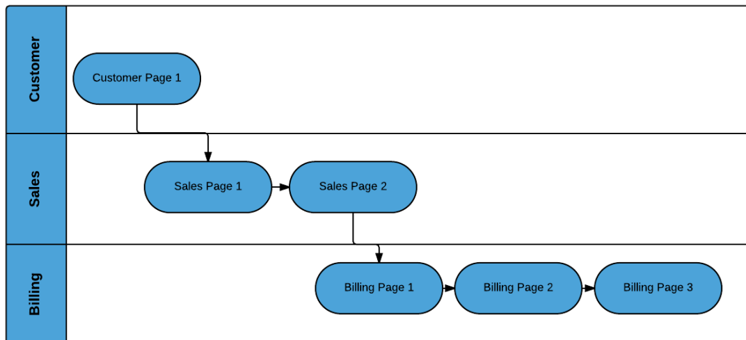
Figure 3-6 Navigation Flow Between Application Features and Pages in a MAF Application
