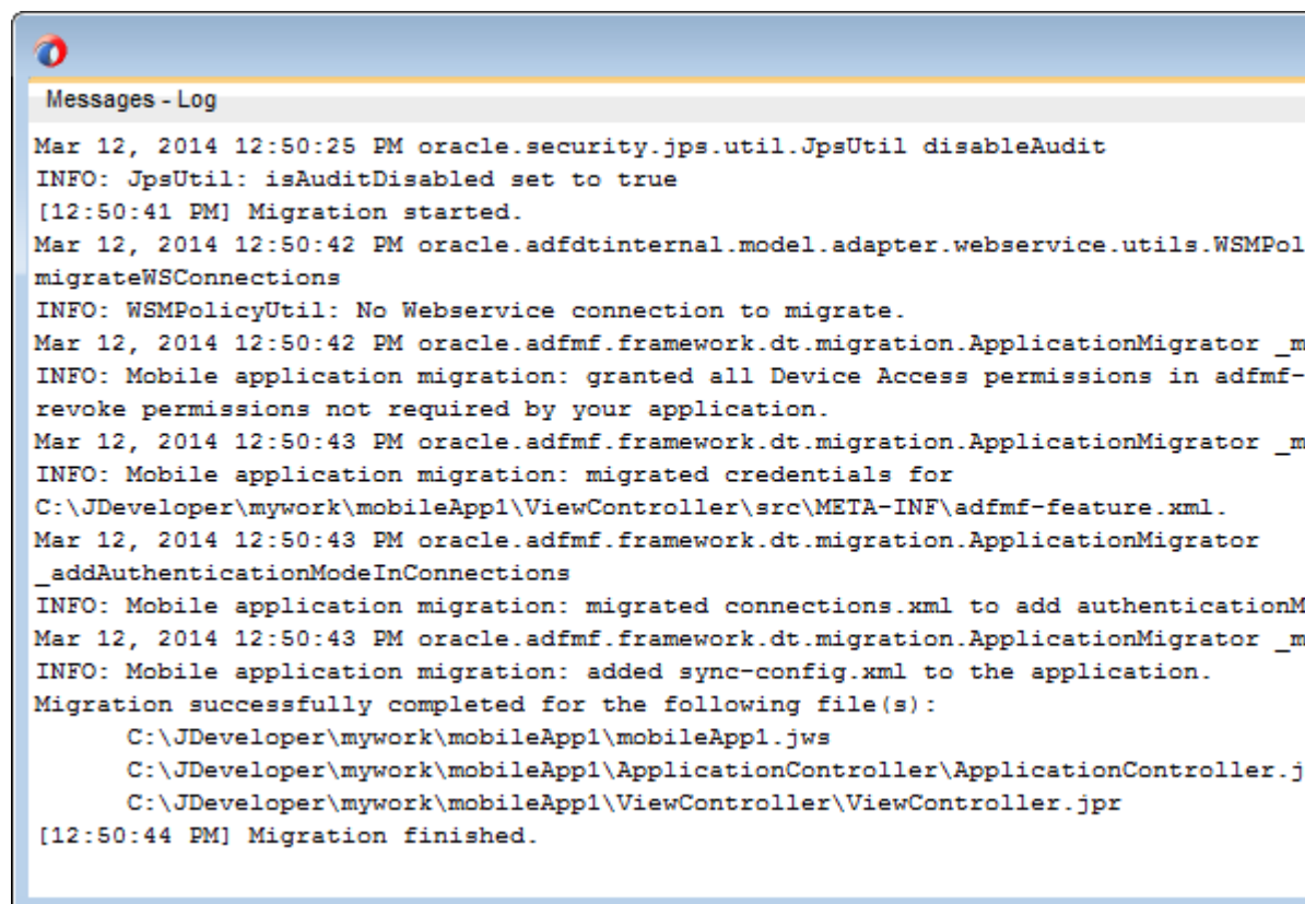
Figure 3-3 Migration Log
