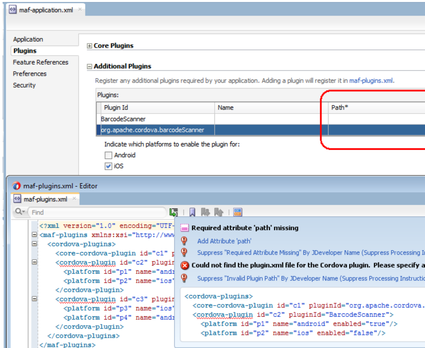
Figure 3-1 MAF Application that Does Not Specify Path to Plugin
