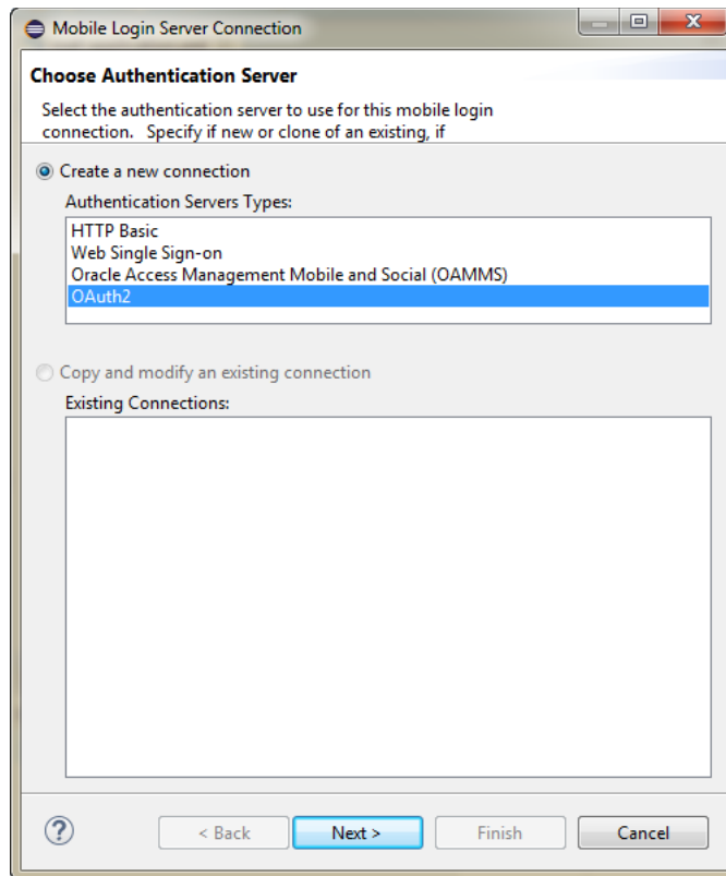
Figure 30–9 Configuring OAuth
