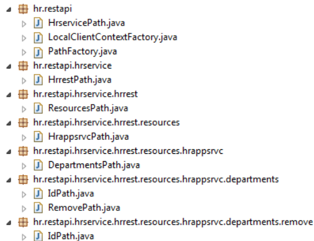
Figure 16–22 Generated REST API Artifacts
