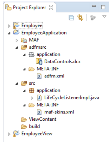
Figure 2–6 Application Project
