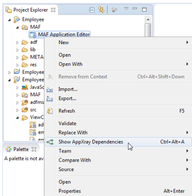
Figure 24–1 Opening AppXaminer
