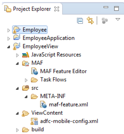
Figure 2–7 View Project
