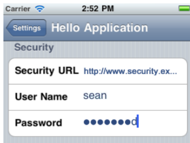
Figure 22-16 Text Preferences
