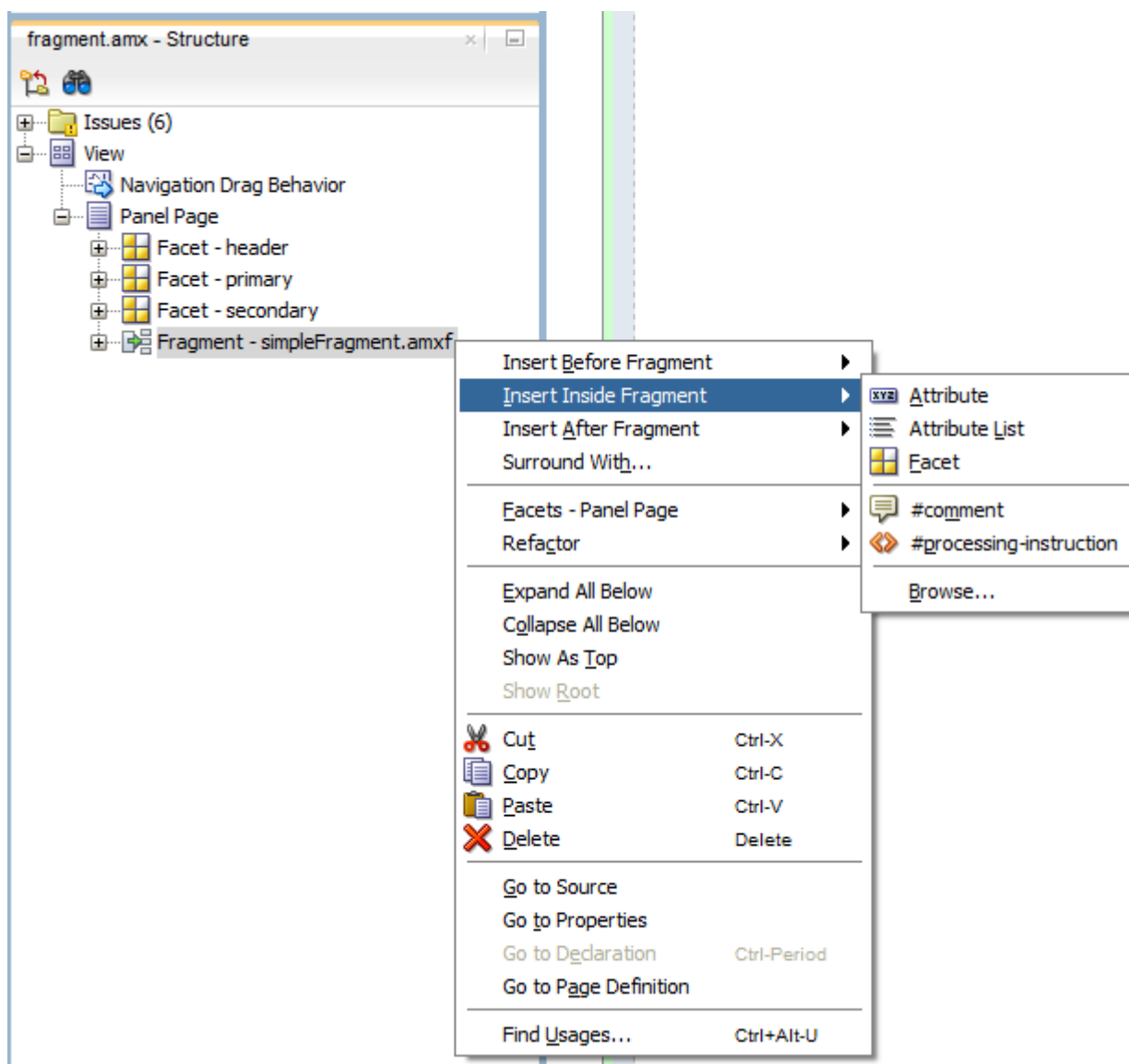
Figure 14-13 Populating Fragment
