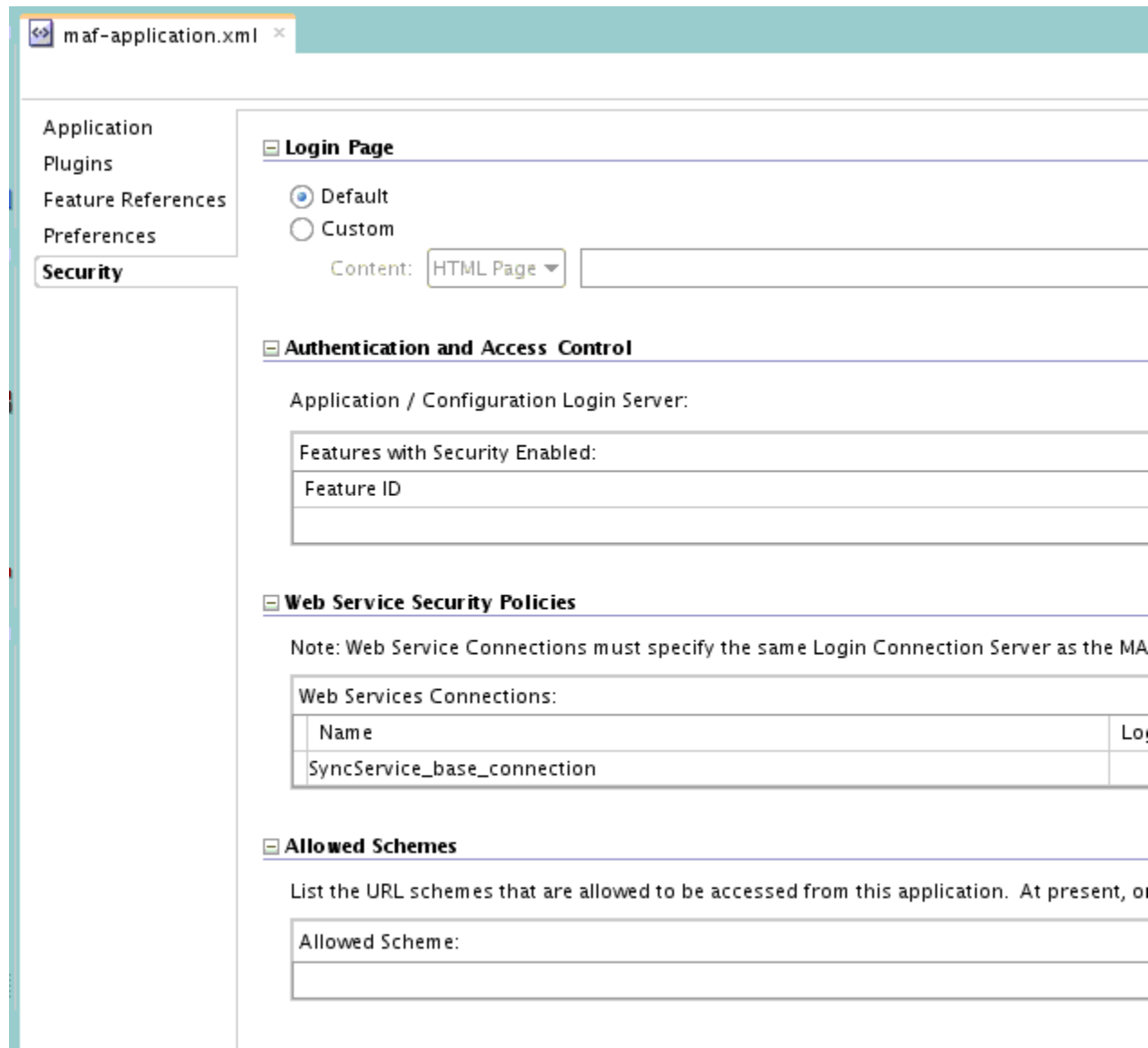
Figure 27-17 The Security Page of the maf-application.xml Overview Editor
