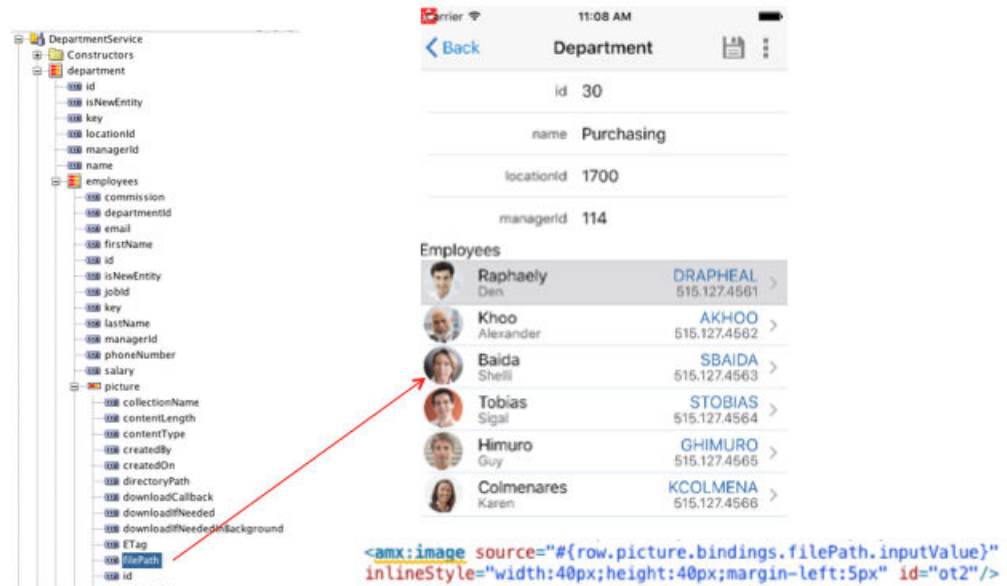
Figure 7-5 Adding an Image to a ListView
