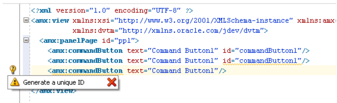
Figure 13-57 Element Identifier Audit in Source Editor
