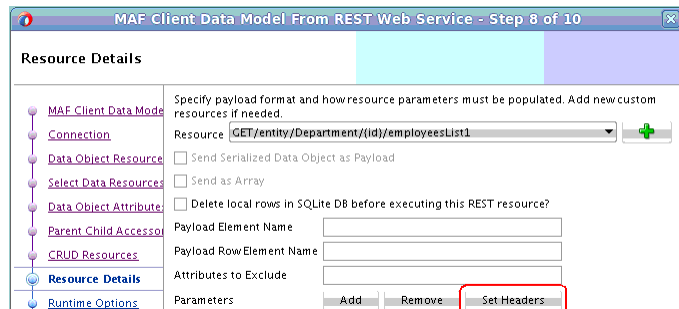
Figure 6-15 Setting HTTP Header Parameters
