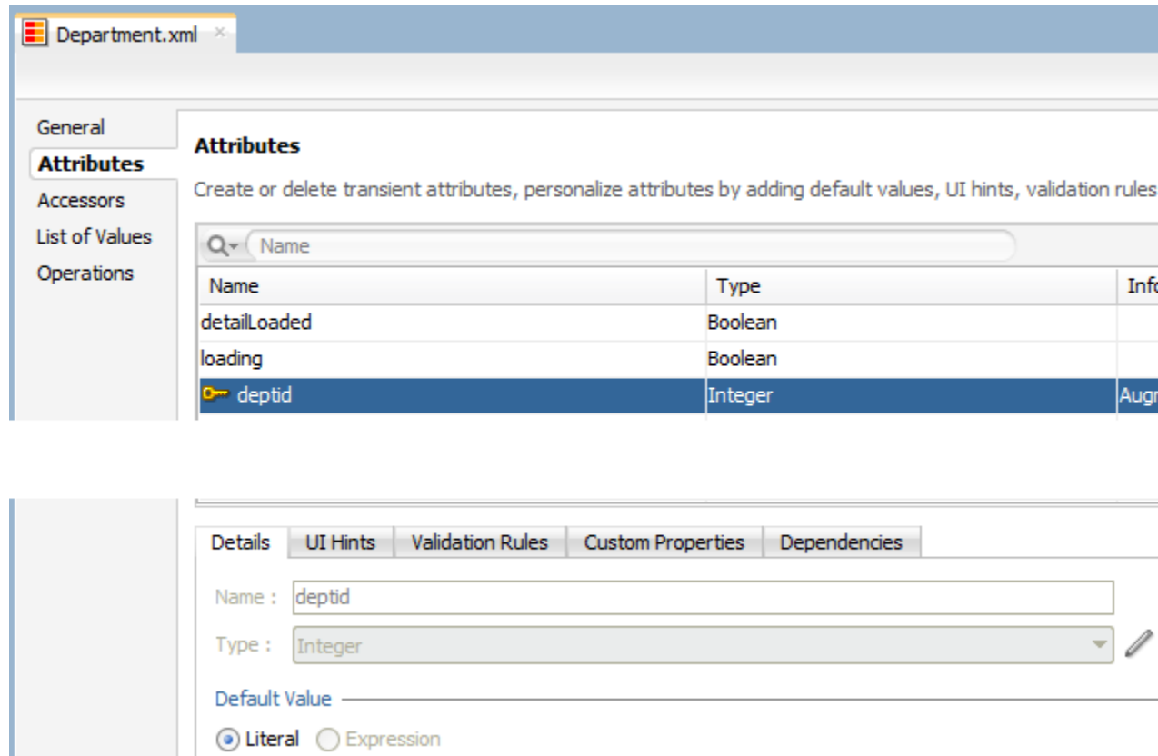
Figure 15-21 Selecting a Key Attribute in the Data Control Structure File of a Data Control
