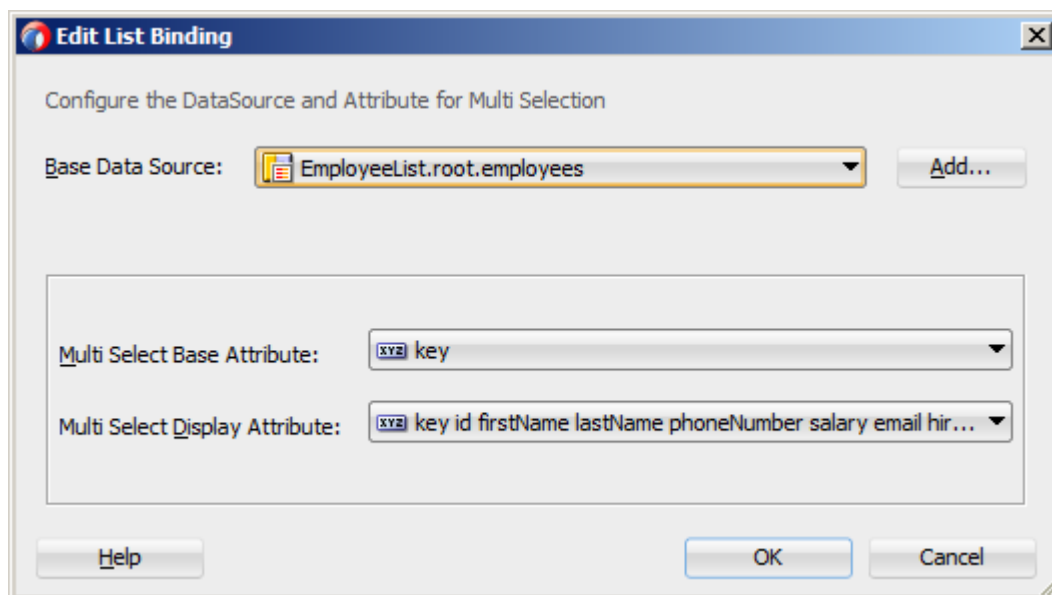
Figure 13-71 Edit List Binding Dialog for Multiple Selection Controls
