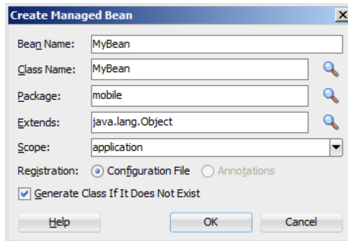
Figure 13-19 Setting Managed Bean Name and Class
