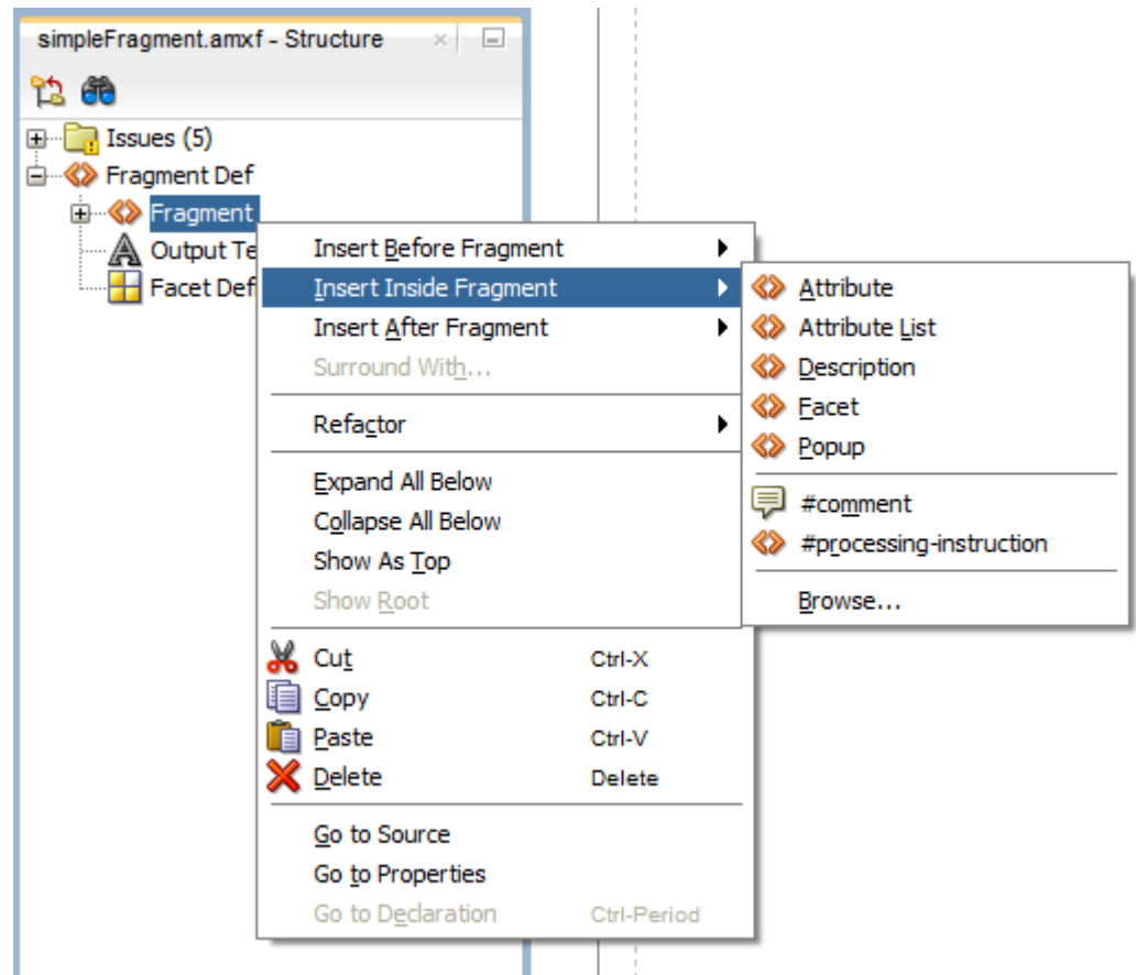
Figure 13-45 Populating Fragment
