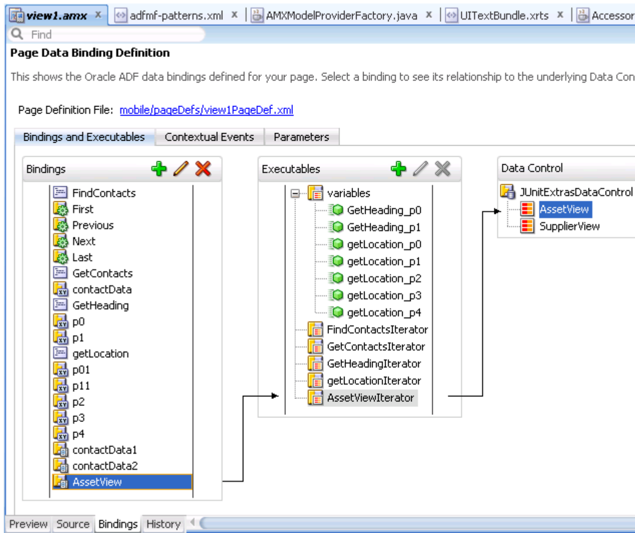
Figure 13-87 Bindings Tab
