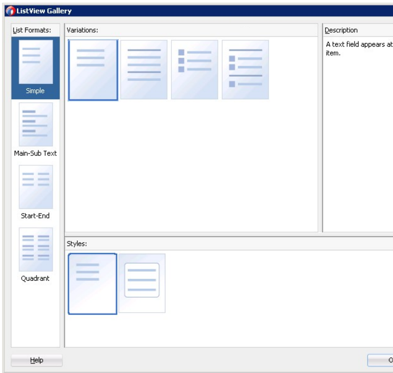
Figure 13-78 ListView Gallery
