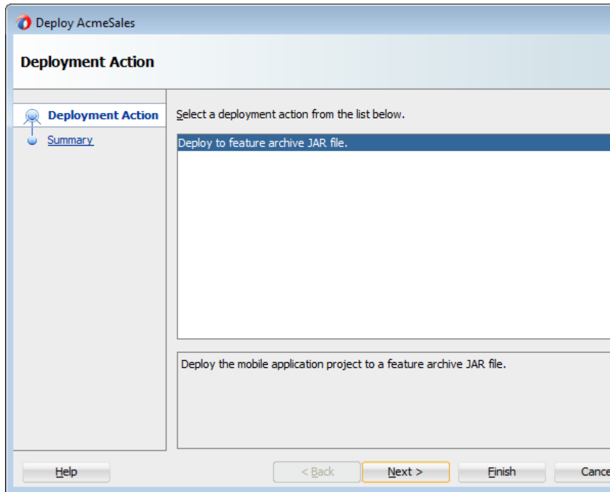
Figure 25-26 Deployment Actions
