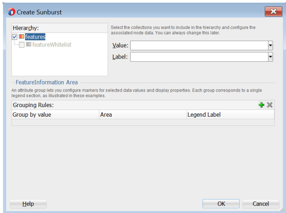
Figure 14-75 Creating Sunburst
