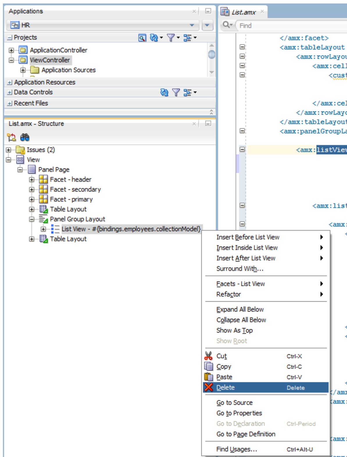
Figure 13-88 Deleting Bound Components from Page
